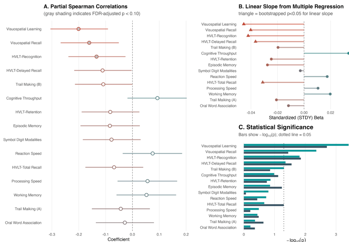
Fig. 4. Exploratory Associations Between Psychiatric Symptom Burden and Cognitive Tests
