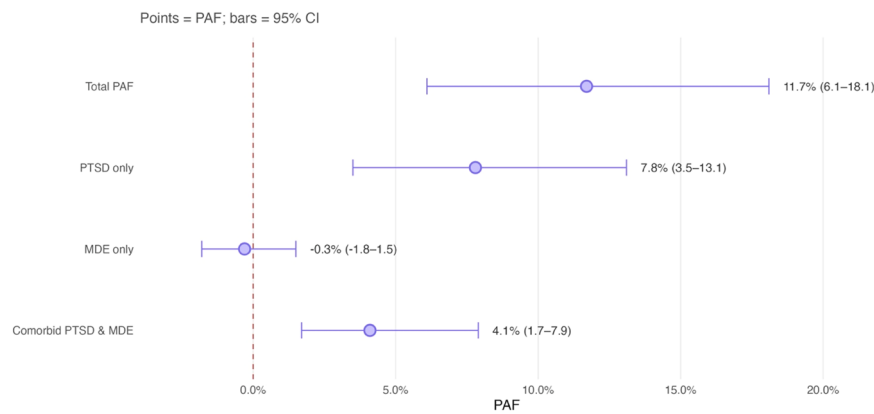
Fig. 3. Population-Attributable Fractions (PAF) for Mild Cognitive Impairment by Psychiatric Diagnoses
