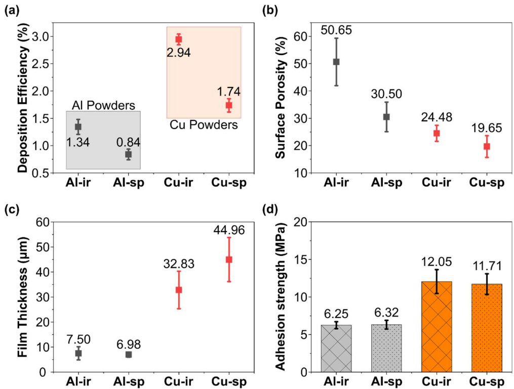
Fig. 2. (a) Deposition efficiency; (b) surface porosity; (c) film thickness; (d) adhesion strength of the resulting depositions. (Refer to Table 3 for the average magnitudes and their corresponding standard deviations).
