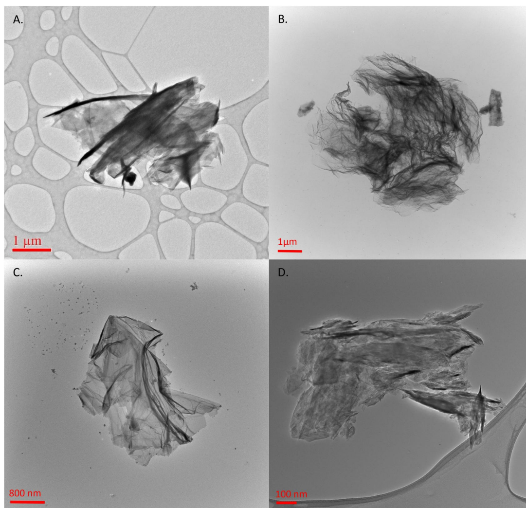
Figure 2. Transmission electron microscopy images of GFNs collected from personal breathing zone samples of workers from (A) GNP from Facility 2; (B) GO from Facility 5; (C) GO from Facility 7; (D) FLG from Facility 9.
