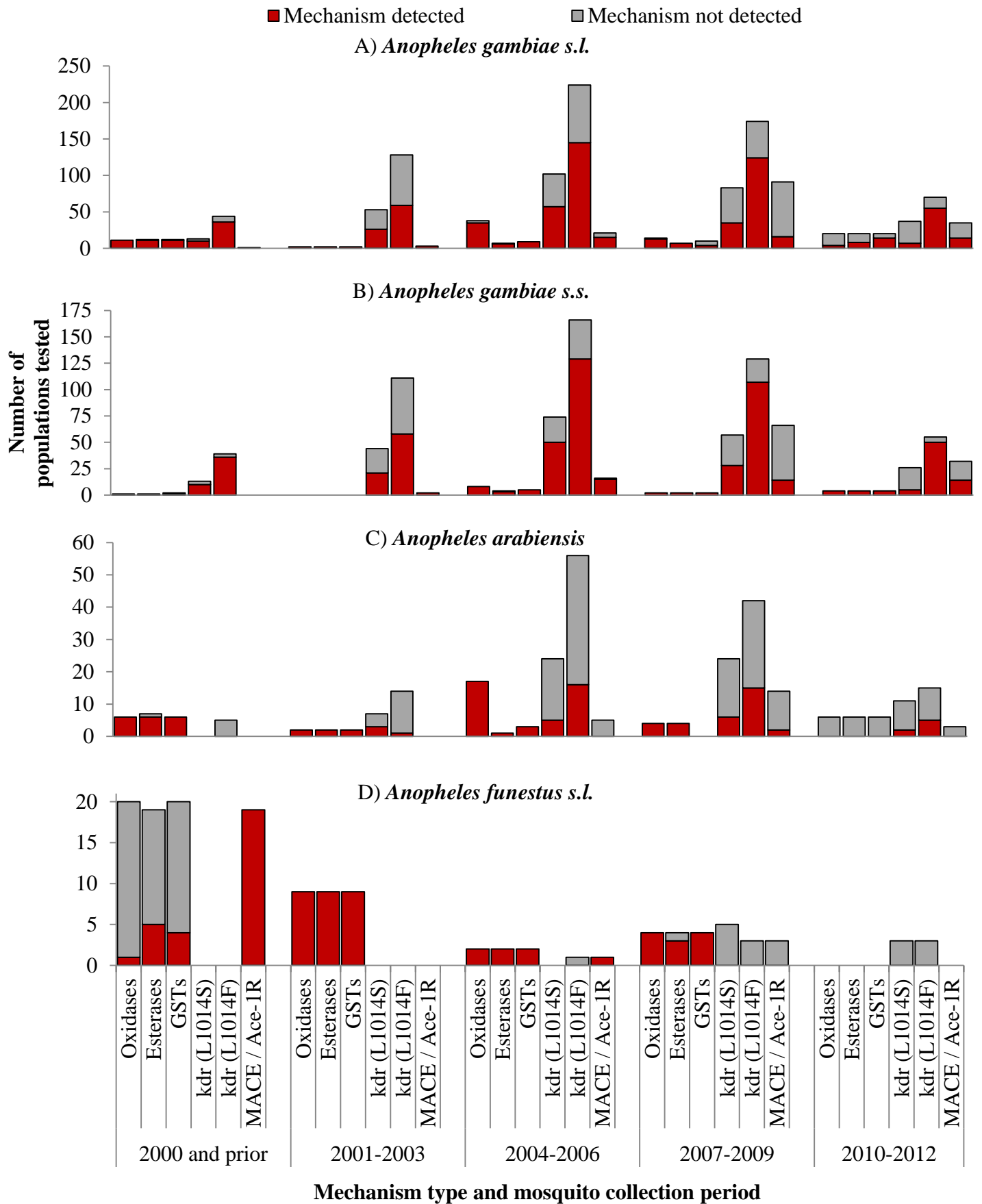
Number of populations for which resistance mechanisms were detected (red) and not detected (grey). A) An. gambiae s.l. , B) An. gambiae s.s. , C) An. arabiensis and D) An. funestus s.l. by year of mosquito collection and mechanism class.
