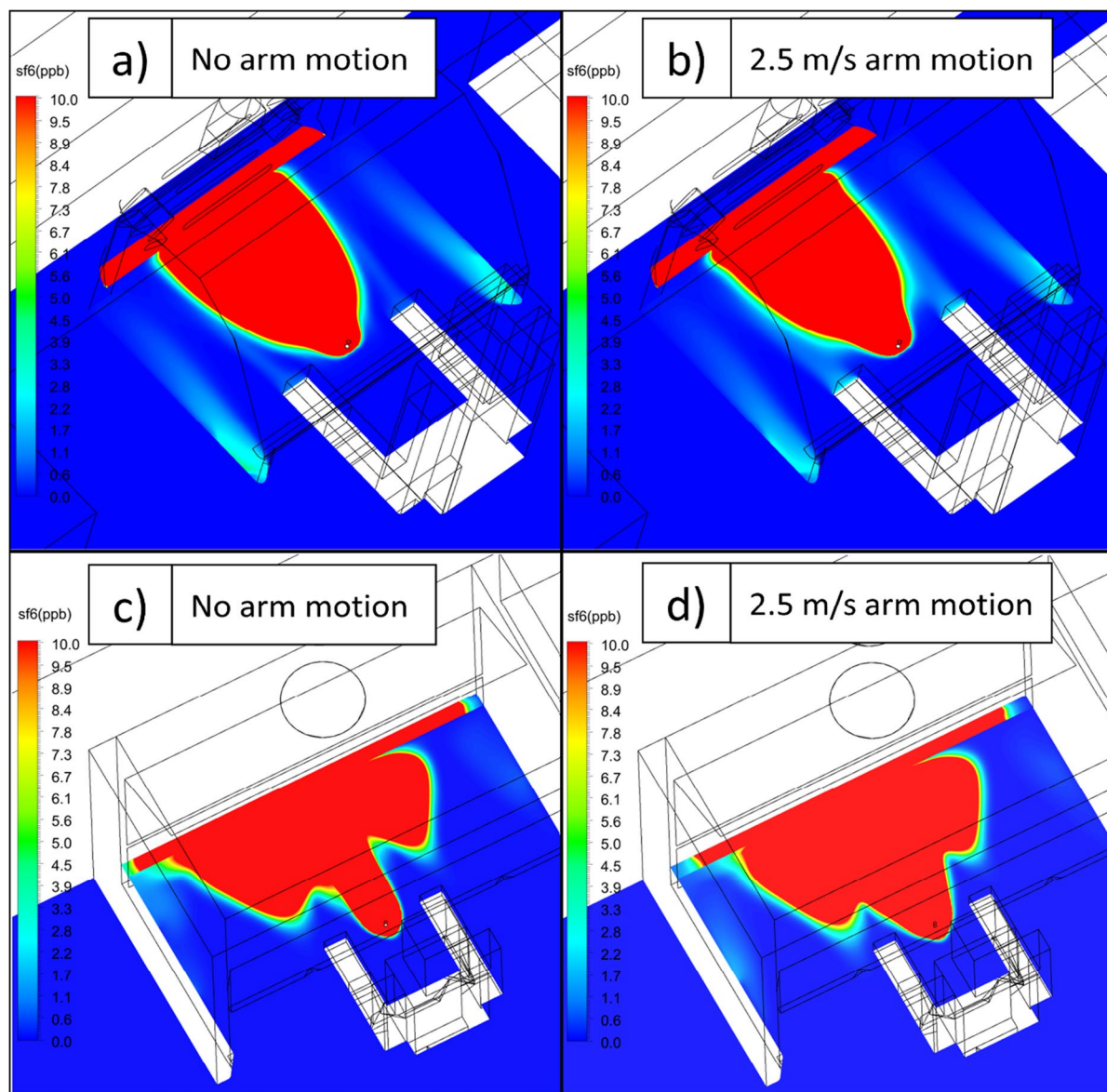
Fig. 5 \text{SF}_6 predicted concentration contours for the CAV hood with no arm motion and 2.5 m/s arm motion at a horizontal cut plane through both arms for a) nano hood with no arm motion,
