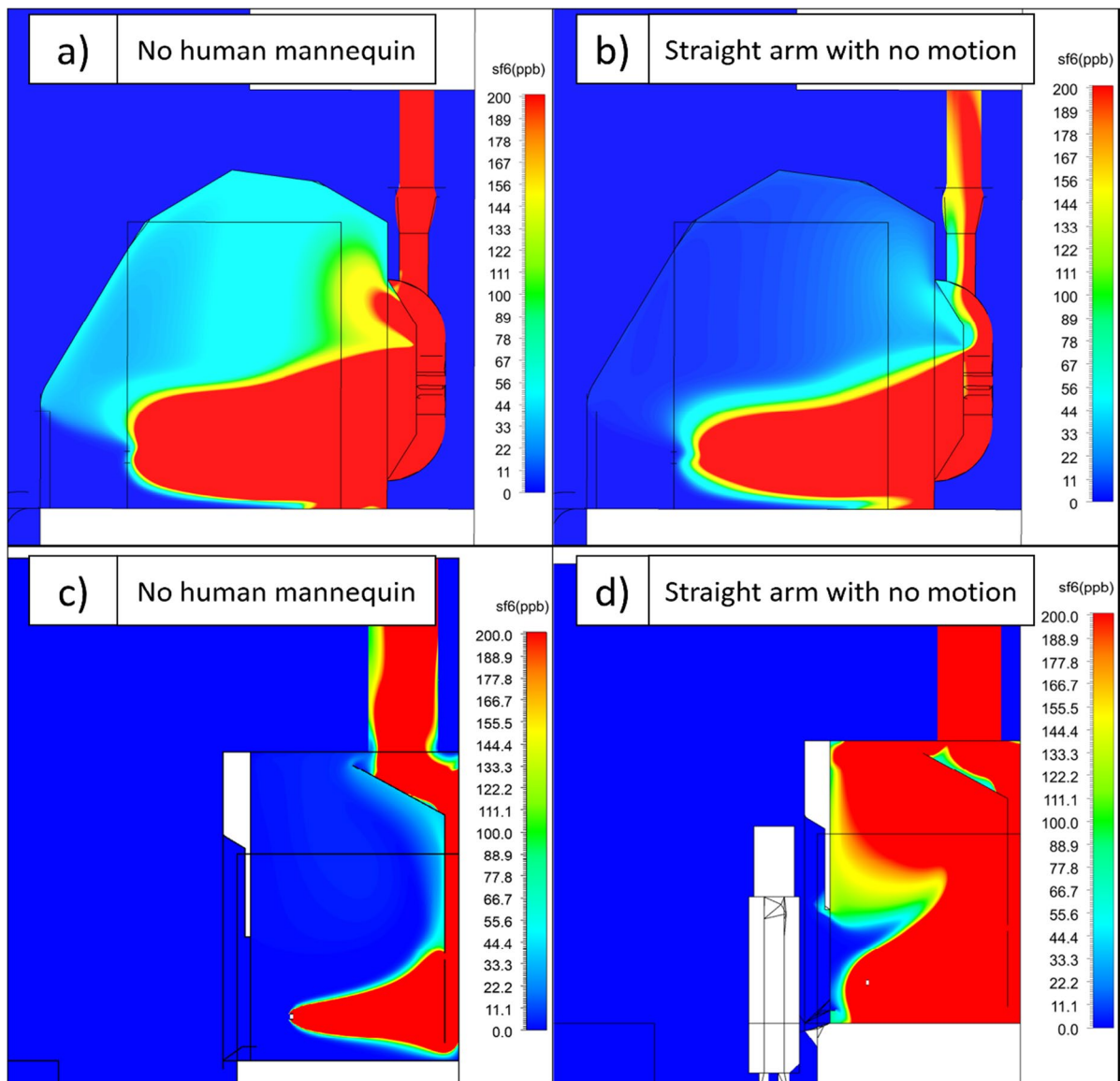
Fig. 4 \text{SF}_6 predicted concentration contours at a vertical cut plane with no human mannequin and with a straight-arm mannequin for a) nano hood without mannequin, b) nano hood
