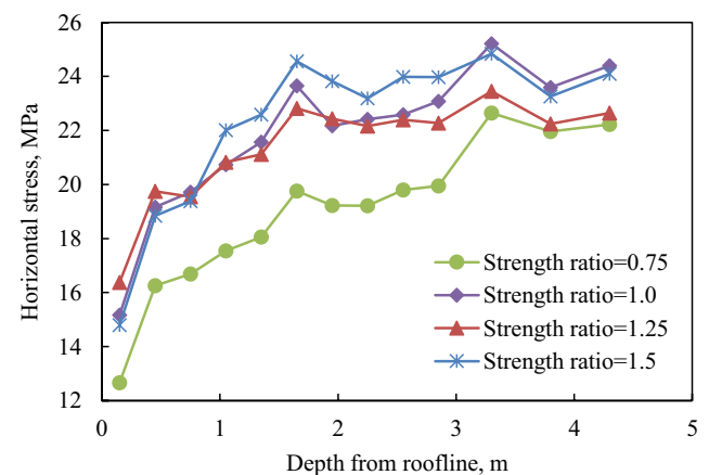
Fig. 12 Effect of discontinuity strength ratio on stress distribution
