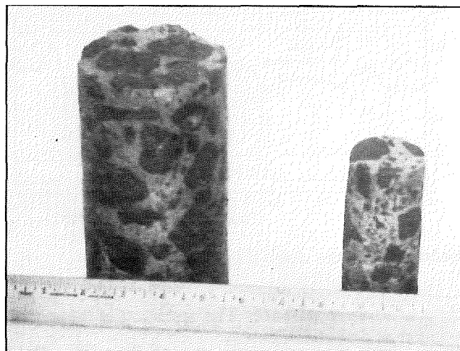
Core samples from full-scale model.
