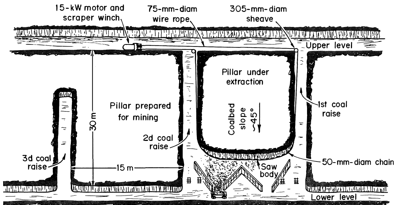
Korean mining system.
