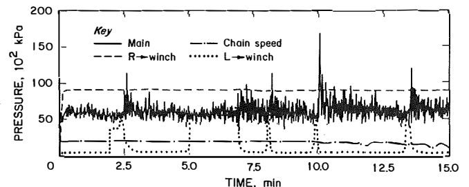
Raw data from down-ridge mining test.
