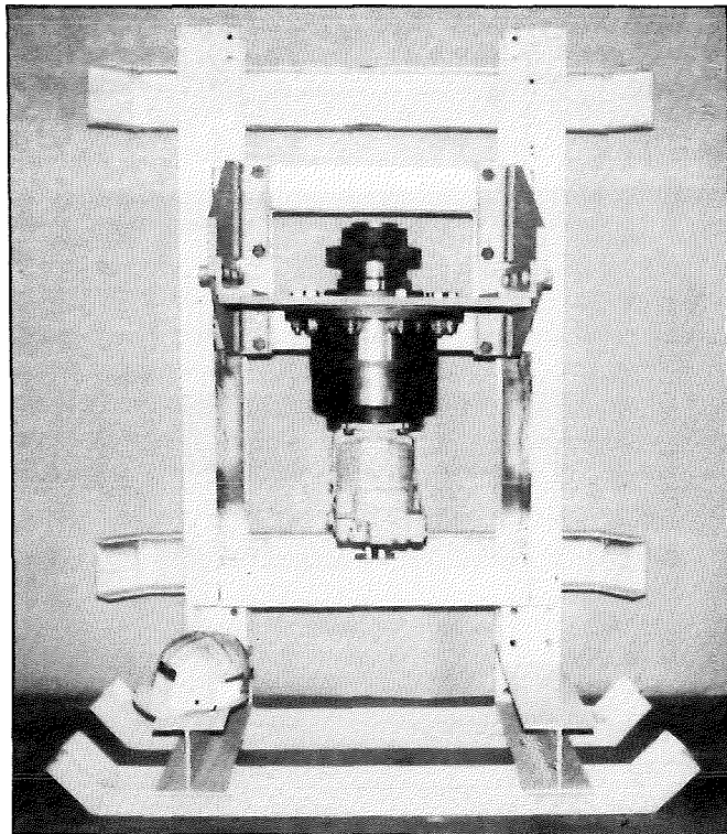
Drive side mobile structure.
