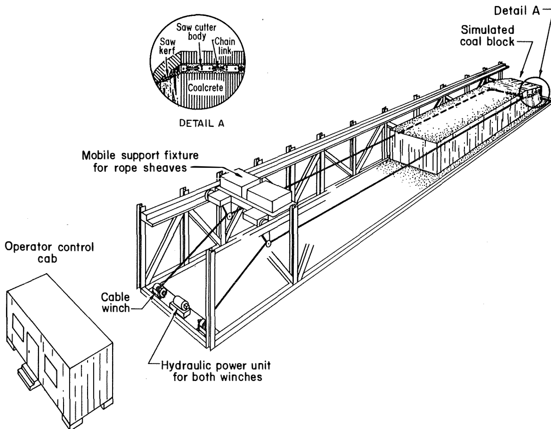
Quasi-full-scale model for cross-ridge mining.
