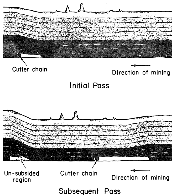
Initial and subsequent passes of RFT mining.
