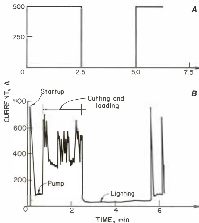
Figure 2.—Step function (A) and continuous miner current traces (B).
