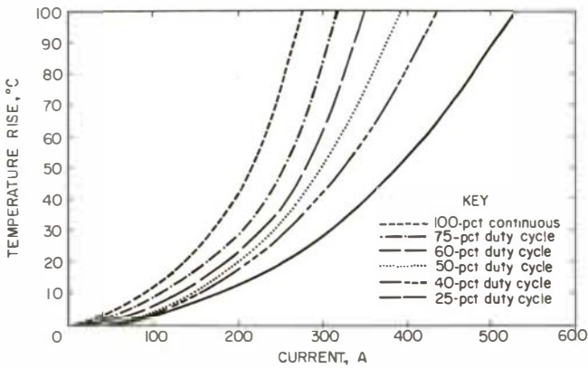
Figure 12.—Average rise above ambient of conductor-insulation interface in No. 2 AWG, 2/c, flat G cable.
