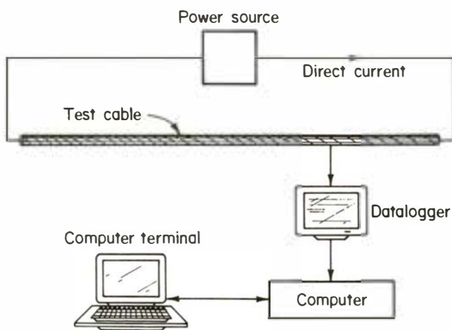
Figure 3.—Load test setup.
