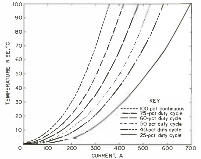
Figure 13.—Average rise above ambient of conductor-insulation interface in No. 1/0 AWG, 2/c, flat W cable.
