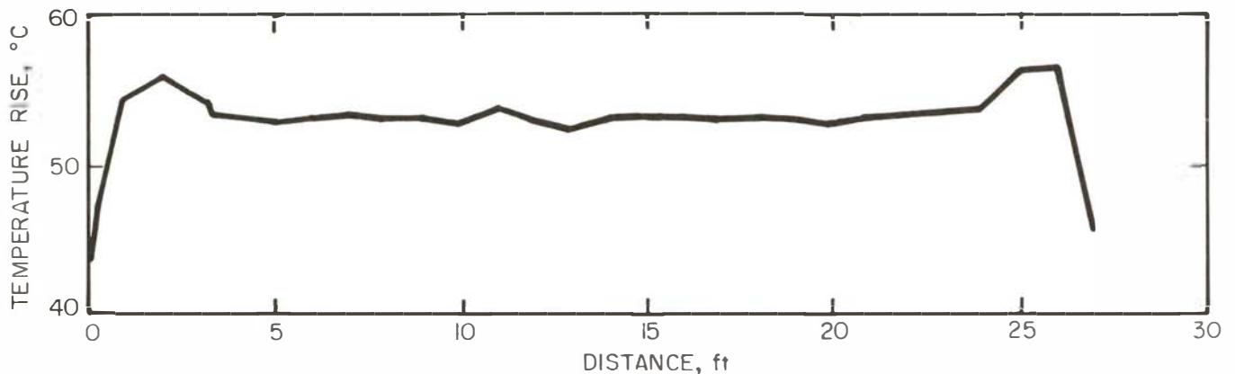
Figure 6.—End effects of cable in still air.
