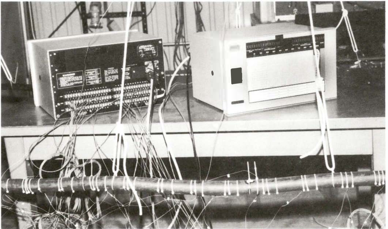
Figure 5.—Thermocouple connections to datalogger.
