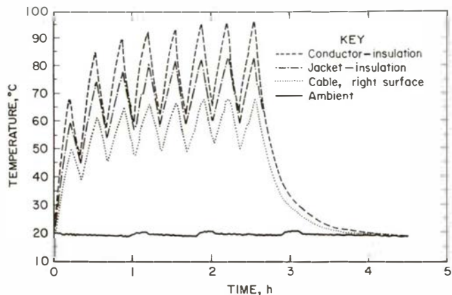
Figure 9.—Intermittent test of No. 2 AWG, 2/c, flat G cable loaded at 300 A for 60 pct of time.
