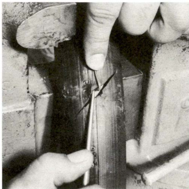
Figure 4.—Thermocouple placement within cable specimen.
