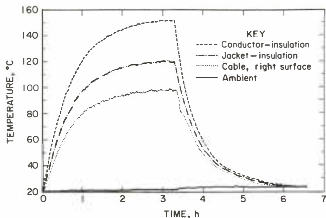
Figure 8.—Steady-state load test results for No. 2/0 AWG, 3/c, round G-GC cable loaded at 400 A.
