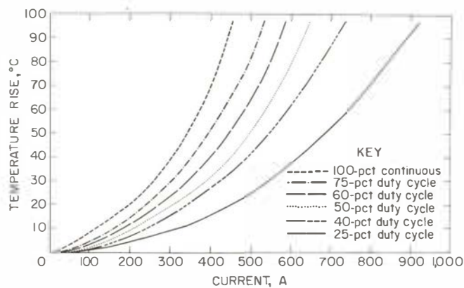
Figure 15.—Average rise above ambient of conductor-insulation interface in No. 4/0 AWG, 3/c, round G-GC cable.
