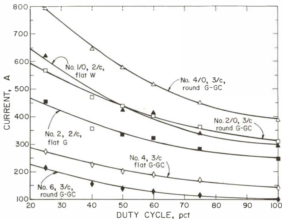
Figure 16.—Load required to effect a 70° C rise.
