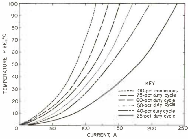
Figure 10.—Average rise above ambient of conductor-insulation interface in No. 6 AWG, 3/c, round G-GC cable.
