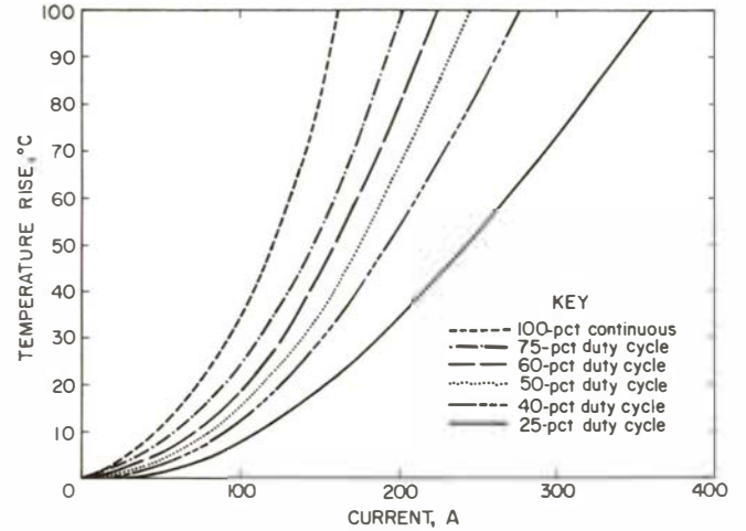
Figure 11.—Average rise above ambient of conductor-insulation interface in No. 4 AWG 3/c, flat G-GC cable.
