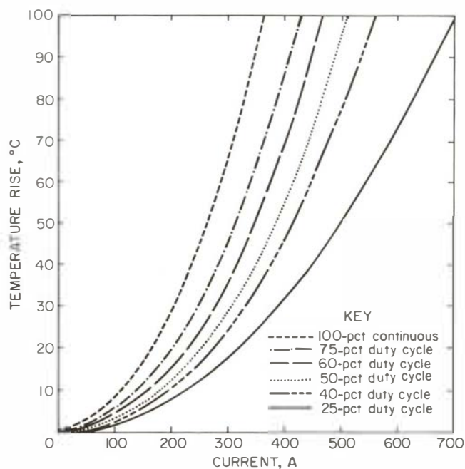
Figure 14.—Average rise above ambient of conductor-insulation interface in No. 2/0 AWG, 3/c, round G-GC cable.
