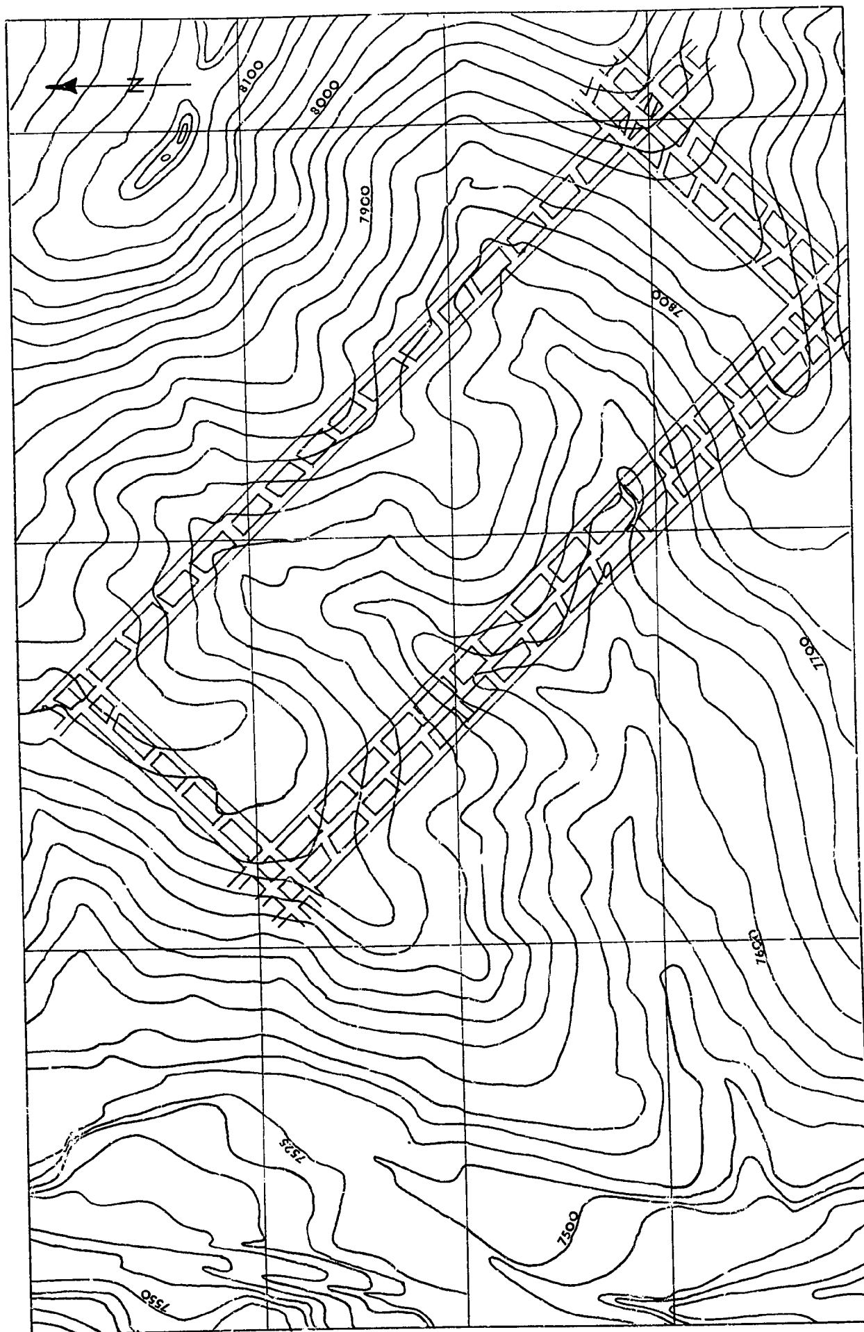
FIG 35 GENERAL TOPOGRAPHY 4N L.W. PANEL. York Canyon Mine.
