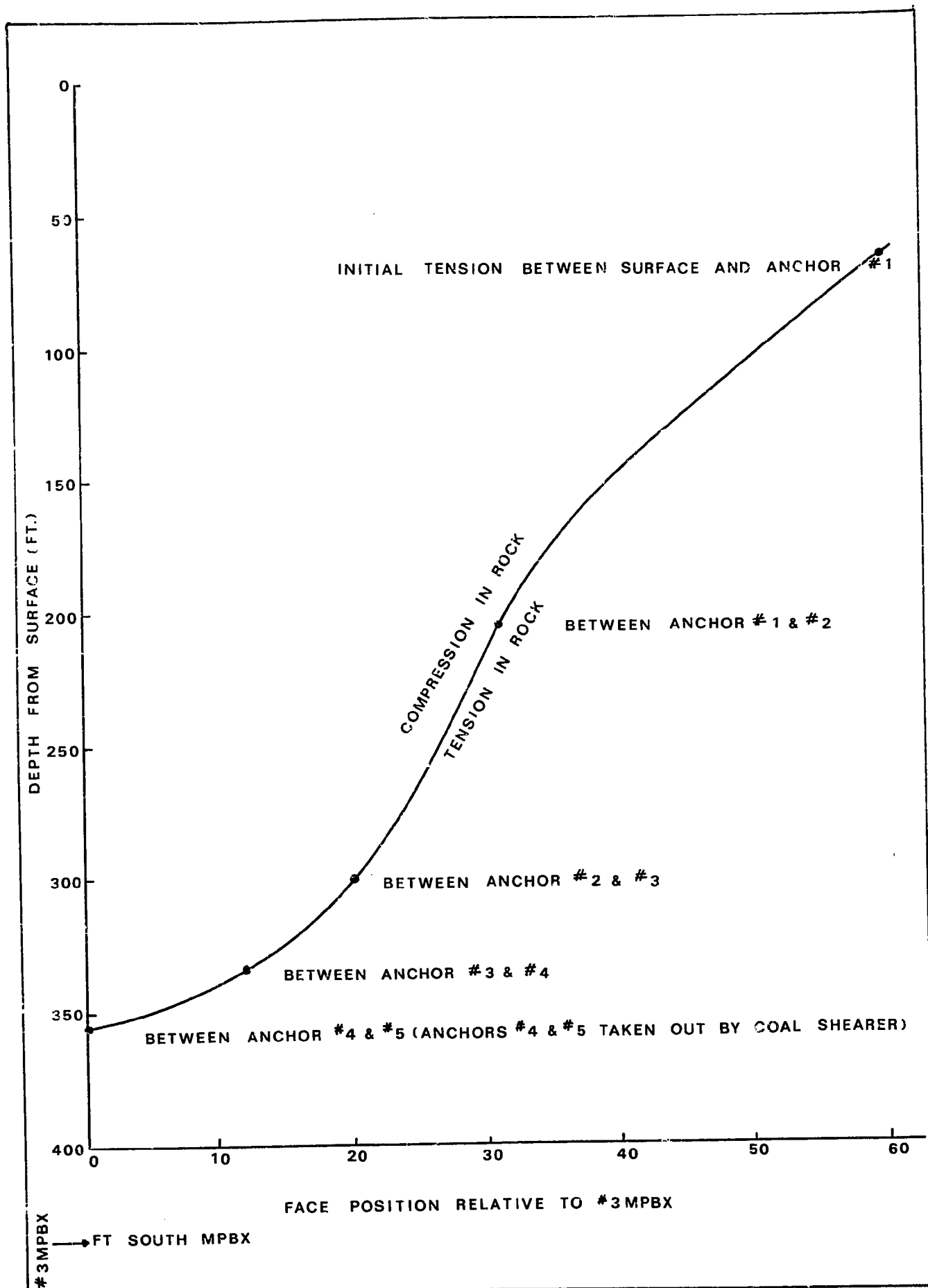
FIG 39 TENSION DEVELOPMENT FOR DEPTH vs FACE POSITION
