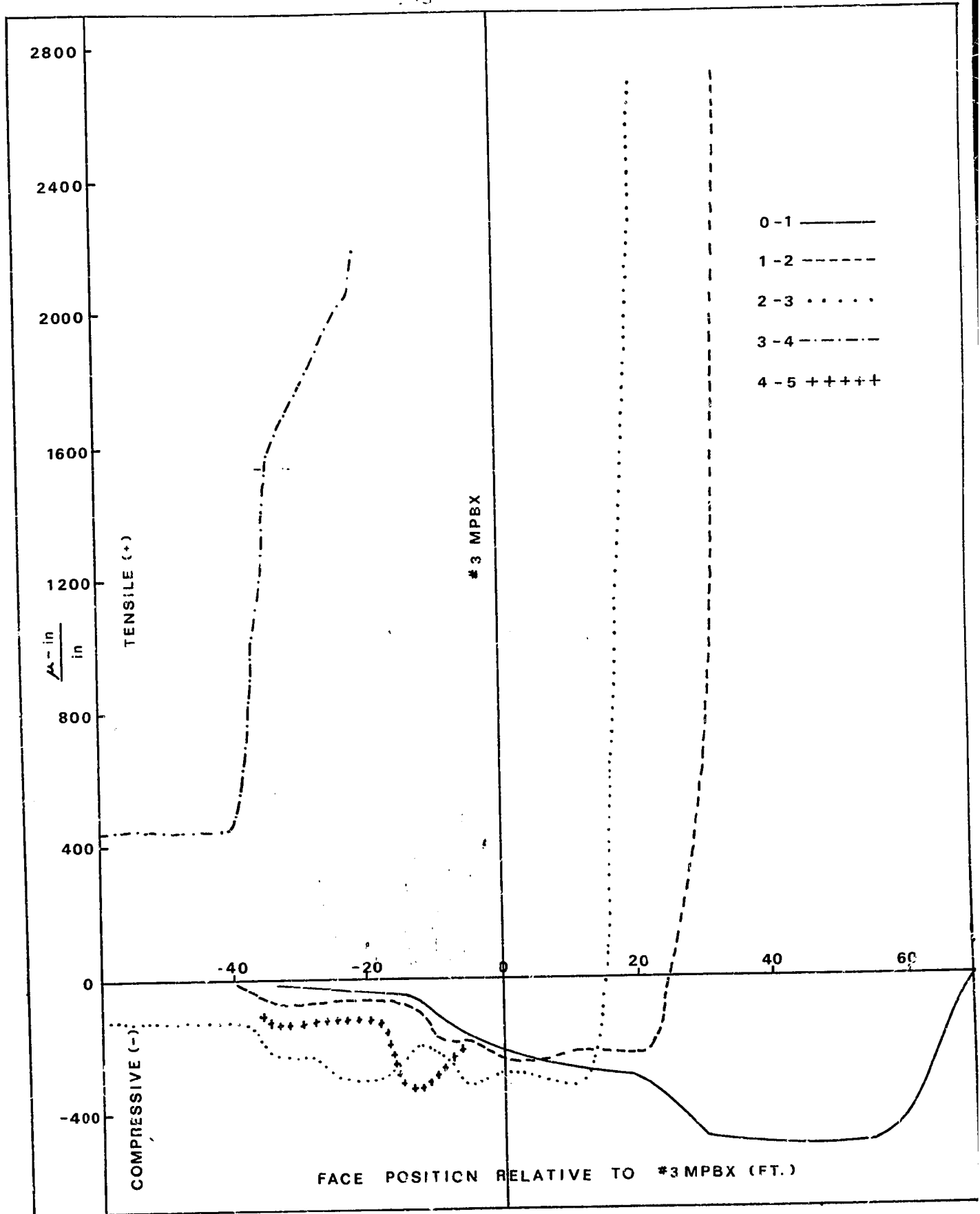
FIG 40 RELATIVE STRAIN BETWEEN ANCHORS York Canyon Mine Test Panel
