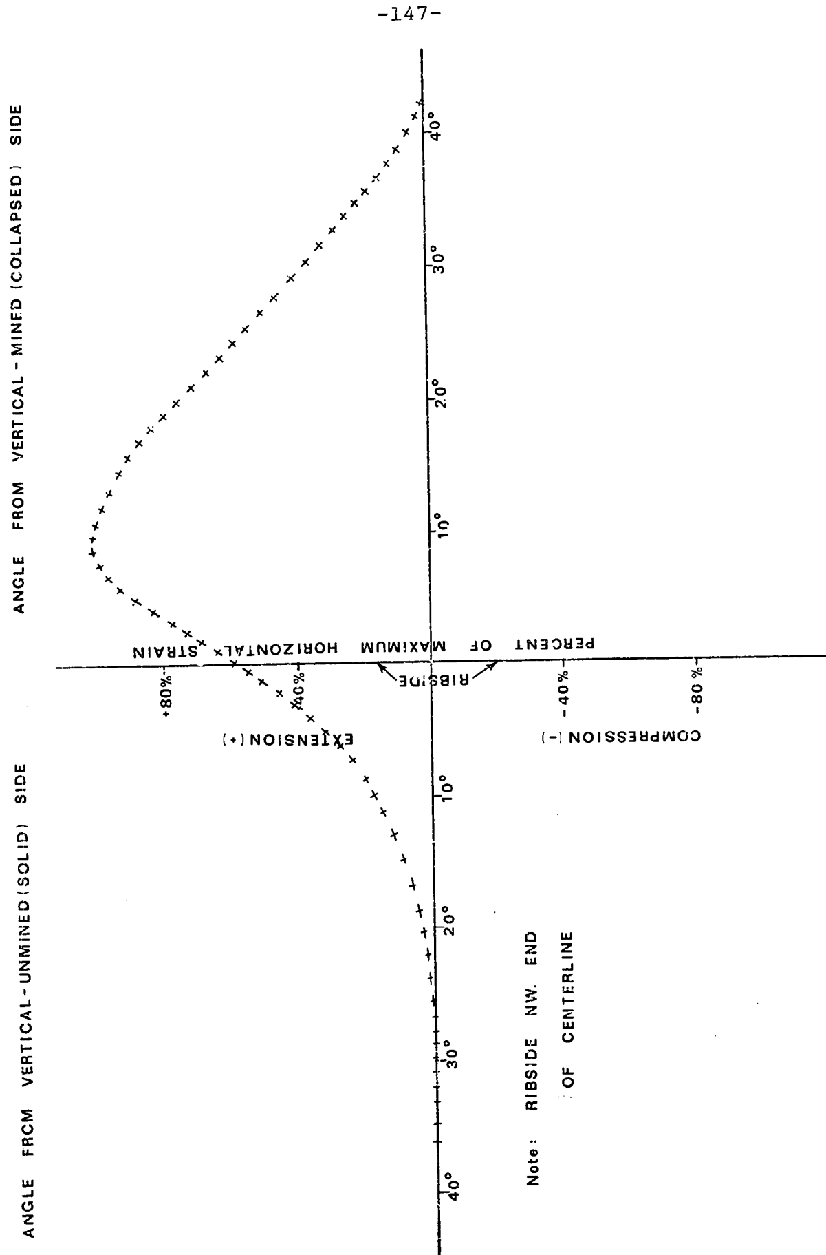
FIG 45 HORIZONTAL STRAIN DISTRIBUTION FOR SUPERCRITICAL CONDITIONS (4N LW)
