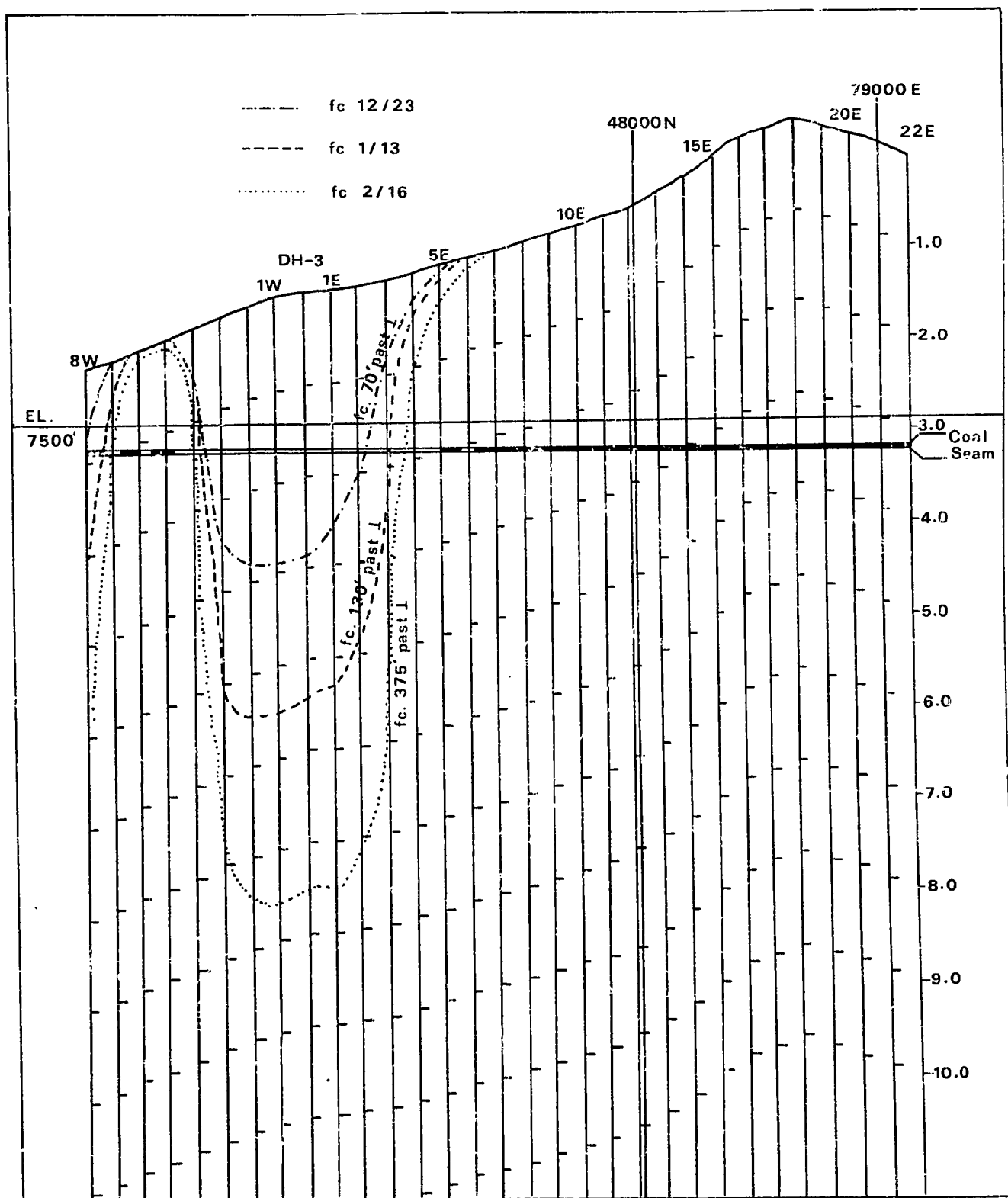
FIG 18 TRAVELING SUBSIDENCE PROFILES (8W-22E) York Canyon Mine Test Panel.
