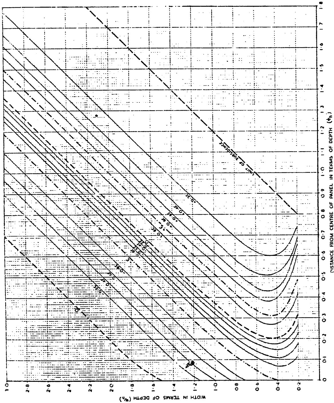
FIG 57 GRAPH FOR PREDICTING STRAIN PROFILES (NATIONAL COAL BOARD, 1975)
