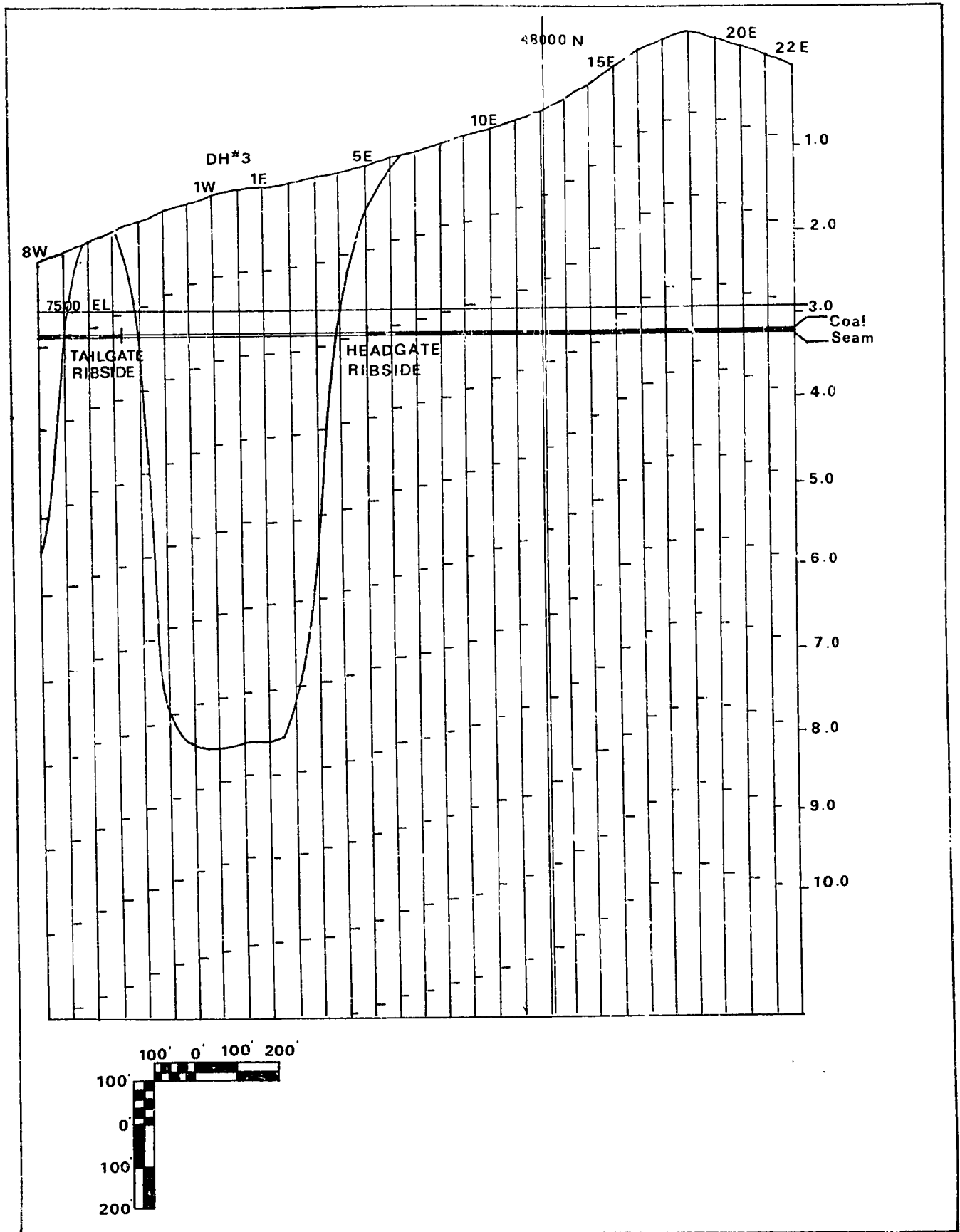
FIG 16 FINAL SUBSIDENCE PROFILE — PANEL PERPENDICULAR (8W-22E)
