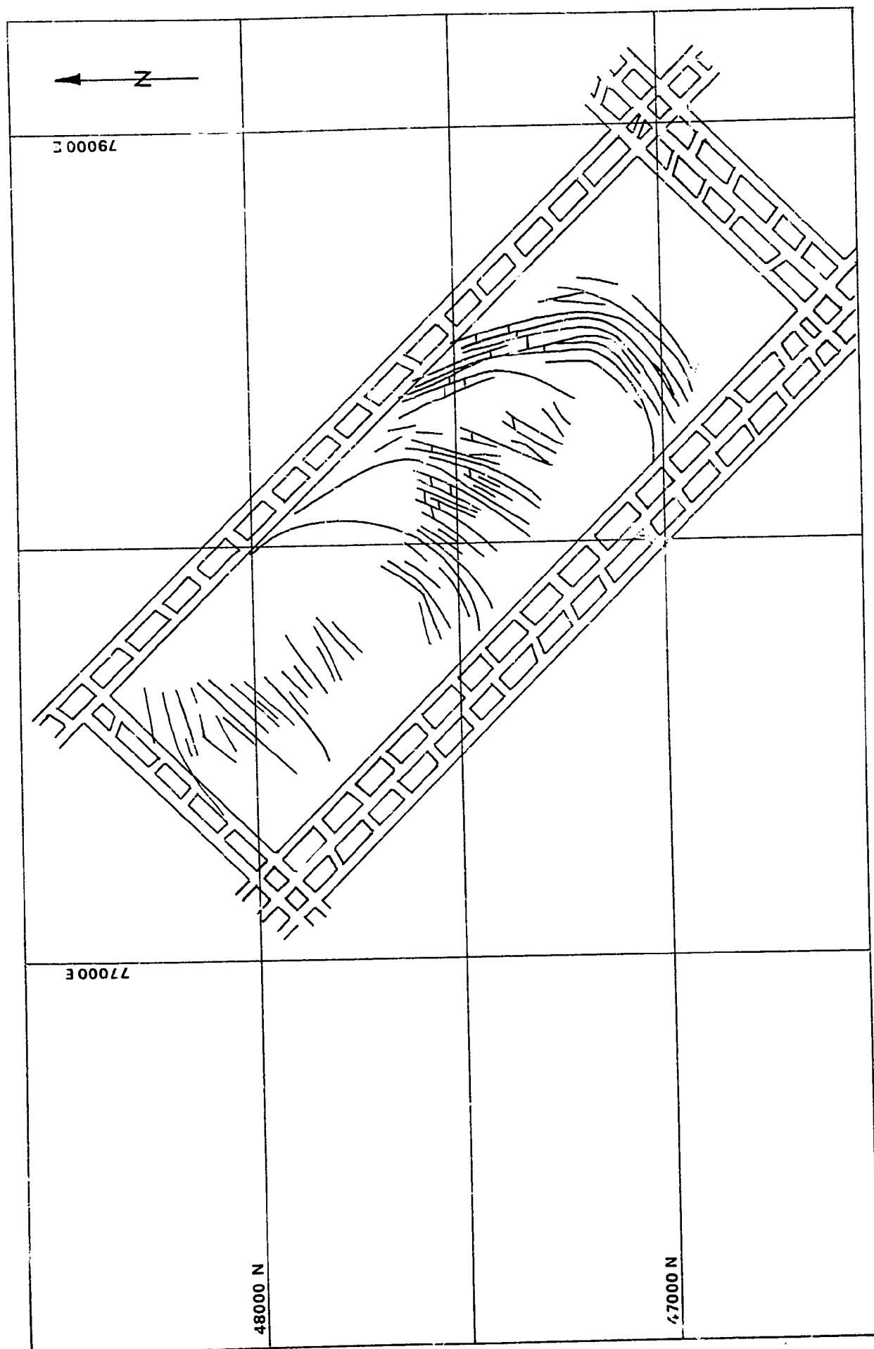
FIG 34 SURFACE CRACKS OVER 4N L.W. PANEL. York Canyon Mine.
