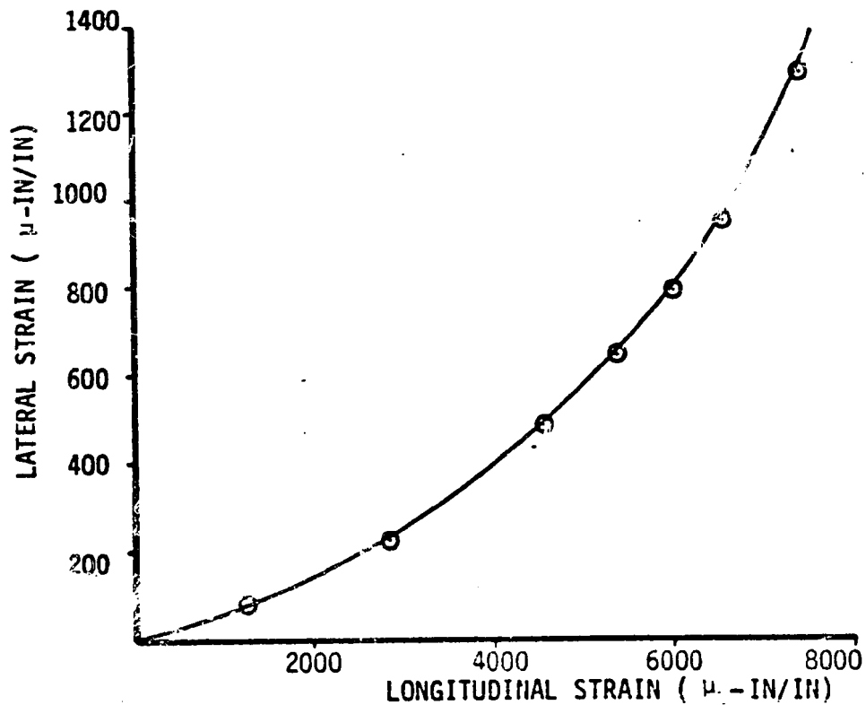
FIG. I-6 UNIAXIAL COMPRESSION TEST RESULTS - ROOF SANDSTONE
