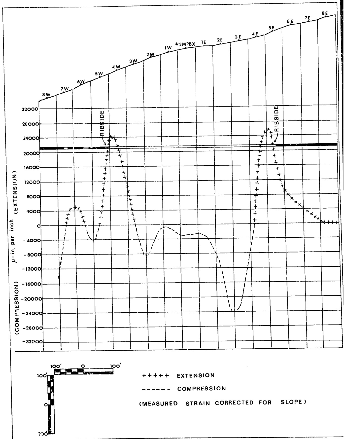
FIG 54 STABILIZED HORIZONTAL STRAIN - PANEL PERPENDICULAR
