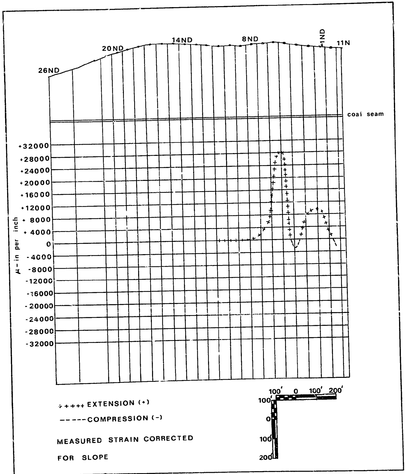
FIG 52 DYNAMIC HORIZONTAL-STRAIN NORTH DIAGONAL York Canyon Mine Test Panel 4N Fc at 8N Sept. 30, 1975
