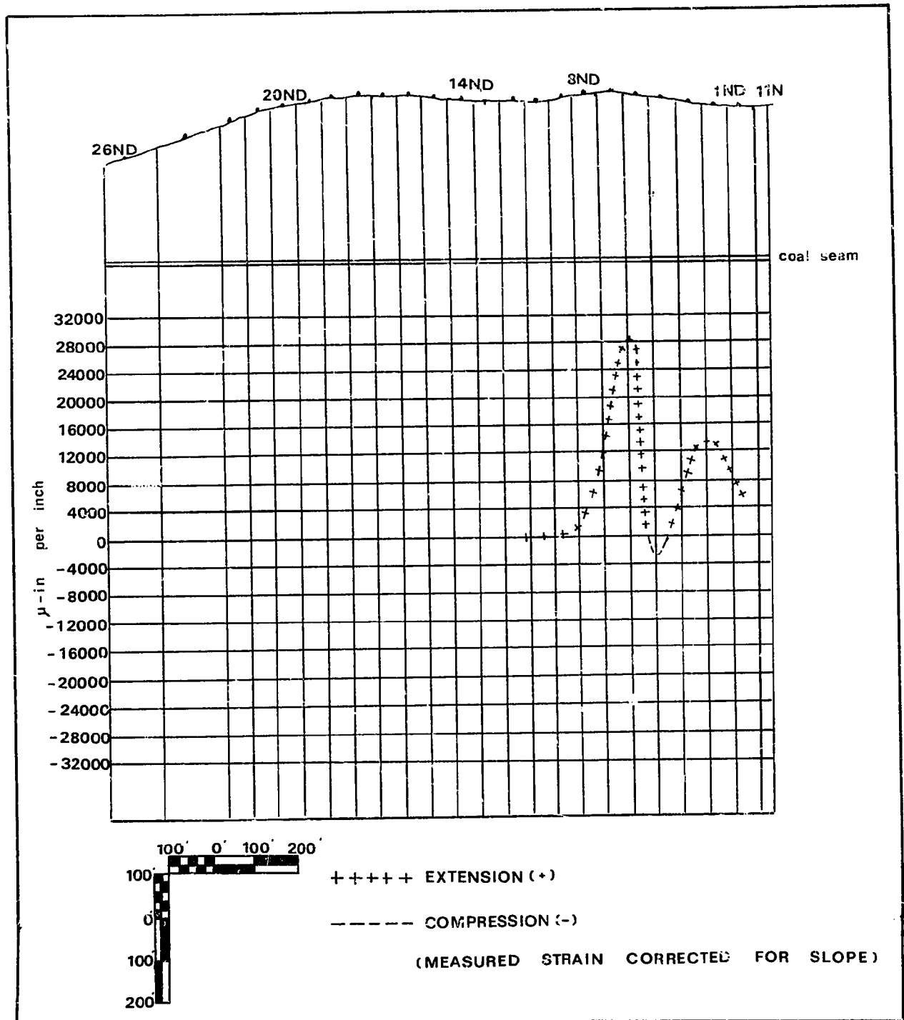
FIG 55 STABILIZED HORIZONTAL STRAIN - NORTH DIAGONAL. York Canyon Mine Test Panel 4N. Fc.1000' Past Diagonal. Jan. 1, 1976
