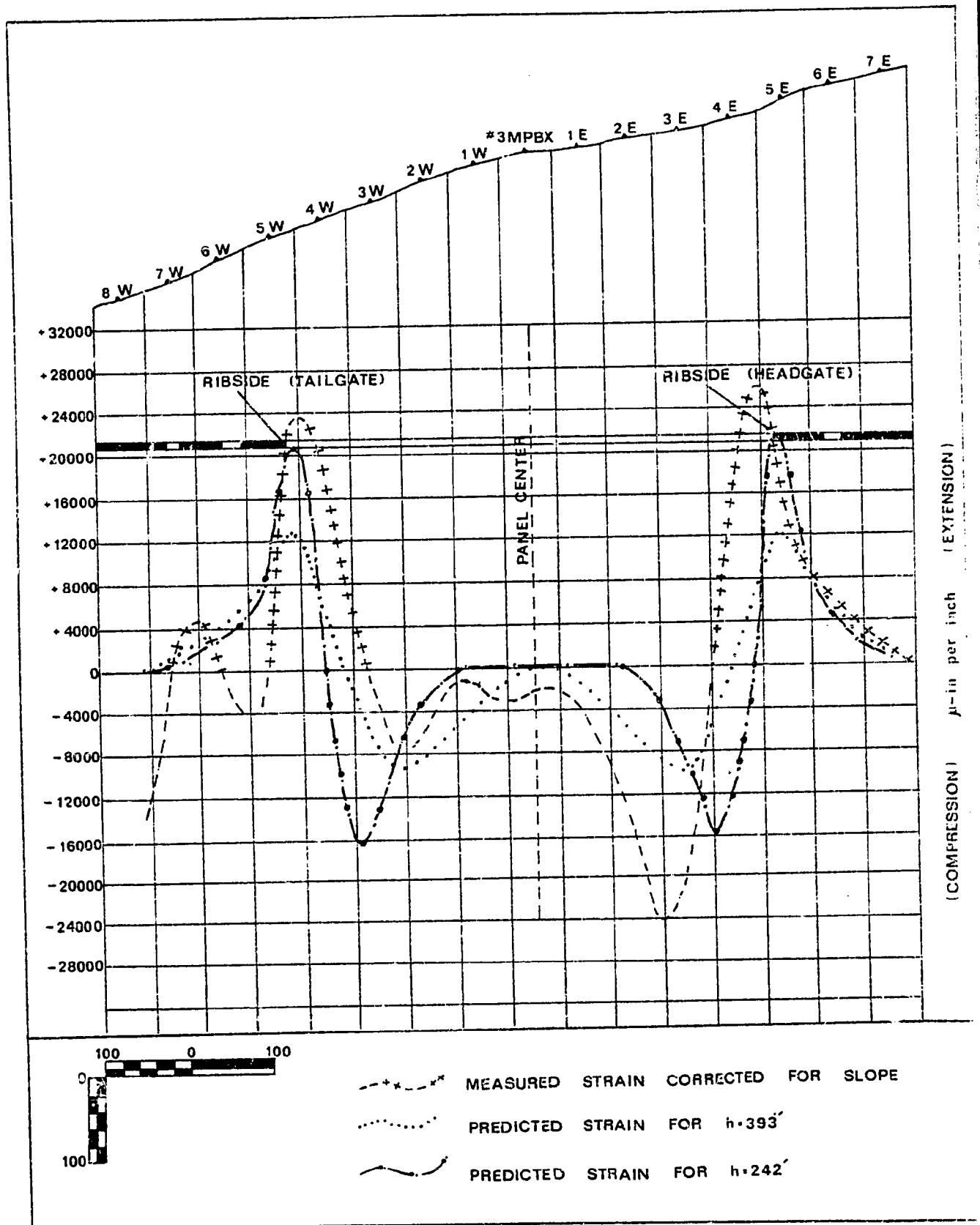
FIG 58 MEASURED VS. PREDICTED STABILIZED HORIZONTAL STRAINS - PANEL PERPENDICULAR.
