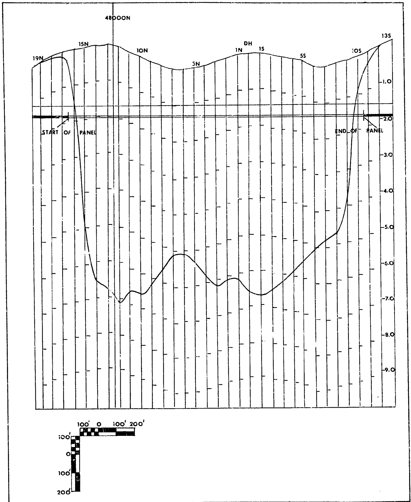
FIG 15 FINAL SUBSIDENCE PROFILE—PANEL CENTERLINE (19N—13S)
