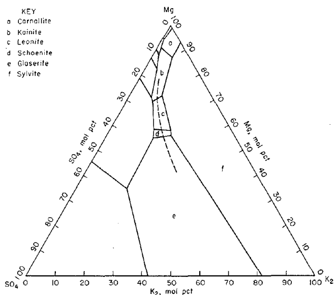
FIGURE 17. - Crystallization path of 10,000-gal brine sample in a solar evaporation pond.
