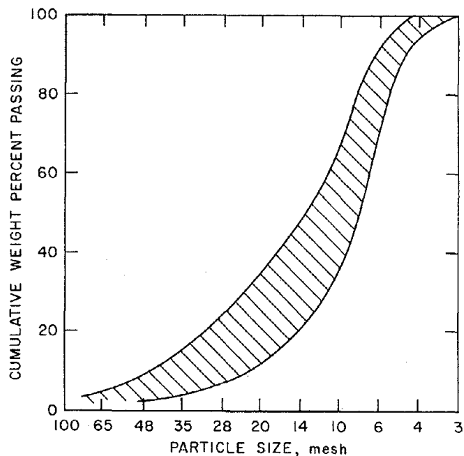
FIGURE 4. - Size distribution range of crushed evaporites from all brine harvests.
