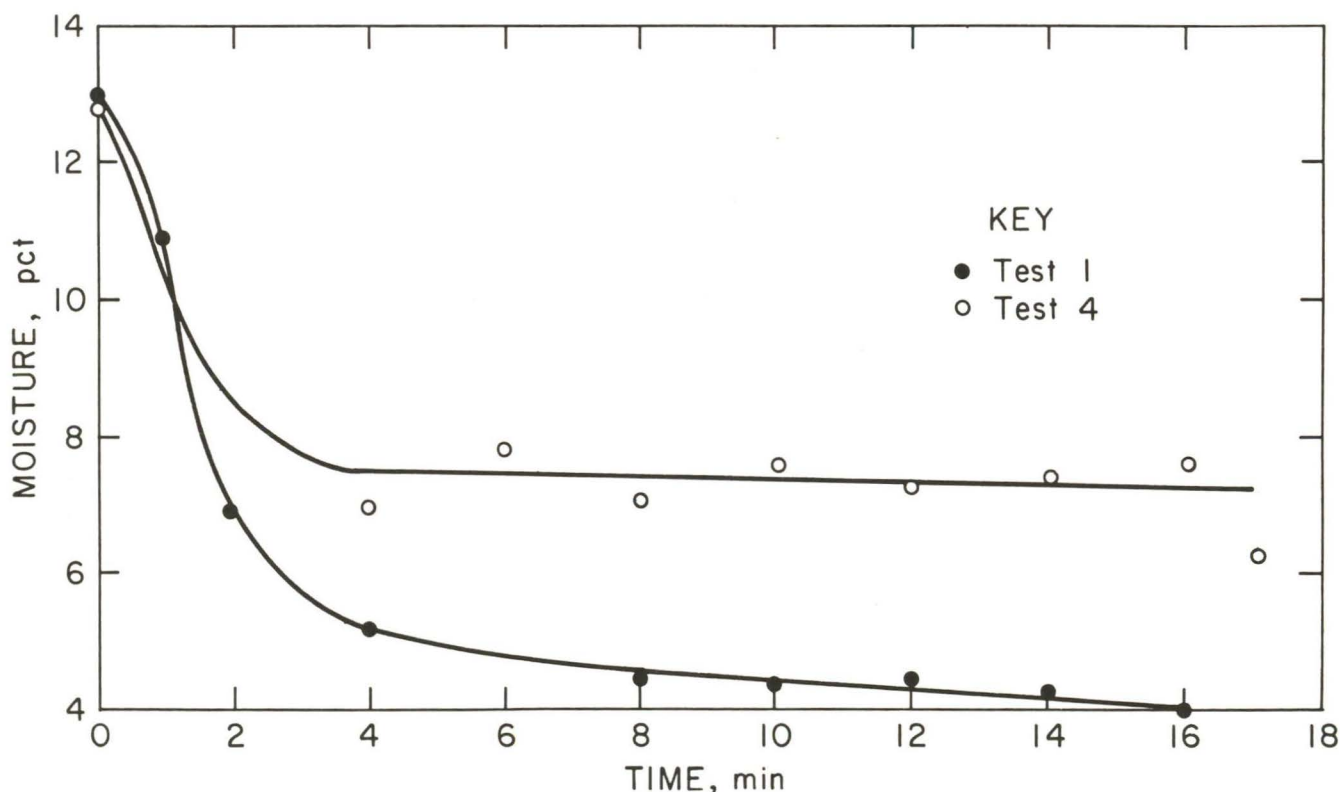
FIGURE 2. - Drying rate curves, Illinois No. 6 coal, minus 1/4 in plus 28 mesh.
