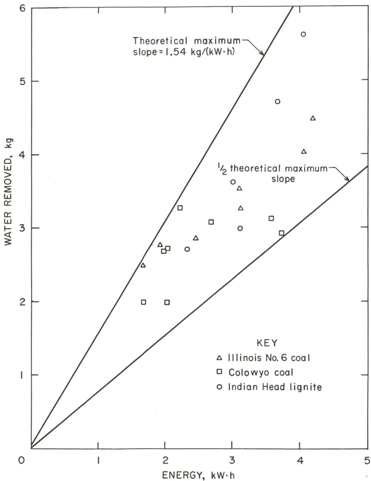
FIGURE 3. - Drying efficiency.
