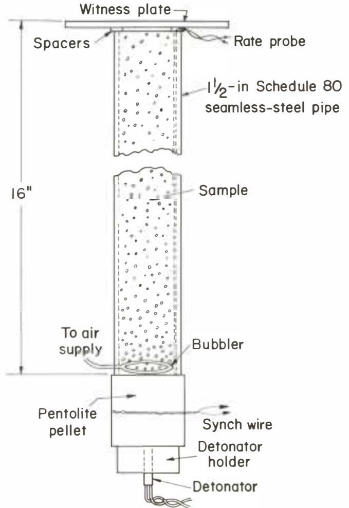
Figure 2.—Bureau of Mines' gap test for liquids.
