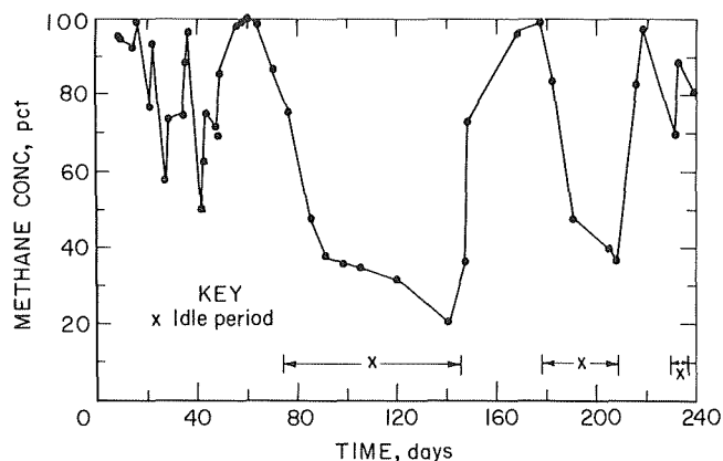
FIGURE 12. - Surface methane concentrations in gas flow.
