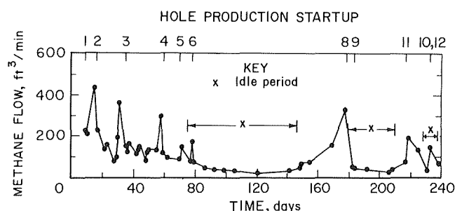
FIGURE 17. - Methane flow in return air.
