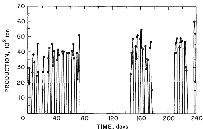
FIGURE 10. - Daily longwall coal production.
