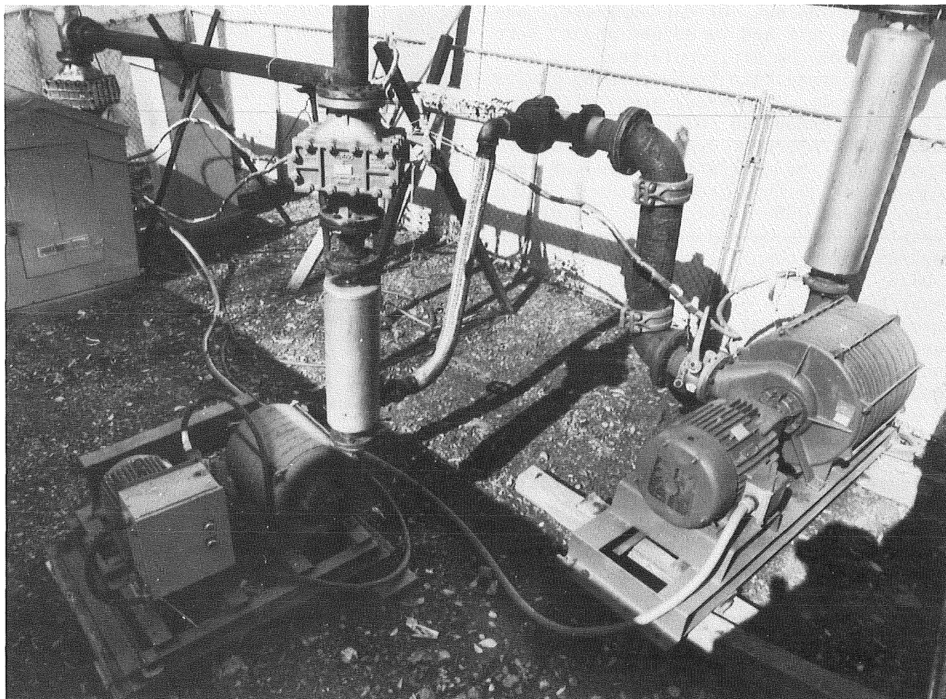
FIGURE 4. - Surface exhausters.
