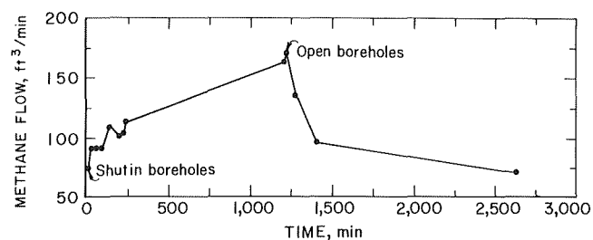
FIGURE 18. - Effects of cross-measure system on methane flow in return air.
