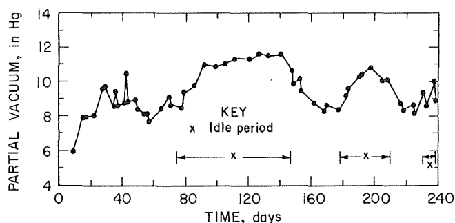
FIGURE 15. - Partial vacuum measured at surface exhauster.
