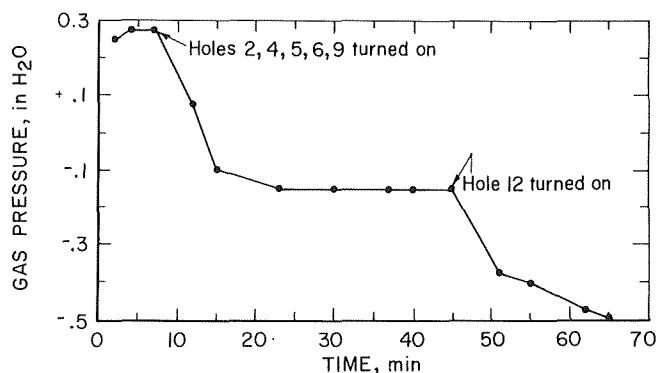
FIGURE 16. - Interference test using hole 11.
