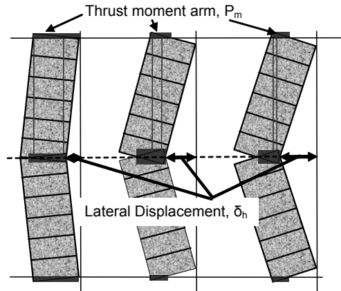
Figure 7. Diagram showing that increased lateral displacement of the stopping reduces the arch thrust which reduces the transverse load capacity of the stopping.
