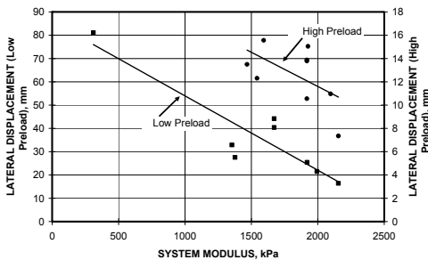
Figure 10. Lateral displacement decreases as the modulus of elasticity of the deformable material of the wall increases, causing an increase in system modulus.
