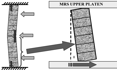
Figure 5. Simulating rigid arching in the NIOSH Mine Roof Simulator.
