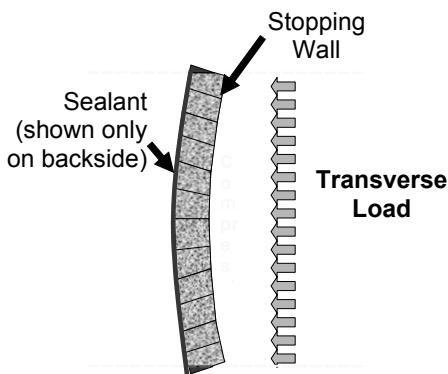
Figure 3. In freestanding evaluation, the sealant provides the main resistance to transverse loading.
