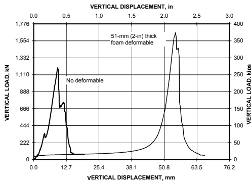
Figure 2. Comparison of a block stopping wall's response to vertical loading with and without a foam, deformable layer.
