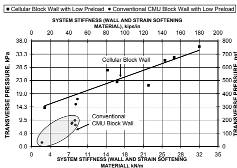
Figure 12. Performance comparison showing the transverse load capacity as a function of the system modulus between stopping walls constructed from cellular concrete blocks and Portland concrete blocks (CMU's).
