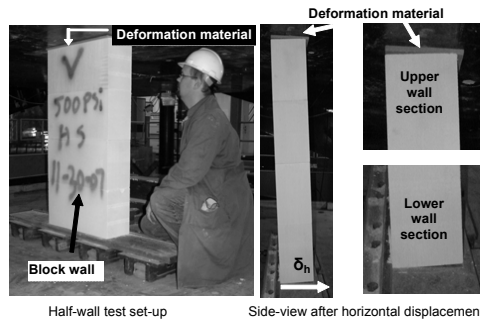
Figure 8. Deformable material placed at the roof interface in the MRS testing program.
