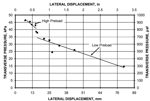
Figure 9. Transverse pressure capacity is reduced as the lateral displacement of the wall increases.
