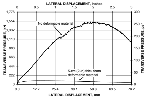
Figure 4. Under arch loading conditions, foam layer can severely degrade transverse load capacity of a stopping. This figure shows the results of the MRS transverse loading tests of a stopping with and without a foam layer.
