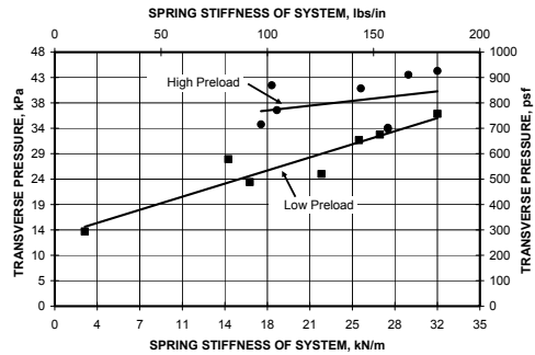
Figure 11. Transverse pressure capacity is increased as the system stiffness of the material of the wall increases due to the use of a higher modulus strain-softening material.
