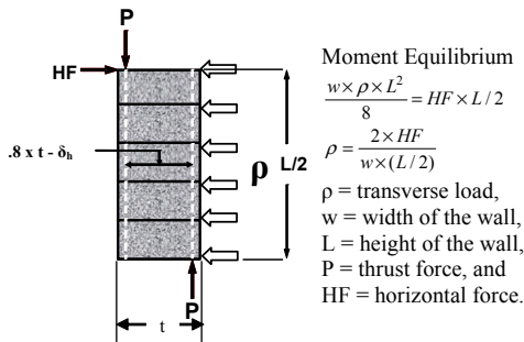
Figure 6. Moment equilibrium equations for half-wall section of stopping subjected to transverse loading.
