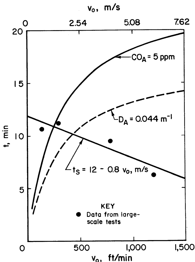
Figure 2.—Times to produce CO and smoke alarm levels for smoldering coal for an entry cross section of 7.53 \text{ m}^2 .
