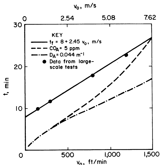
Figure 5.—Times to produce CO and smoke alarm levels for flaming coal fires for an entry cross section of 7.53 \text{ m}^2 .
