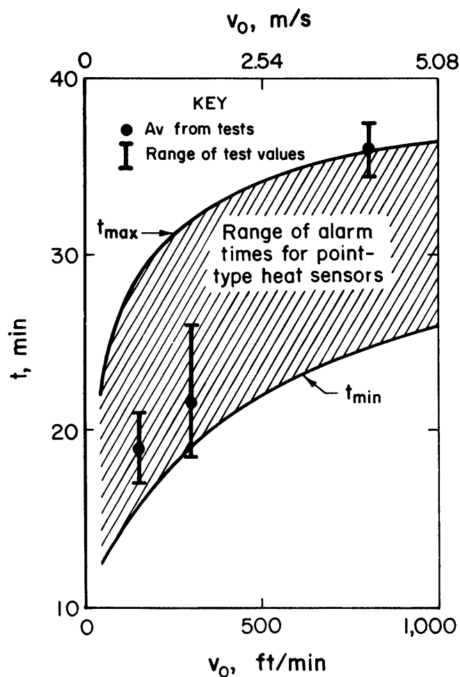
Figure B-1.—Thermal alarm times as function of air velocity for surface fire gallery tests. ( A_o = 7.53 \text{ m}^2 )
