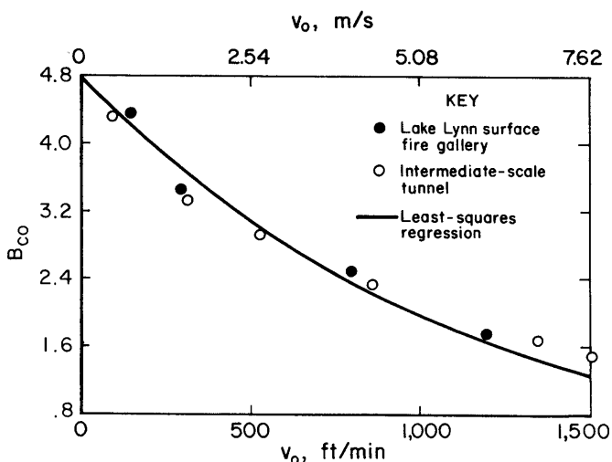
Figure 3.—Production constant for CO for flaming coal fires. The curve is defined by the expression B_{CO} = 4.80 e^{-0.175 v_o, m/s} .
