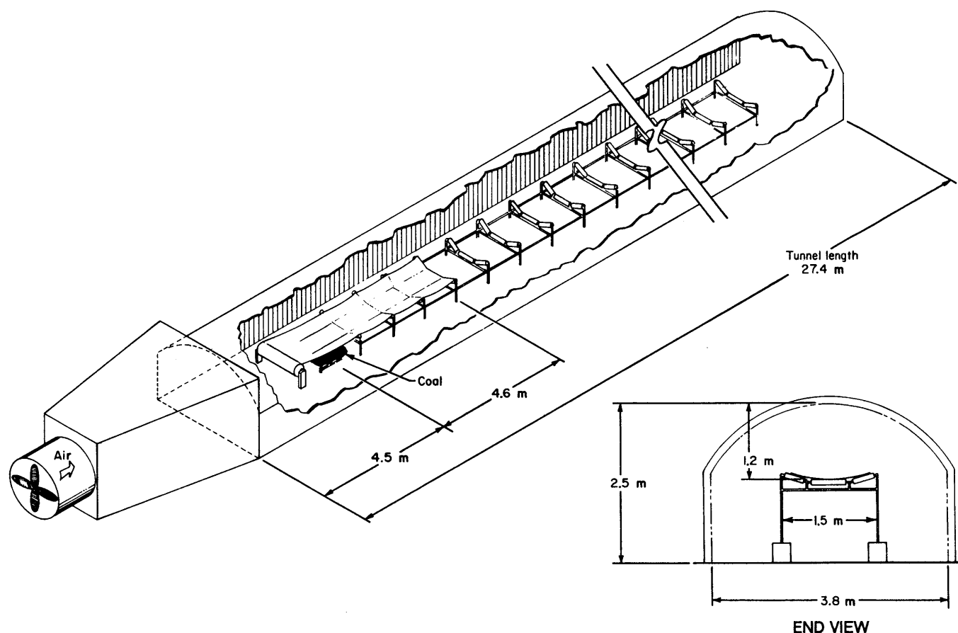
Figure 1.—Schematic of Lake Lynn aboveground fire gallery.
