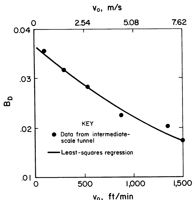
Figure 4.—Production constant for smoke for flaming coal fires. The curve is defined by the expression B_D = 0.037 e^{-0.1 v_o} , m/s .
