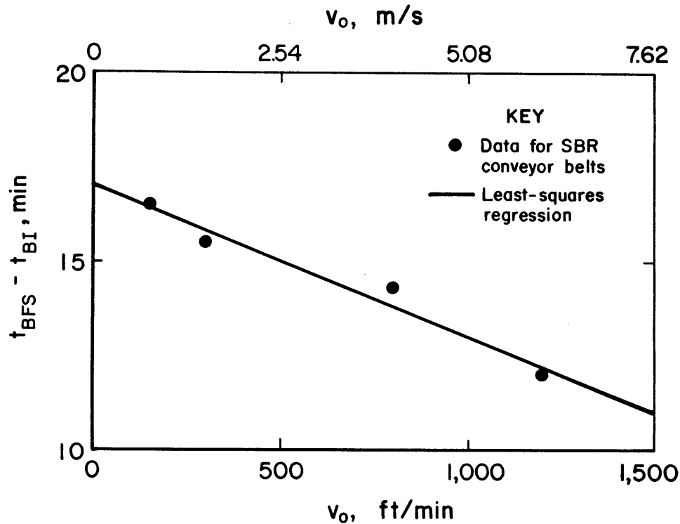
Figure 6.—Average times from belt ignition to onset of belt flame spread for SBR conveyor belts. The curve is defined by the expression t_{BFS} - t_{BI} = 17 - 0.8v_o , m/s.
