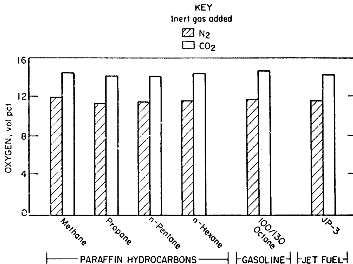
FIGURE 8. Comparison of minimum oxygen concentrations required for flame propagation of various fuel vapor-air-inert gas mixtures at 80°F and atmospheric pressure.
