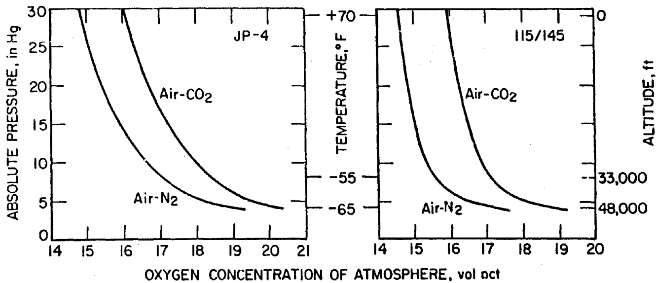
FIGURE 9. Minimum oxygen concentrations required for flame propagation of JP-4 and aviation gasoline (115/145) sprays in air-CO 2 and air-N 2 atmospheres at various pressure altitude conditions.
