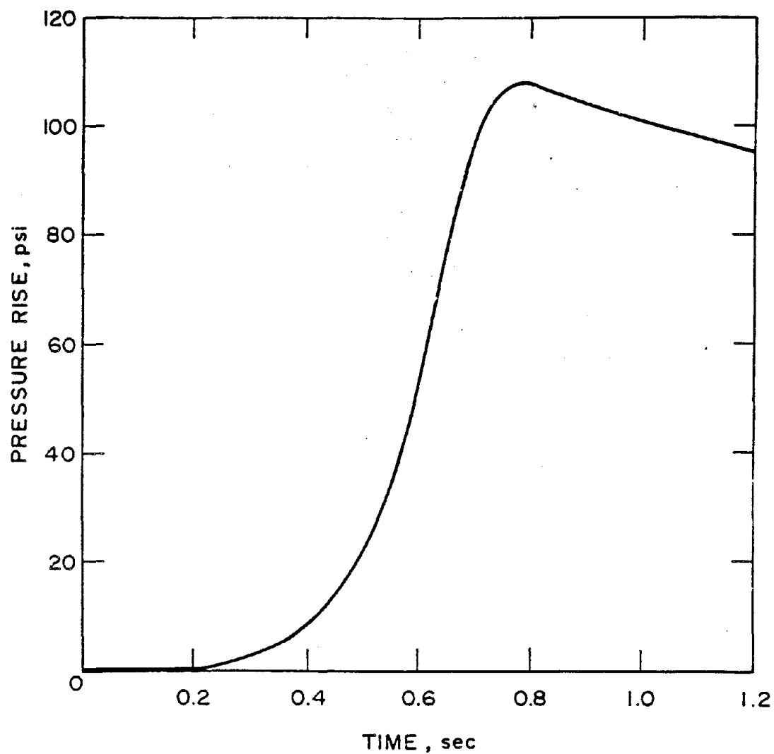
FIGURE 31. Pressure history for the explosion of a stoichiometric methane-air mixture (75°F) in a 12-ft diameter sphere at atmospheric pressure.
