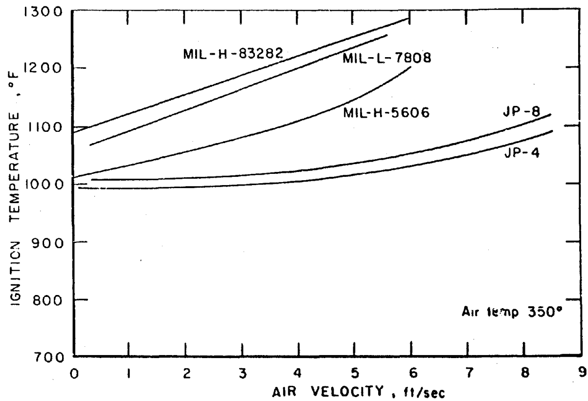
FIGURE 27. Comparison of ignition temperatures of aircraft fuels or fluids at various air velocities with a heated 2-inch diameter by 24-inch long steel target.
