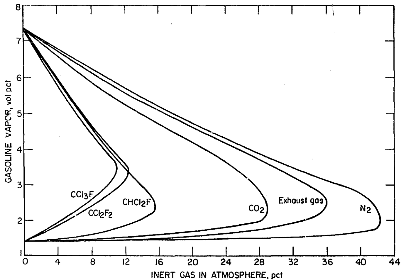
FIGURE 43. Effectiveness of various inerting agents on limits of flammability of gasoline vapor-air mixtures at 80°F and atmospheric pressure.
