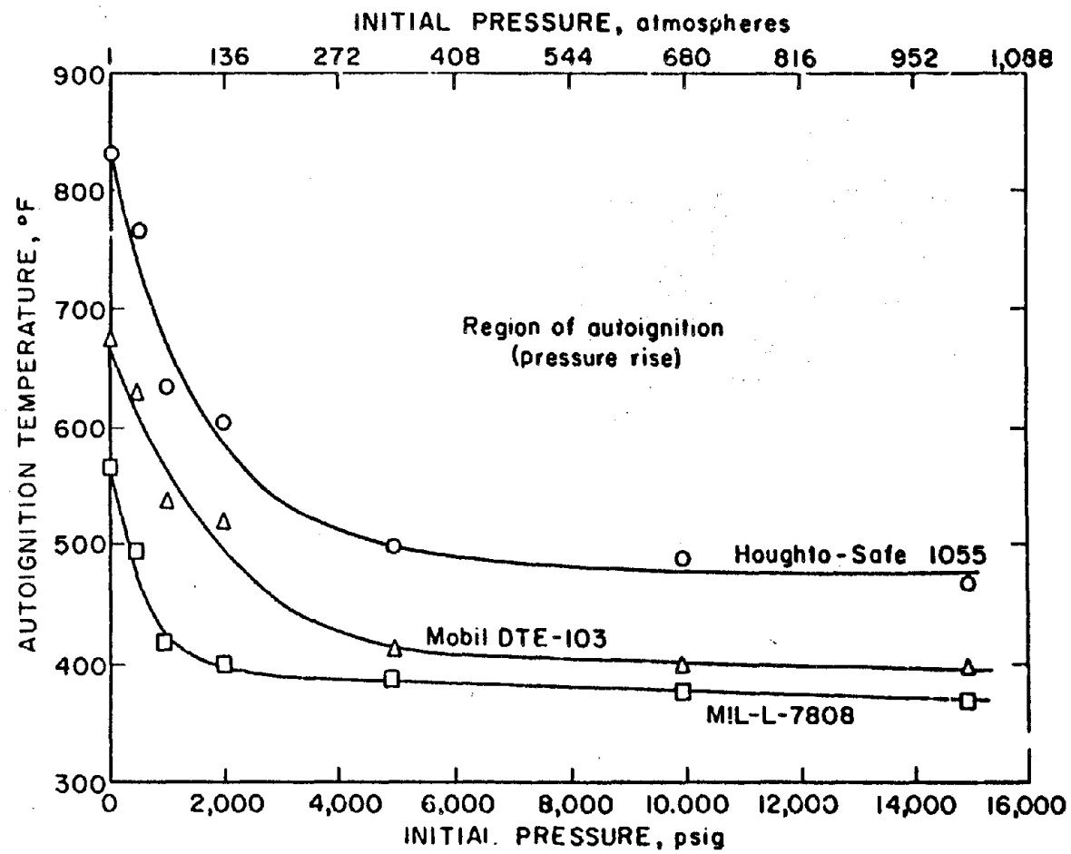
FIGURE 25. Minimum autoignition temperatures of Houghto-Safe-1055, Mobil DTE-103, and MIL-L-7808 lubricants in air at various initial pressures.
