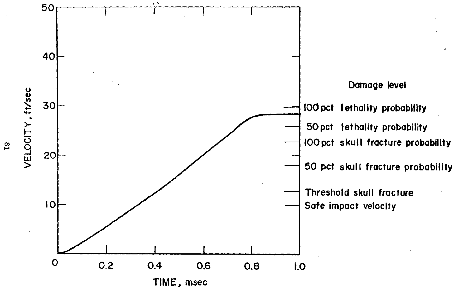
FIGURE 42. Velocity-time profile for translation of 1/8-inch diameter nylon sphere.
