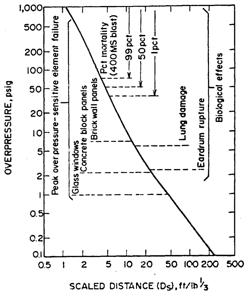
FIGURE 39. Peak overpressure and approximate damage potentials from hemispherical TNT surface bursts.
