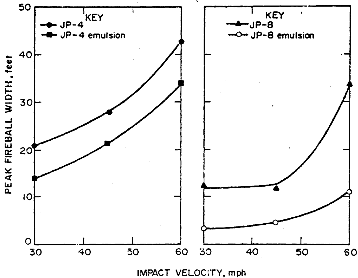
FIGURE 35. Variation of peak fireball width with impact velocity for vertical fuel drops with 5 gallon metal container.
