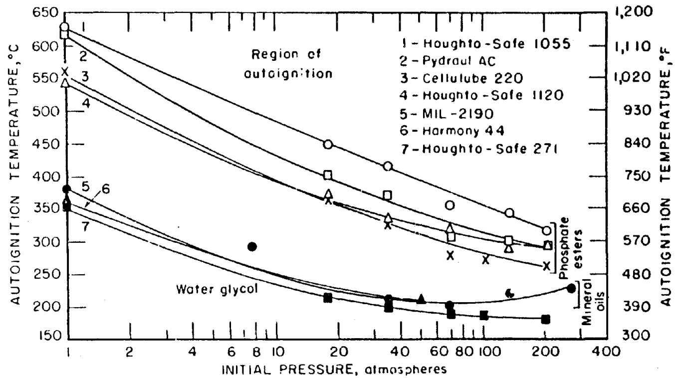
FIGURE 24. Minimum autoignition temperatures of phosphate ester, mineral oil, and water-glycol lubricants in air at various initial pressures.
