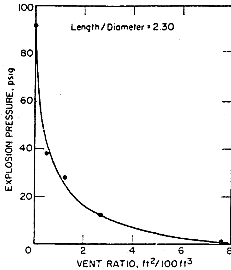
FIGURE 34. Effect of vent ratio on explosion pressure for 3% propane-air mixtures (75°F) in a 3 ft 3 tank at atmospheric pressure.
