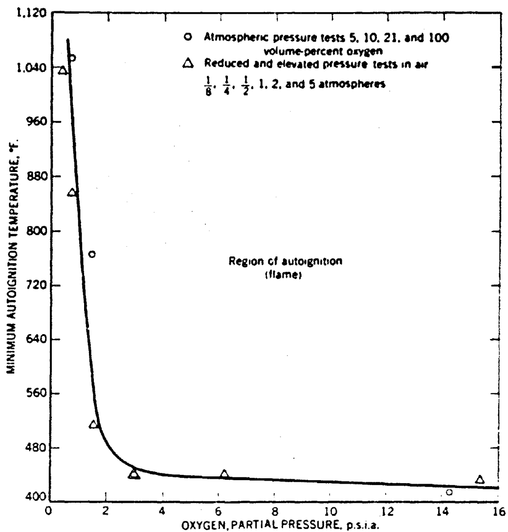
FIGURE 20. Effect of oxygen partial pressure on the minimum auto-ignition temperature of JP-6 fuel vapor-oxygen-nitrogen mixtures at various total pressures under static conditions.
