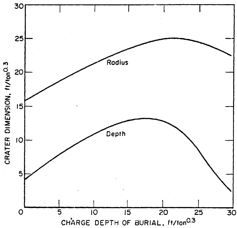
FIGURE 40. Crater dimensions scaled to 1-ton charges of TNT or equivalent buried in dry soil.
