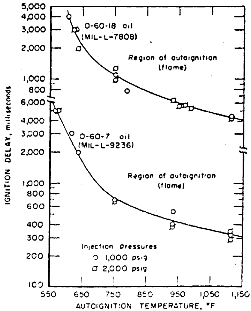
FIGURE 21. Variation of ignition delay with temperature in auto-ignition of MIL-L-7808 and MIL-L-9236 engine oils in air (1 atm) at 1000 and 2000 psig injection pressures.
