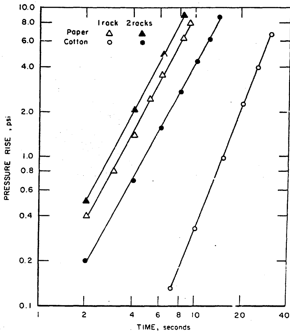
FIGURE 33. Pressure rise vs time for the burning of paper and cotton sheeting ( 0.035 \text{ oz/ft}^2 ) in air on single and double burning racks in a 216 \text{ ft}^3 chamber (1 atm).
