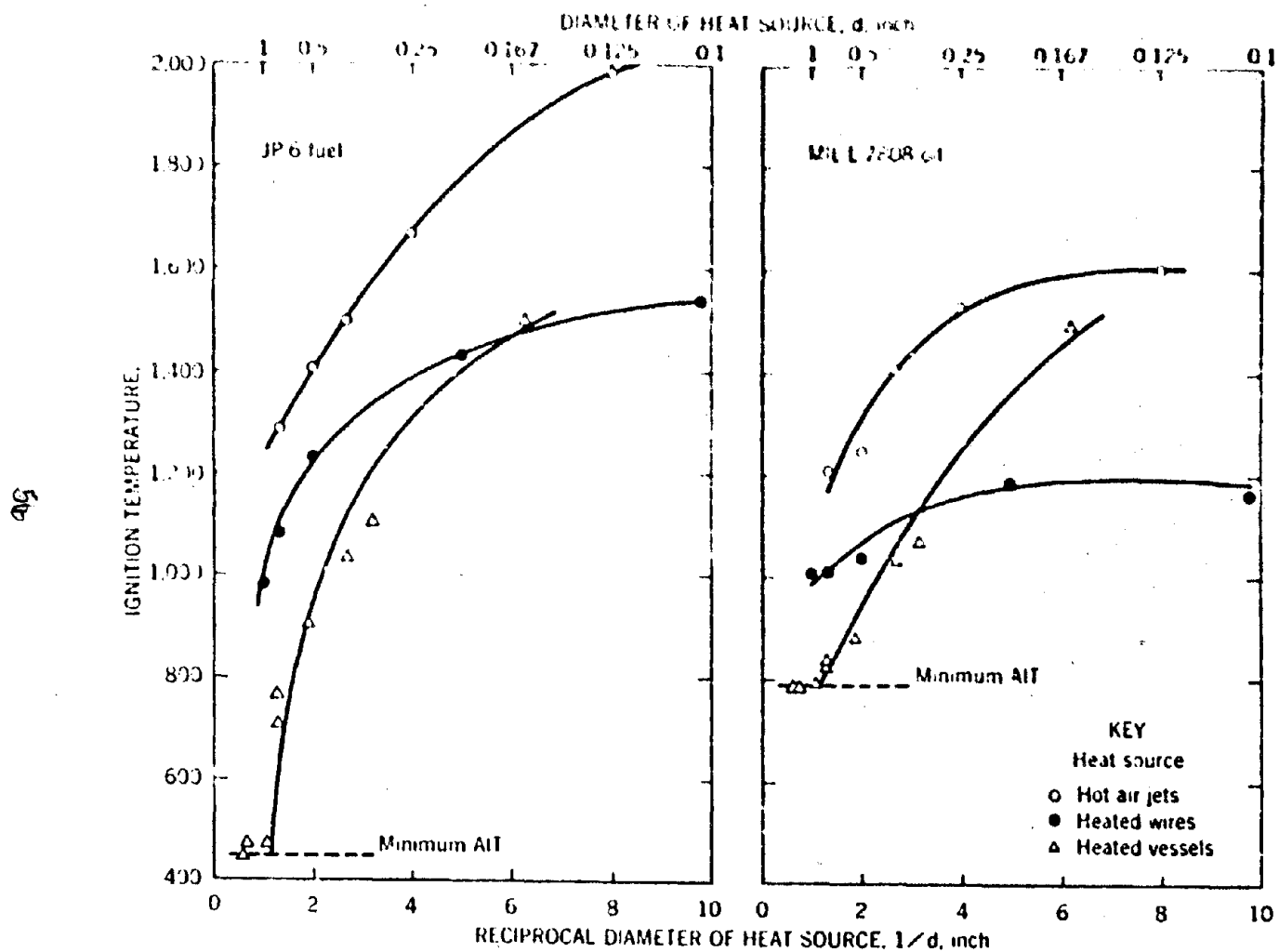
FIGURE 30. Variation of hot gas and hot surface ignition temperatures with reciprocal diameter of heat source for JP-6 fuel and MIL-L-7808 engine oil vapor-air mixtures.
