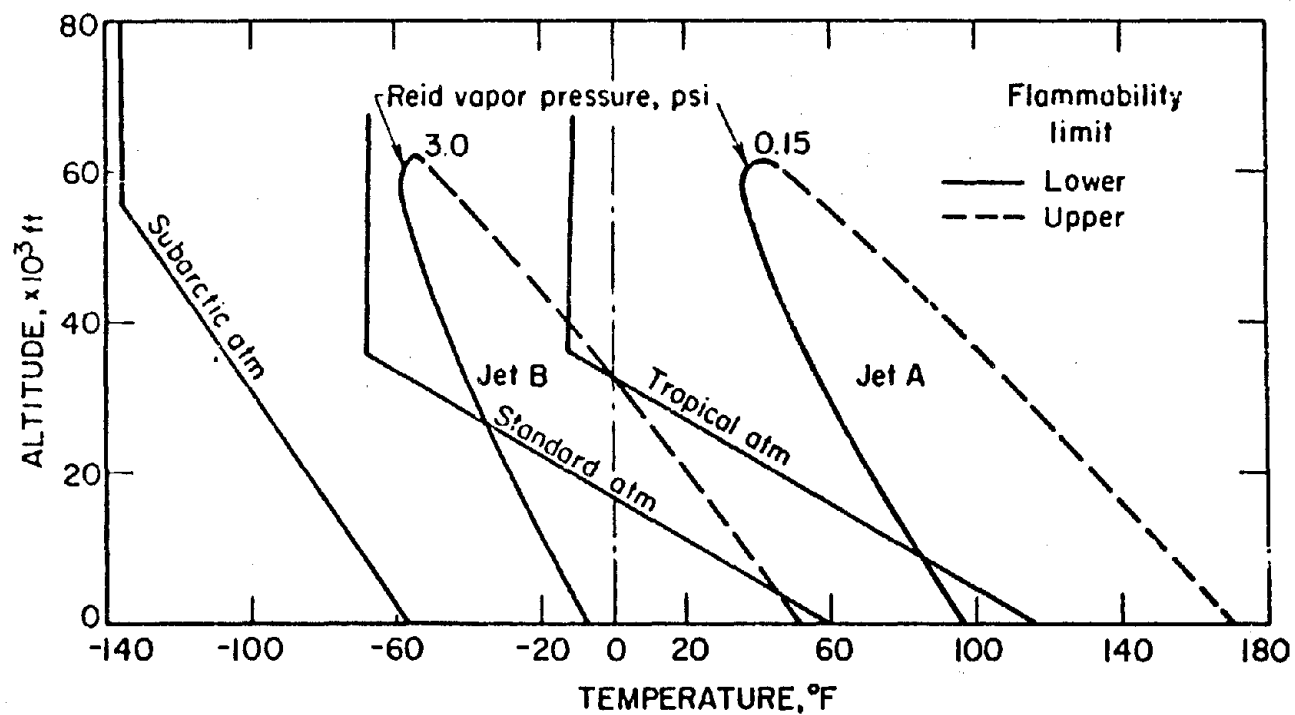
FIGURE 4. Altitude-temperature limits of flammability for Jet A and Jet B type fuels in air. (Large quenching effects at high pressure altitudes.)
