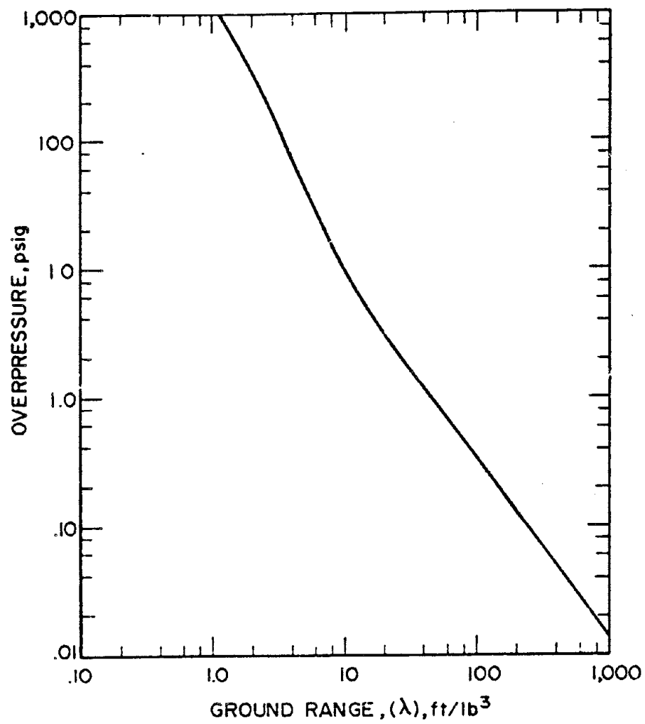
FIGURE 38. Peak overpressure vs scaled distance for hemispherical TNT surface bursts.
