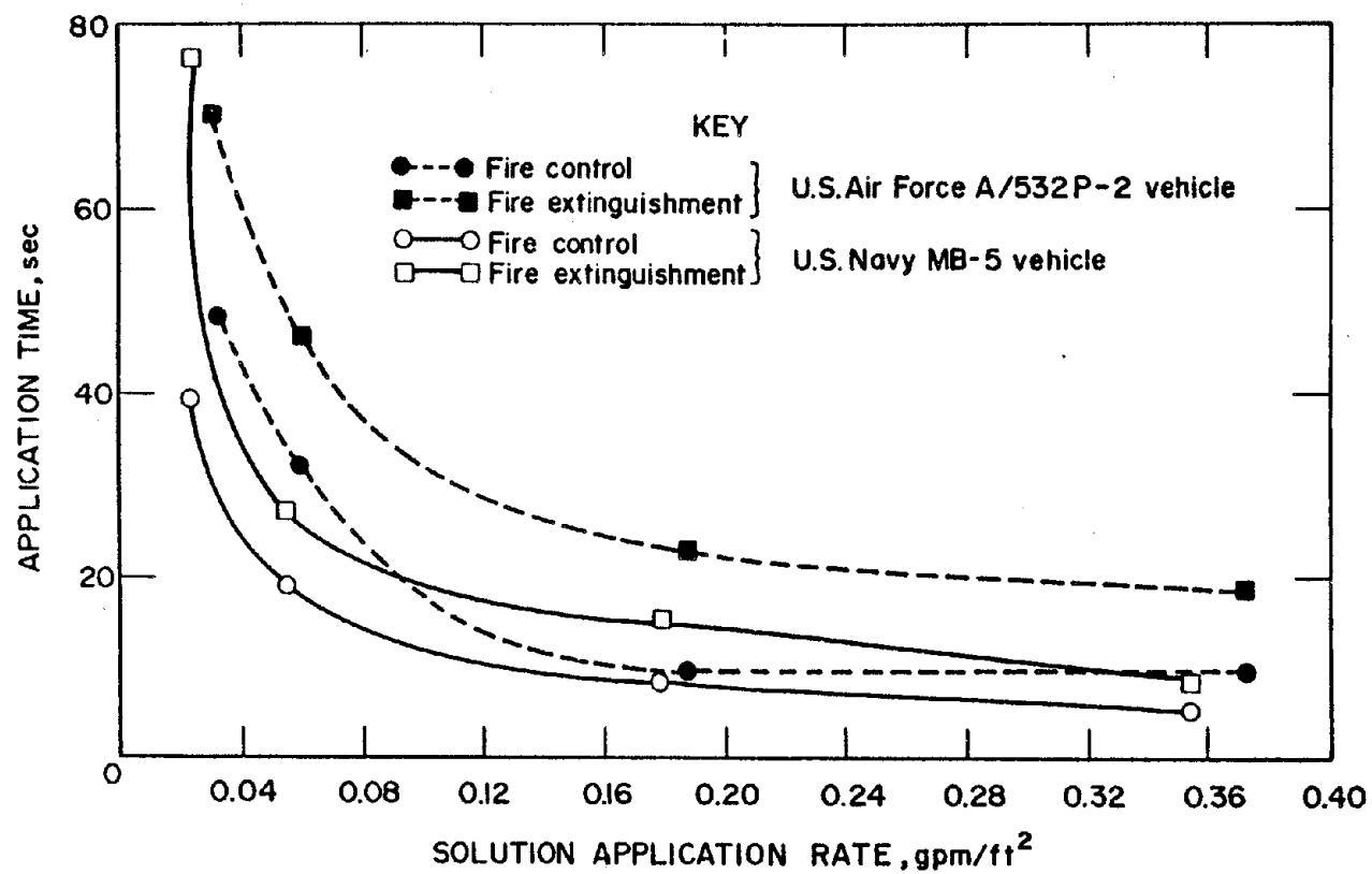
FIGURE 47. Fire control and extinguishing times as a function of AFFF solution application rate for Jet A fuel fires using the Air Force A/S32P-2 and U. S. Navy MB-5 trucks.
