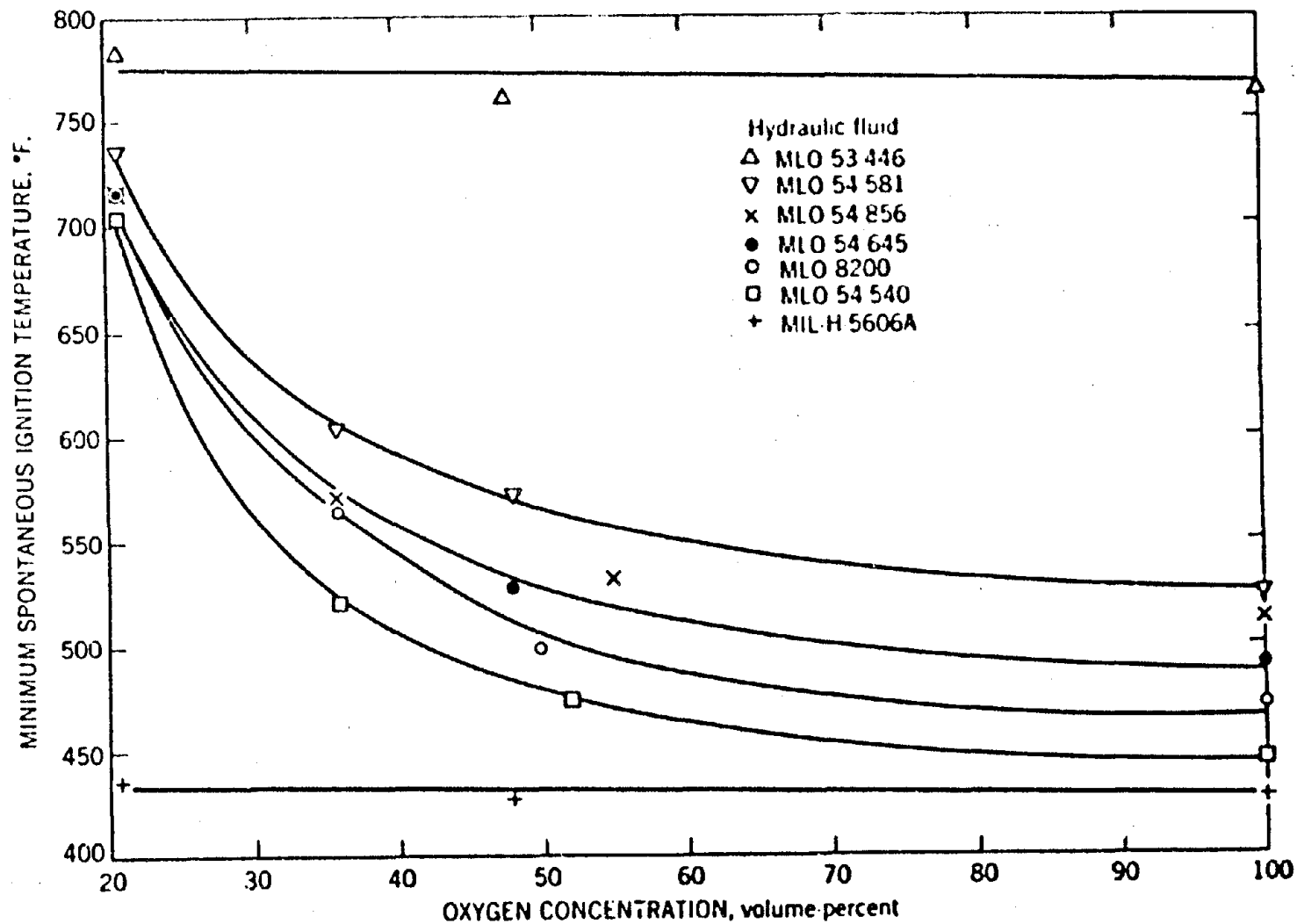
FIGURE 23. Effect of oxygen concentration on the minimum auto-ignition temperature of seven hydraulic fluids in oxygen-nitrogen mixtures (1 atm) under static conditions.
