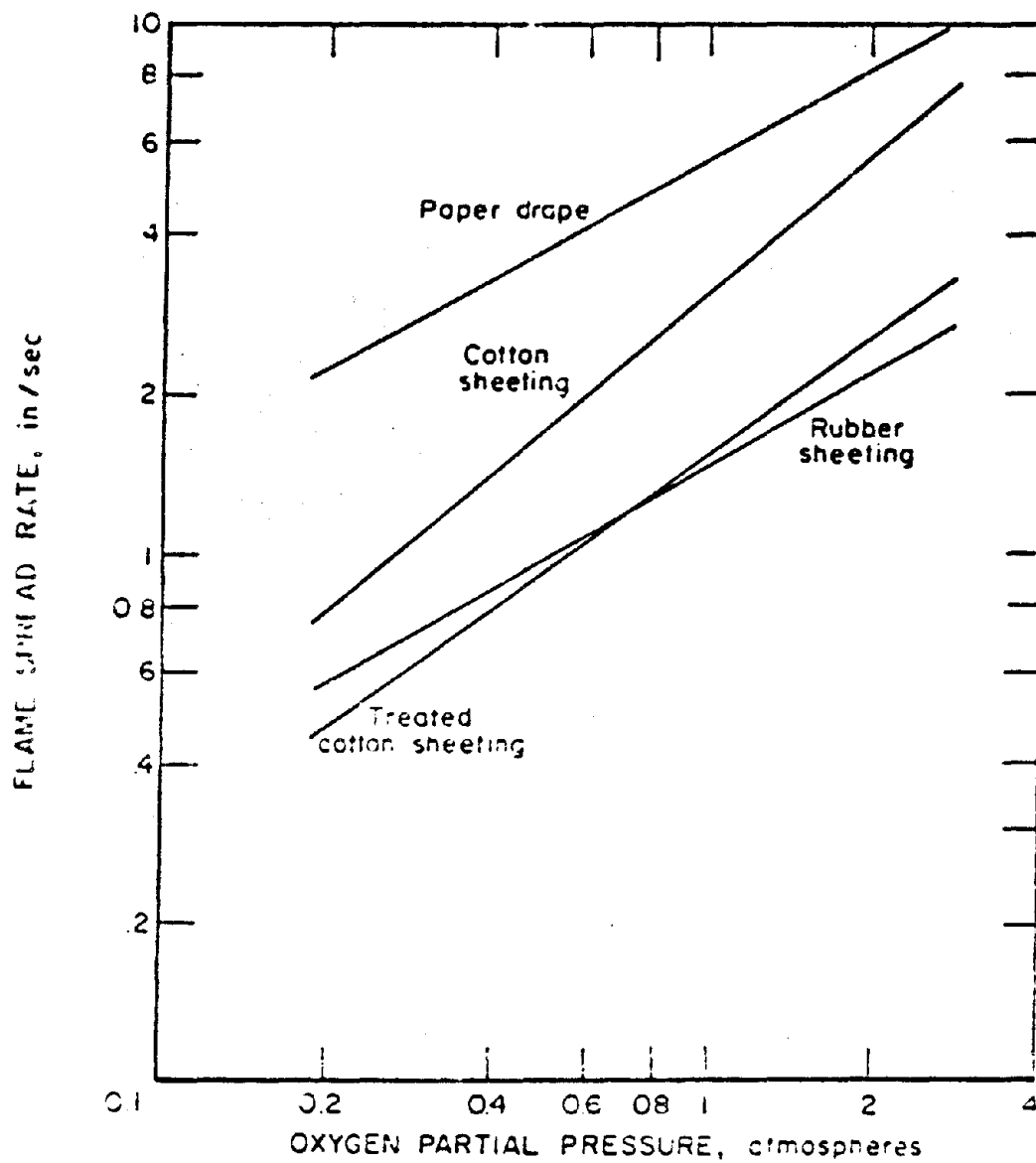
FIGURE 13. Flame spread rates of paper, cotton, and rubber combustibles in oxygen-nitrogen mixtures ( \geq 21\% \text{ O}_2 ) at 0.2 to 6 atmospheres total pressure ( 45^\circ angle burning).
