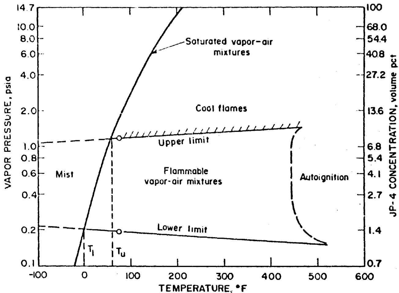
FIGURE 2. Flammability diagram of JP-4 in air at atmospheric pressure.
