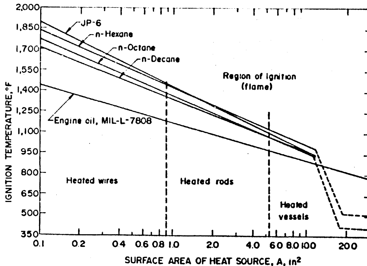
FIGURE 29. Hot surface ignition temperature as a function of the surface area of the heat source for various hydrocarbon fuels and an engine oil in near-stagnant air.
