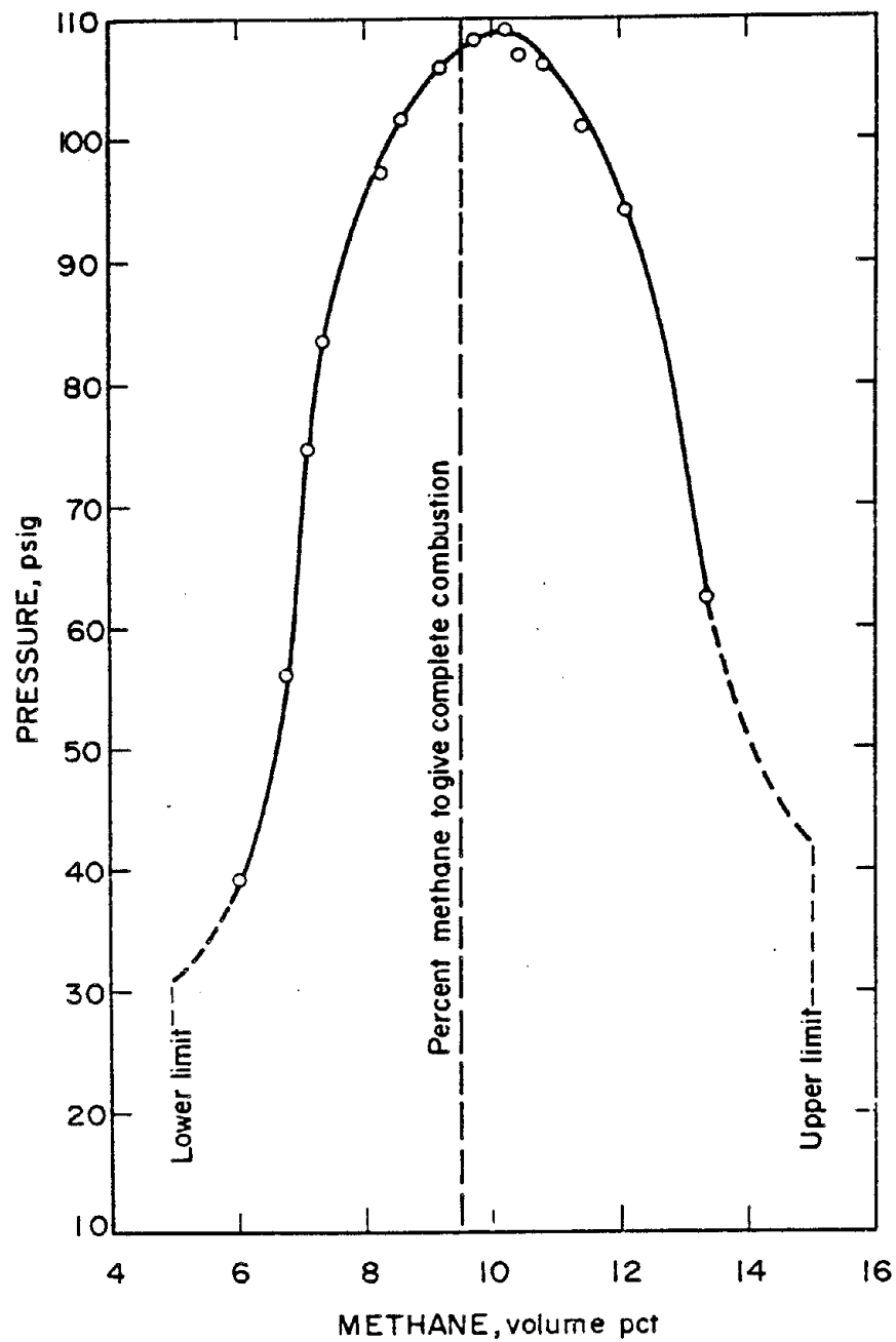
FIGURE 32. Effect of fuel concentration on explosion pressure for methane-air mixtures (75°F) in a 244 in 3 vessel at atmospheric pressure.
