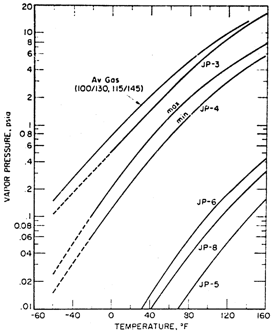
FIGURE 1. Reid vapor pressure vs temperature for various aircraft fuels.
