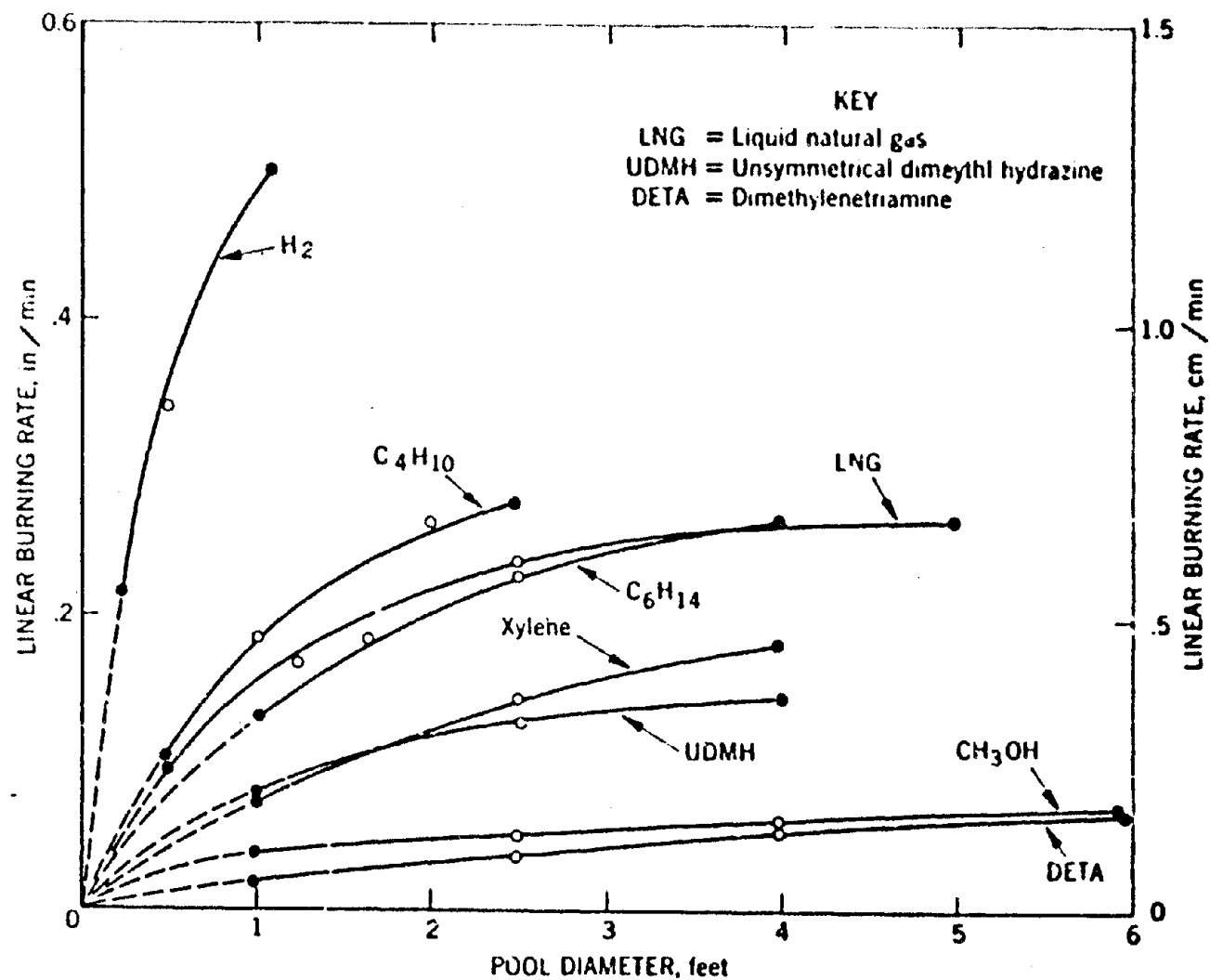
FIGURE 12. Linear burning rate of combustible liquids as a function of pool diameter.
