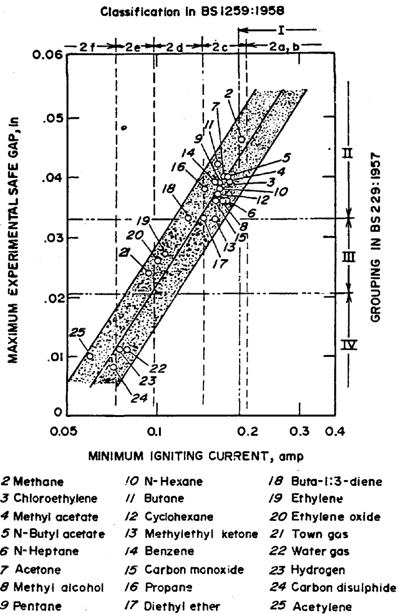
FIGURE 48. Correlation of maximum experimental safe gap with minimum igniting current (limits of 95% confidence shown shaded).
