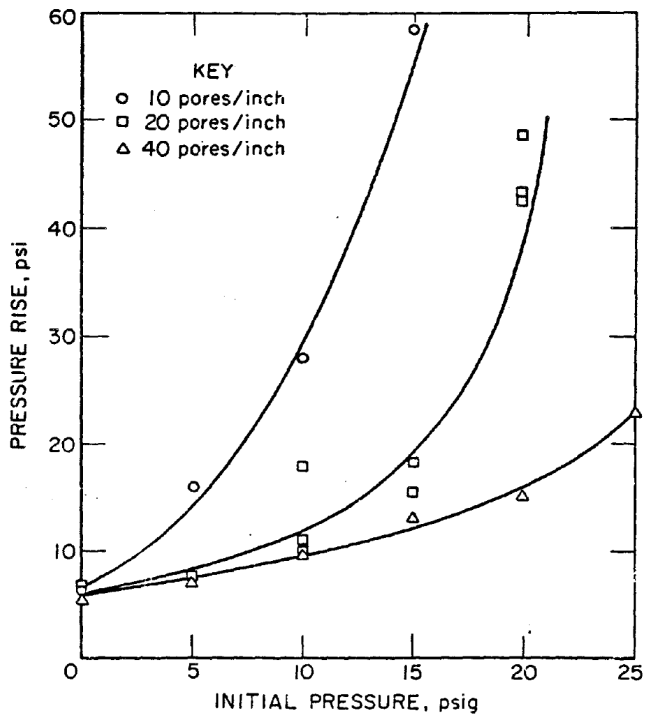
FIGURE 49. Effectiveness of 10, 20, and 40 pore/inch polyurethane foam in quenching ignitions of near-stoichiometric n-pentane-air mixtures (1 atm) in a 1-ft 3 cylindrical vessel. Arrestor length (30-in)/Ignition void (18-in) = 1.67.
