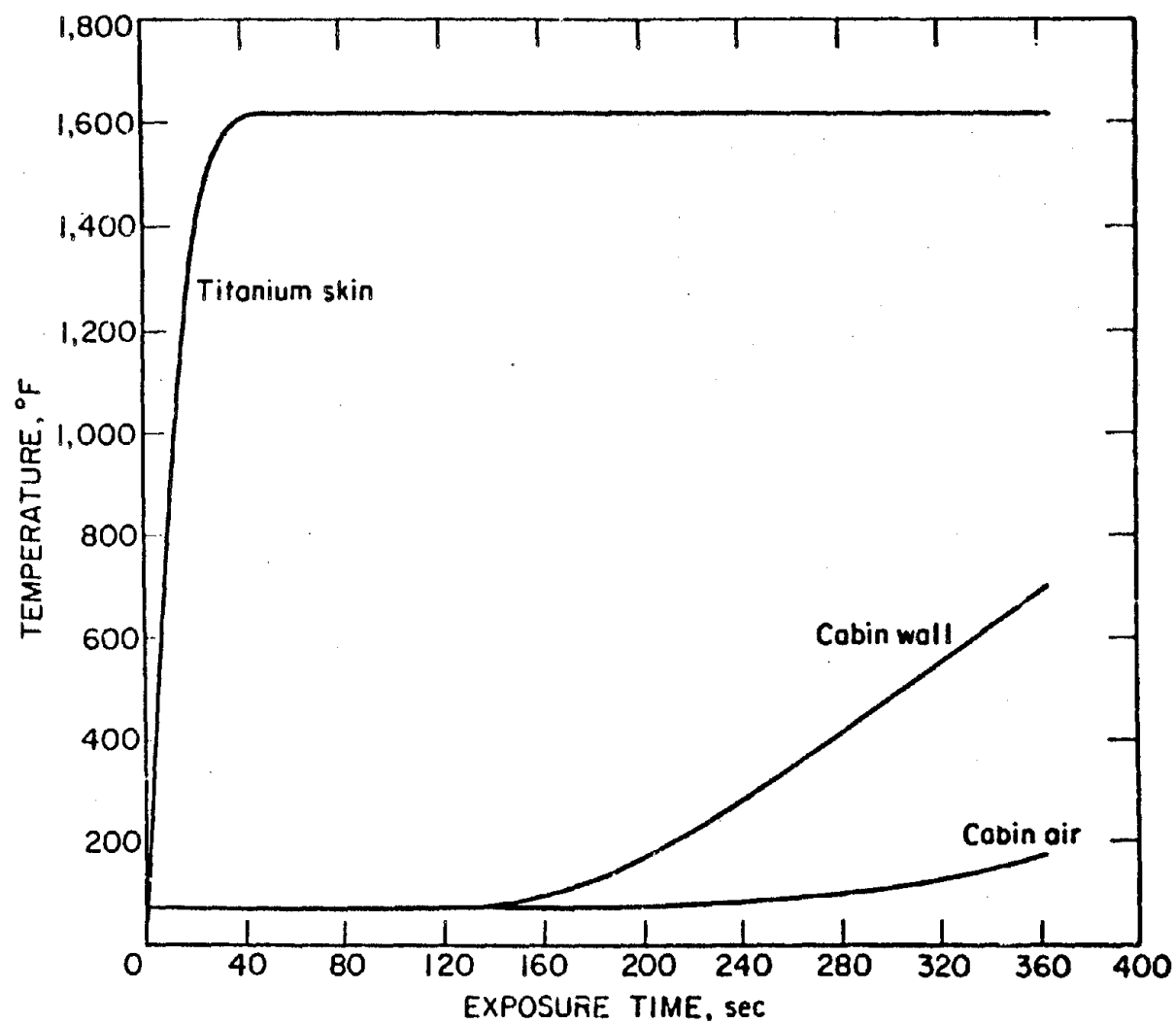
FIGURE 36. Predicted temperature history of a titanium fuselage adjacent to a severe external JP-4 fuel fire.
