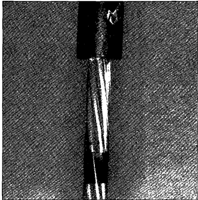
Figure 10.—Closeup of cable bolt strain gauge.
