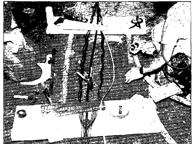
Figure 13.—Strain gauge being placed on combined conventional and birdcage cable.
