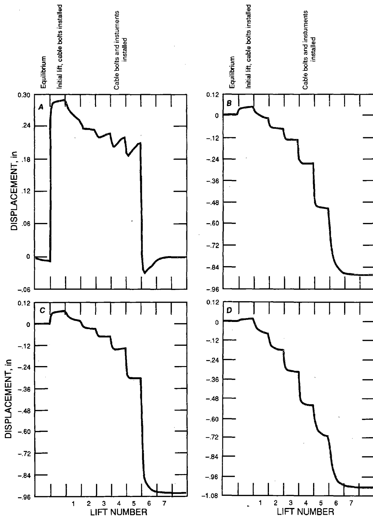
Figure 22.—Displacement curves from numerical analysis of 45-48N stope. A, Anchor 2; B, anchor 4; C, anchor 5; D, anchor 6.
