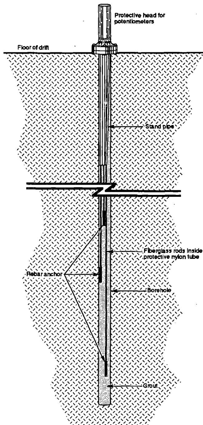
Figure 8.—Profile of extensometer with groutable anchors.
