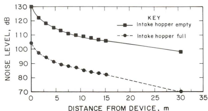
Typical noise levels at site during operation of Pneumatic Pipefeeder and High-Efficiency Ejector.
