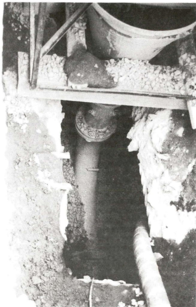
Installation of Pneumatic Pipefeeder on tunnel floor.
