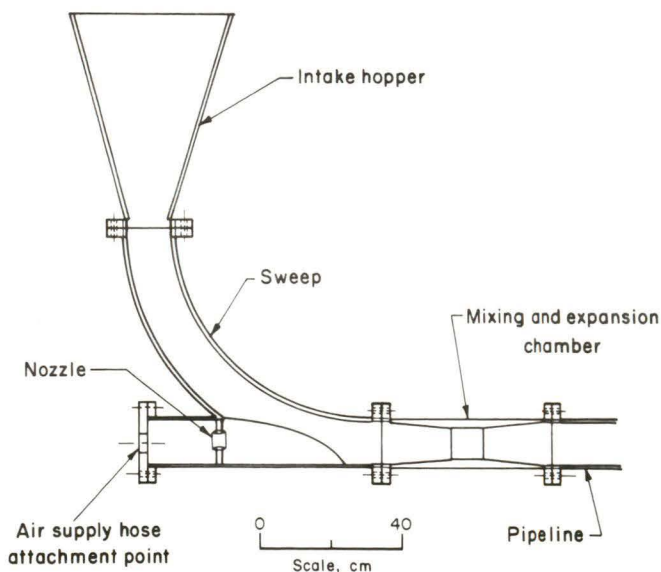
Pneumatic Pipefeeder.
