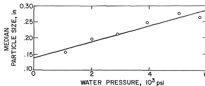
Figure 11.—Median particle size versus water pressure.
