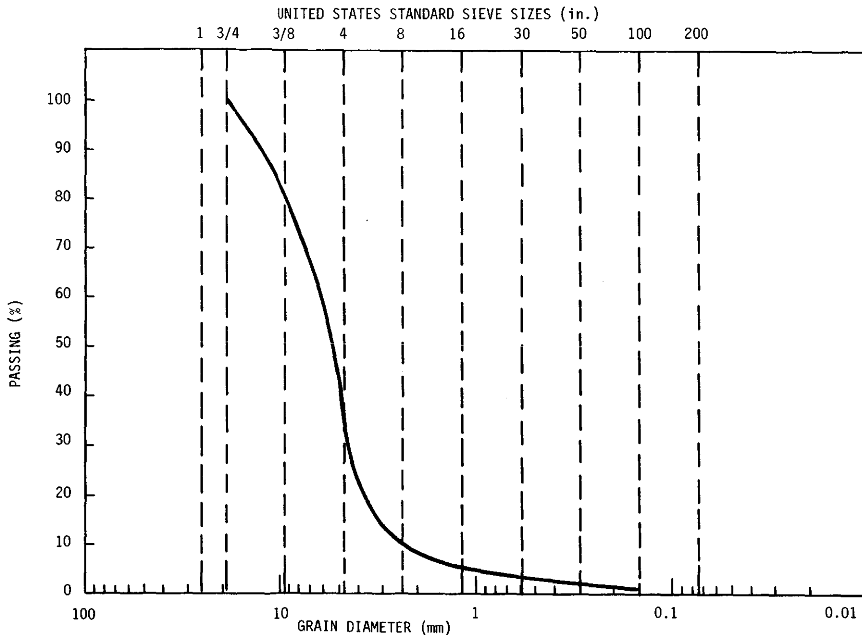
FIGURE 34. - Grain size distribution (sample taken 3/19/80).
