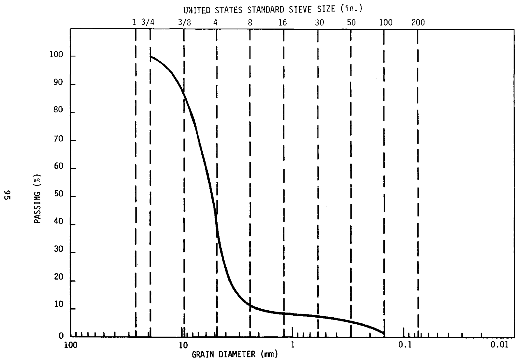
FIGURE 32. - Grain size distribution (sample taken 3/17/80).
