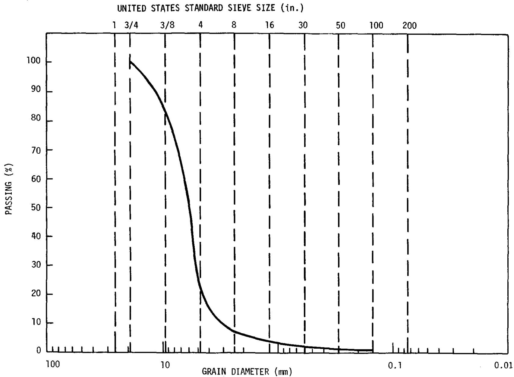
FIGURE 29. - Grain size distribution (sample taken 3/12/80).
