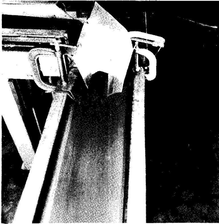
FIGURE 24. - Hopper chute.
