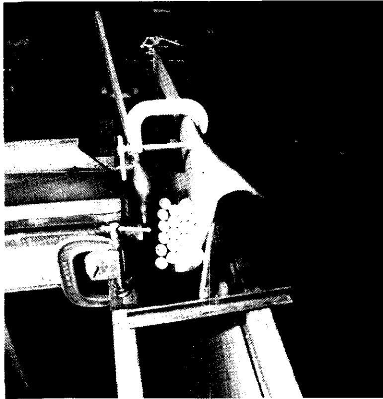
FIGURE 25. - Catenary chute.
