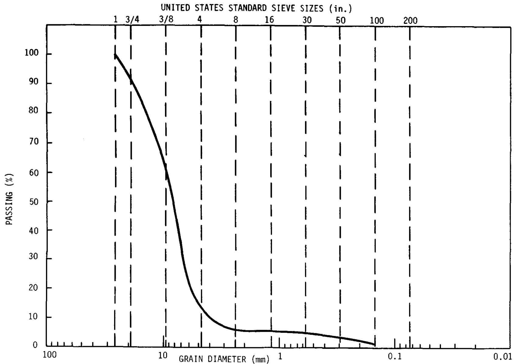
FIGURE 35. - Grain size distribution (sample taken 3/21/80).
