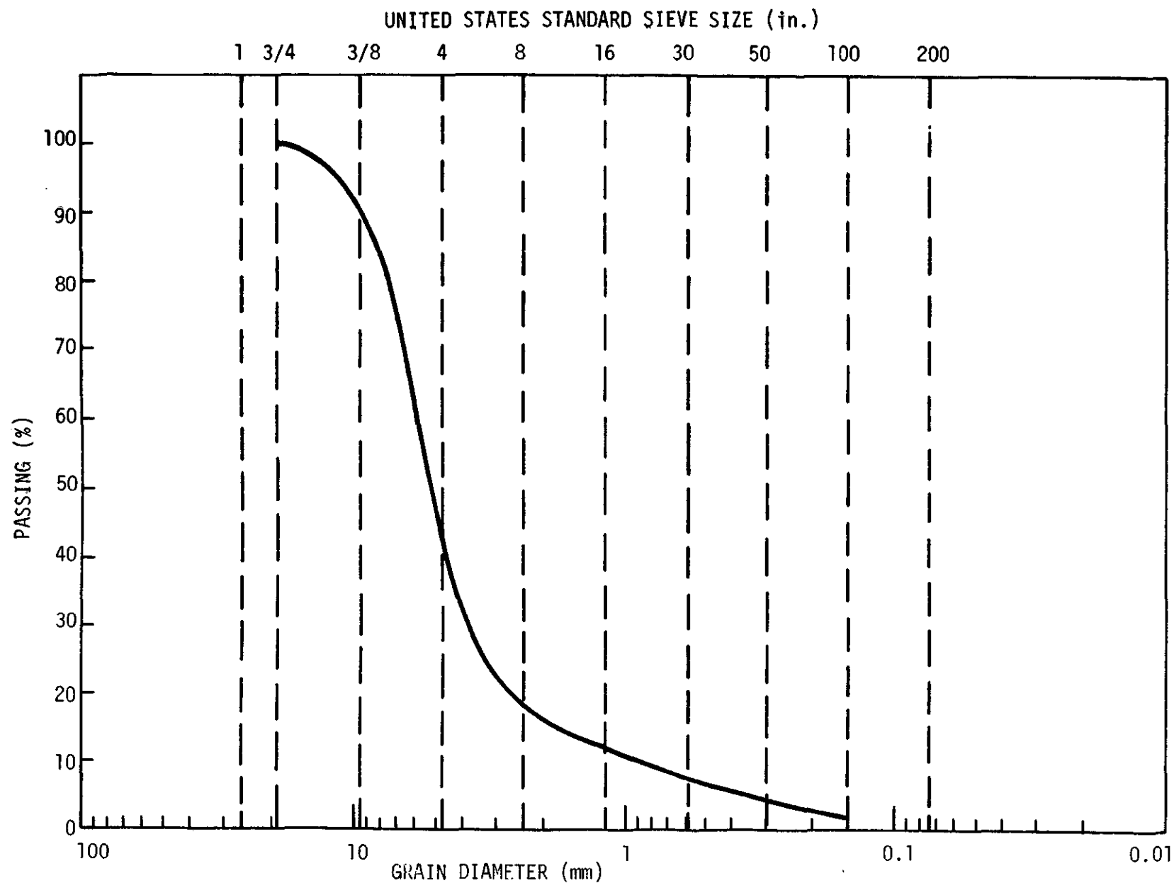
FIGURE 31. - Grain size distribution (sample taken 3/14/80).
