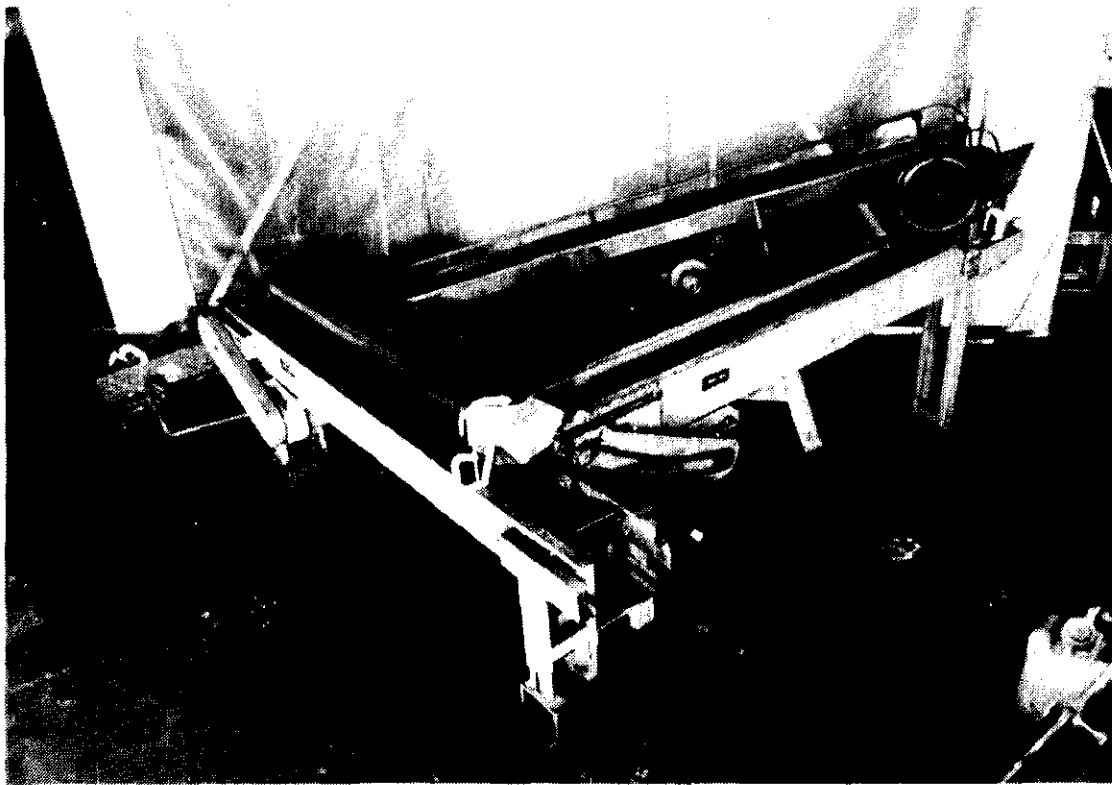
FIGURE 1. - Conveyor arrangement.
