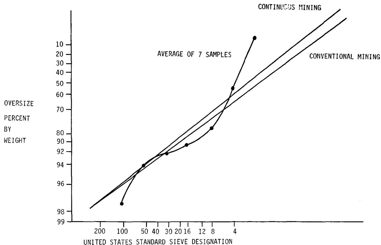
FIGURE 27. - Average size distribution of bituminous coal.
