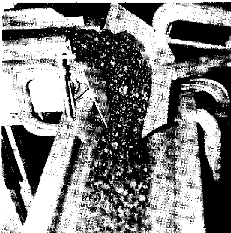
FIGURE 50. - Hopper chute.
