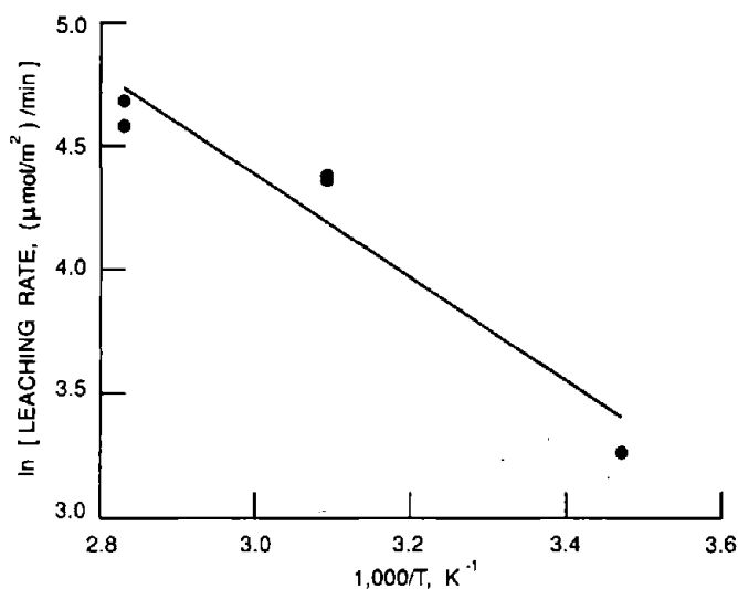
Figure 5.—Arrhenius plot for dissolution of Pd foils in 0.1M NaOH, 1 pct NaCN, at 15°, 50°, and 80° C.
