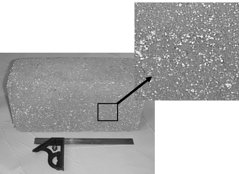
Figure 3. Extruded foam block showing close up of foam pellets (white colored areas) imbedded in a stopping block.
