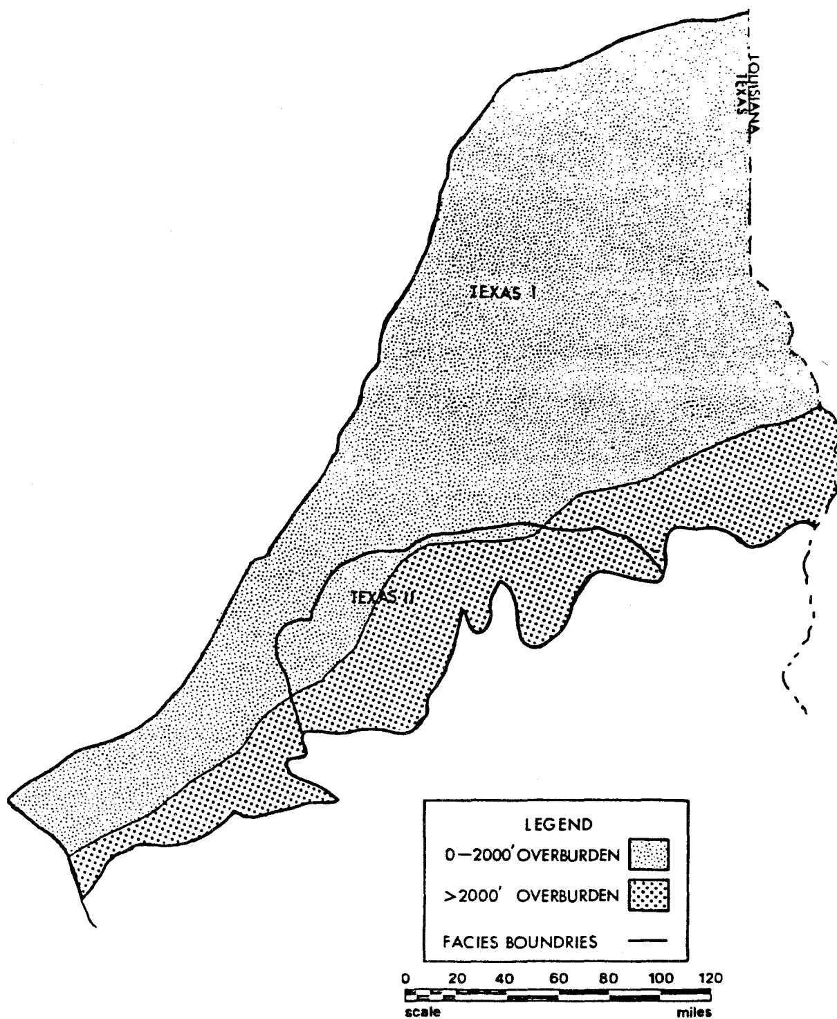
Figure 14. Location of Areas of Resource Estimation for the Texas Portion of the Gulf Coast Lignite Province (Area designated "Texas I" indicates relatively thin lignite; "Texas II" are areas where lignite is relatively thick. See Tables A-22 and A-23 for resources in each area.)
