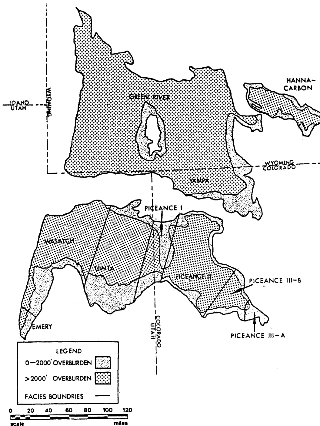
Figure 21. Location of Areas of Resource Estimation for the West Central District of the Rocky Mountain Province. (See Tables A-45 to A-47, A-53, and A-54 for resources in the Emery, Wasatch, Uinta, Green River and Hanna-Carbon areas, respectively. See Table A-48 for total resources in the Piceance area and Tables A-49 and A-51 -- "Piceance I" and "Piceance III-A", respectively -- where the coal-bearing formations are partially eroded. See Tables A-50 and A-52 -- "Piceance II" and "III-B", respectively -- for areas where the full sequence of the coal bearing formations are present, and Table A-44 for total resources for the district.)
