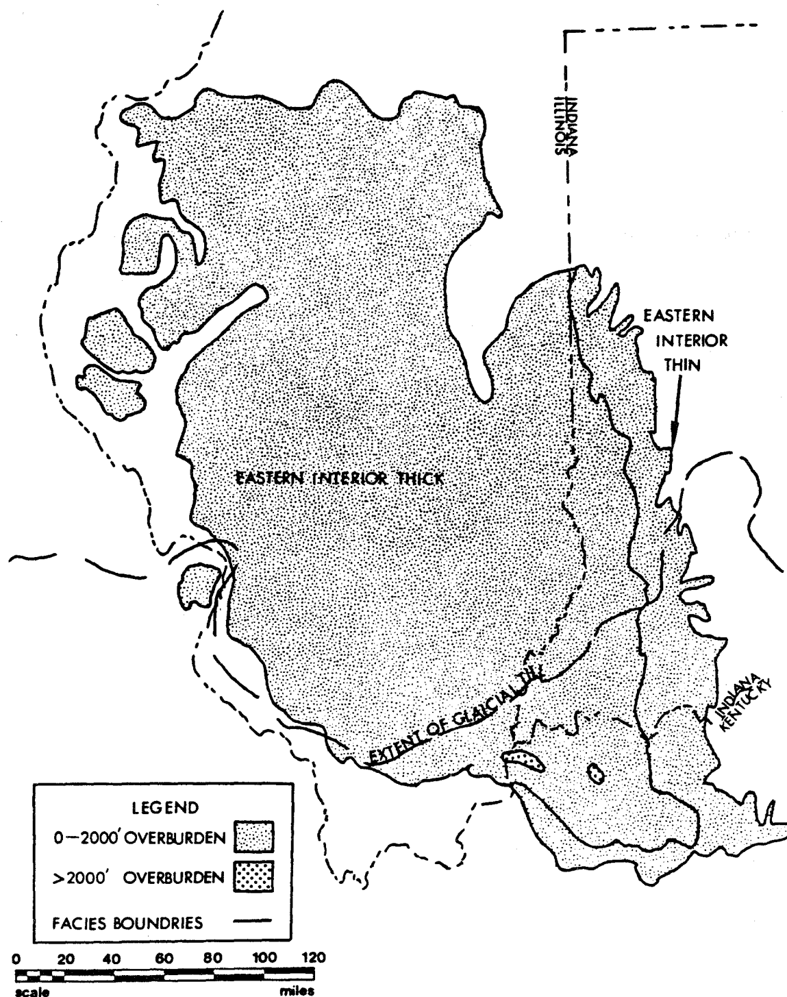
Figure 10. Location of Areas of Coal Resource Estimation in the Eastern Interior Basin in the Carboniferous Interior Province (Area designated "Eastern Interior Thick" consists mainly of the major coal bearing formations. Area designated "Eastern Interior Thin" is mainly thin older seams that have no importance elsewhere in the basin. See Tables A-19 and A-20 for each area and Table A-18 for total resources.)
