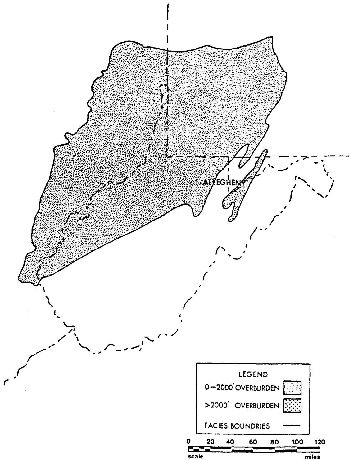
Figure 5. Location of Areas of Coal Resource Estimation for the Allegheny Formation in the Dunkard Basin of the Appalachian Plateau Province. (See Table A-5 for resources.)
