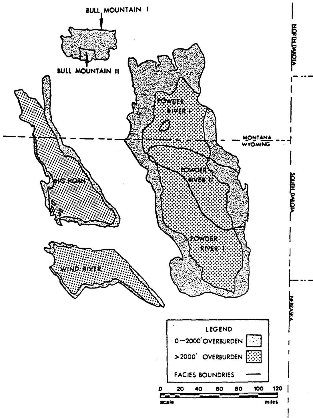
Figure 22. Location of Areas of Resource Estimation for the Northern District of the Rocky Mountain Province (See Tables A-56 and A-57 for resources in the Wind River and Big Horn areas and Table A-58 for total resources of the Bull Mountain area. Tables A-59 and A-60 show, respectively, resources for "Bull Mountain I" where the coal-bearing formations are partially eroded and "Bull Mountain II" where the full coal-bearing sequence is present. Table A-61 shows total resources for the Powder River area, and Tables A-62 and A-63 show, respectively, resources for "Powder River II" where the coal is thicker and the full sequence is present. Table A-55 shows total resources for the district.)
