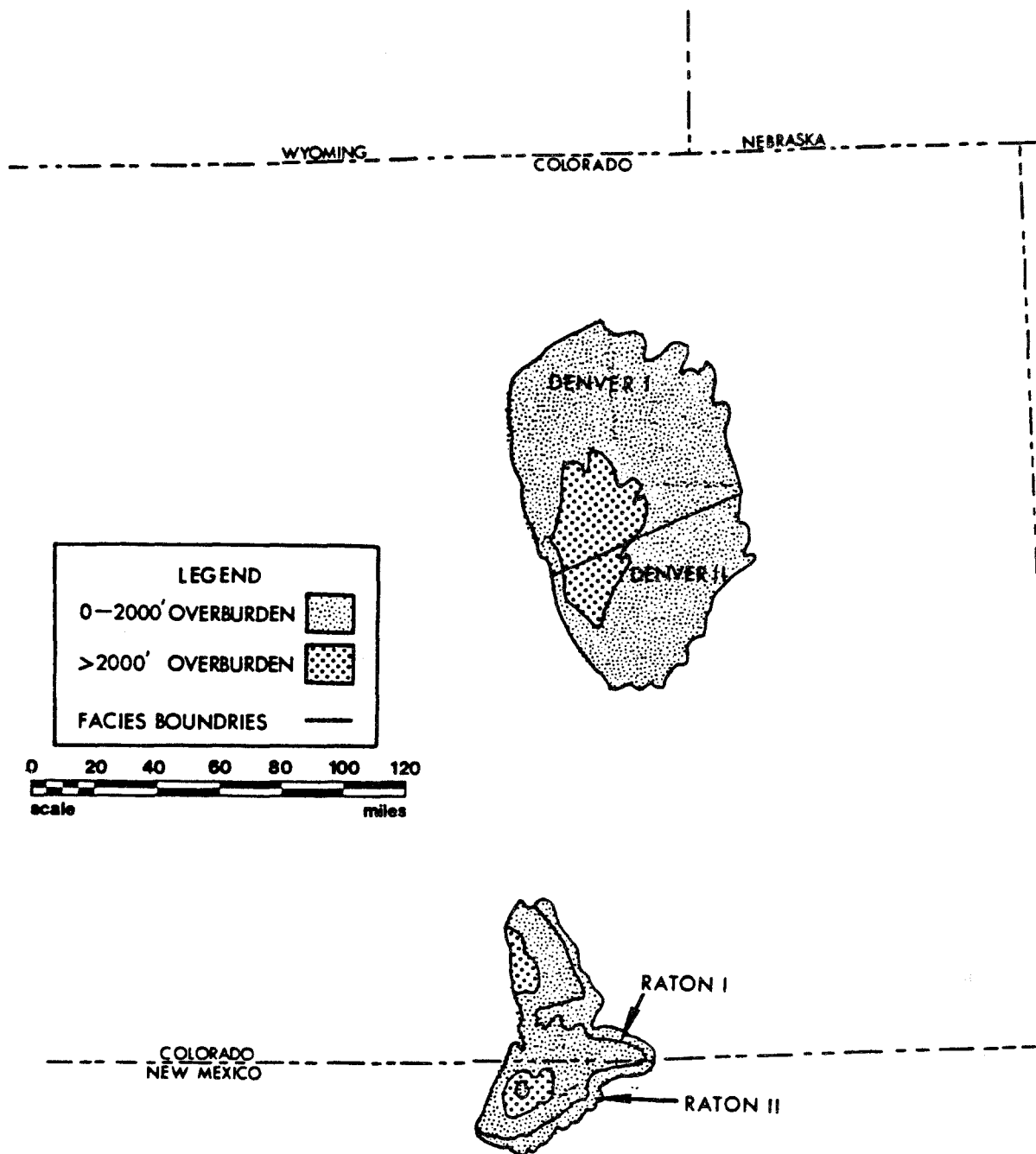
Figure 23. Location of Areas of Resource Estimation for the Front Range District of the Rocky Mountain Province (See Table A-65 for total resources in the Denver Basin area and Tables A-66 and A-67 for areas "Denver I" where the rank of coal is subbituminous, and "Denver II" where the rank is lignite. See Table A-68 for total resources for the Raton Area, and Tables A-69 and A-70 for areas "Raton I" where the coal seams are gently dipping and where a great percentage of tonnage occurs in seams 15 ft - 42 in. and "Raton II" in which the coal is gently dipping and has an overburden of less than 500 ft. Table A-64 shows resources for the district.)
