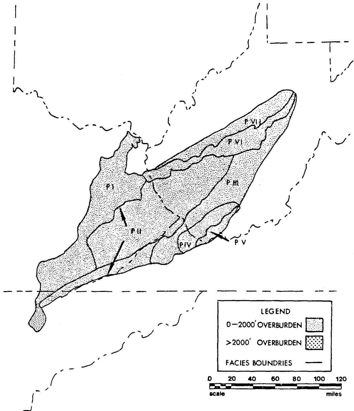
Figure 6. Location of Areas of Coal Resource Estimation for the Pocahontas Basin in the Appalachian Plateau Province. (Areas "P-I" through "P-VII" represent outcrop and subcrop areas of different coal formations in the Pocahontas Basin. See text for description of coals in each area and Tables A-6 through A-13 for resources.)
