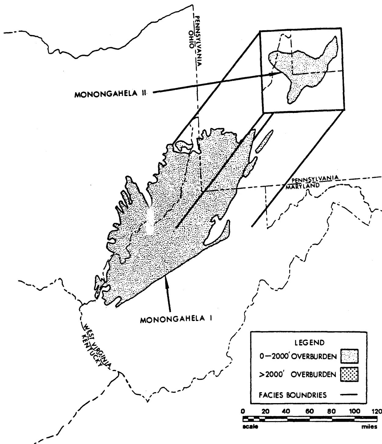
Figure 4. Location of Areas of Coal Resource Estimation for the Monongahela Formation in the Dunkard Basin of the Appalachian Plateau Province (Larger area -- "Monongahela I" -- represents the area where the formation is partially eroded; smaller area -- "Monongahela II" -- represents the area where the full thickness of the formation is present. See Tables A-3 and A-4 for resources in each area and Table A-2 for total resources.)
