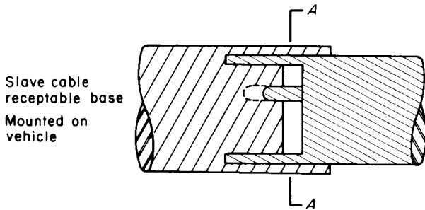
FIGURE 2. - Offcenter slave cable connector.
