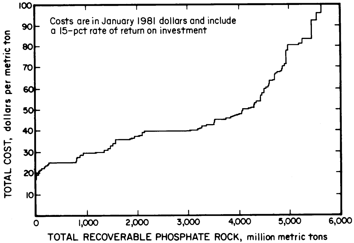
FIGURE 14. - Phosphate rock potentially recoverable from all domestic deposits.
