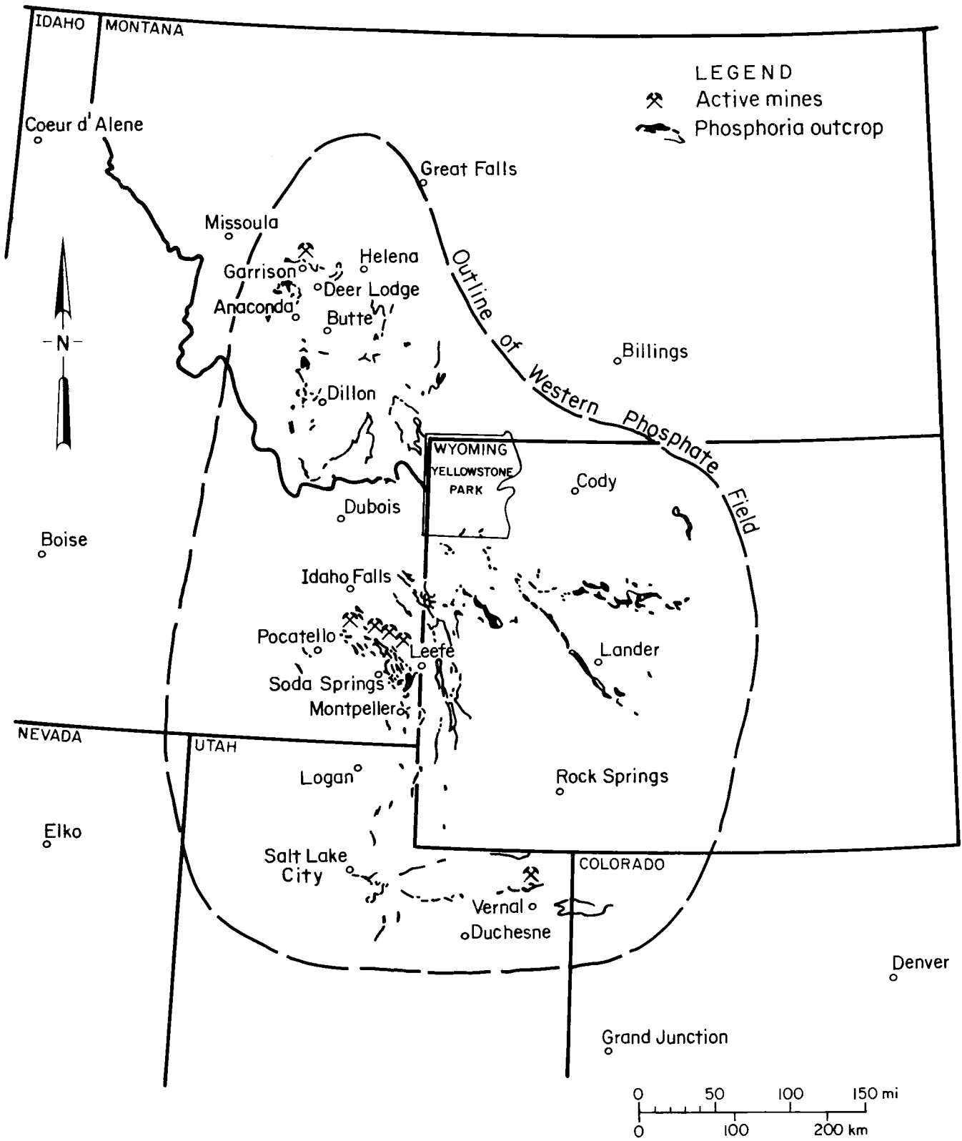
FIGURE 8. - Location of Western U.S. phosphate deposits. (Modified from reference 10.)
