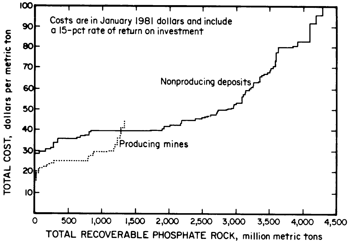
FIGURE 18. - Phosphate rock potentially recoverable from producing mines and nonproducing deposits.
