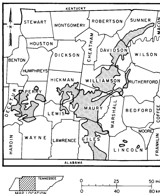
FIGURE 7. - Location of Tennessee phosphate deposits.
