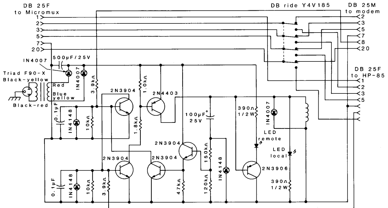
FIGURE B-2. - Arbiter schematic.
