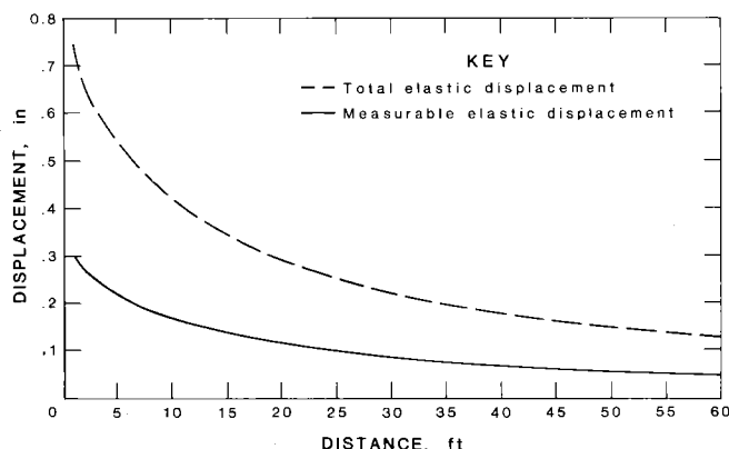
FIGURE 1. - Total and measurable rock displacement at the 2,414 level.
