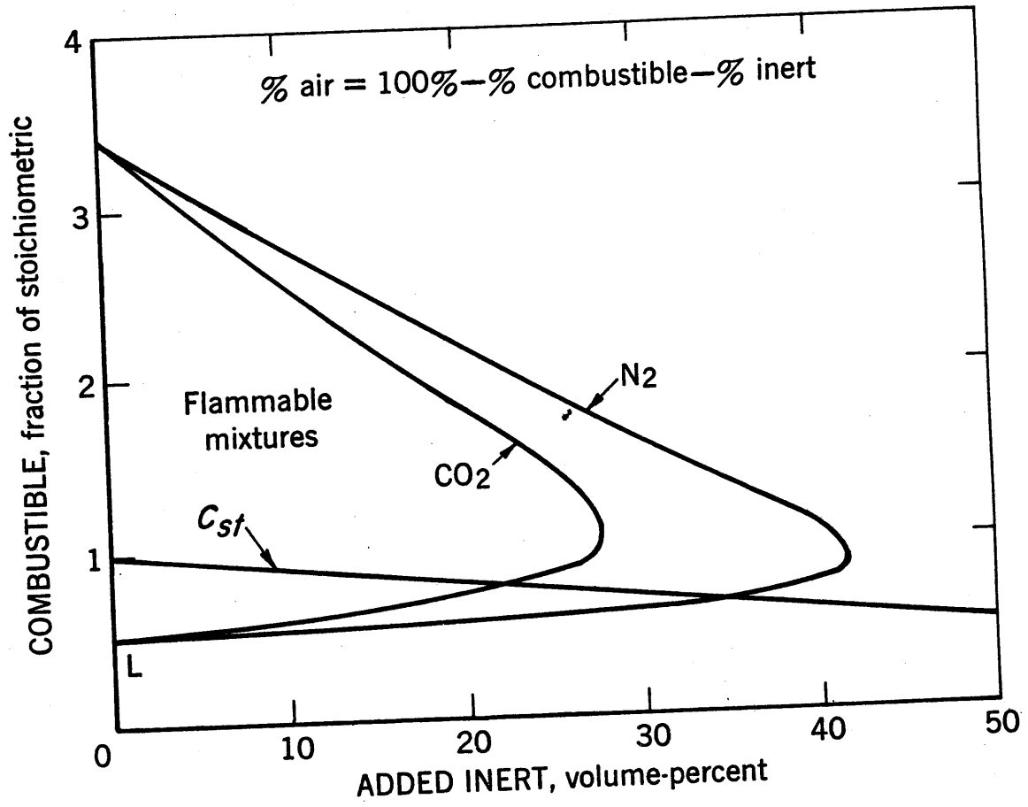
FIGURE 35.—Approximate Limits of Flammability of Higher Paraffin Hydrocarbons ( \text{C}_n\text{H}_{2n+2} , n \geq 5 ) in Carbon Dioxide-Air and Nitrogen-Air Mixtures at 25^\circ \text{C} and Atmospheric Pressure.
