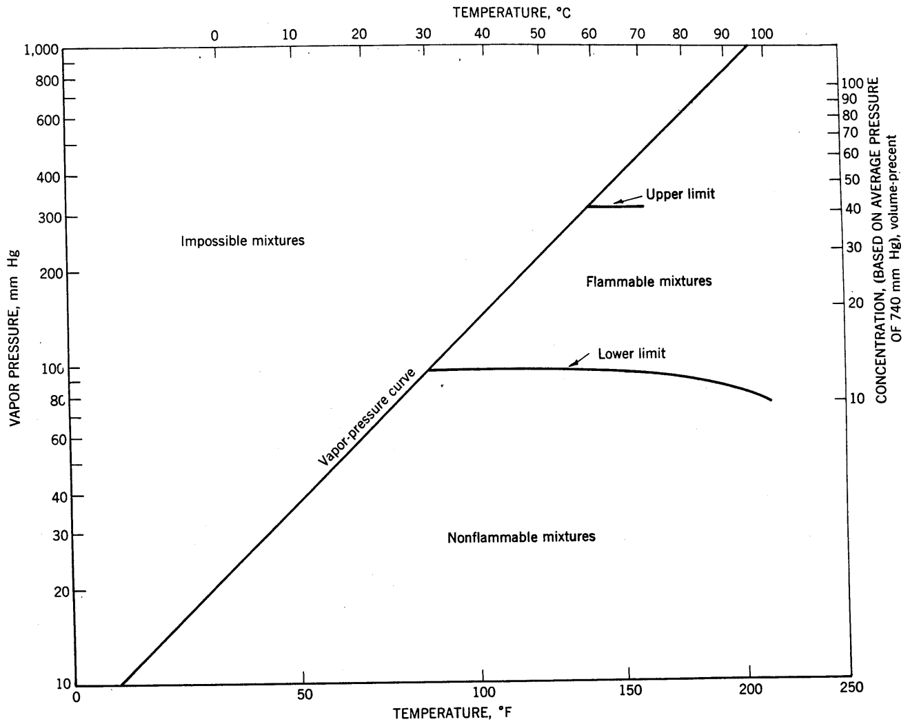
FIGURE 131.—Flammability of Trichloroethylene-Air Mixtures.
