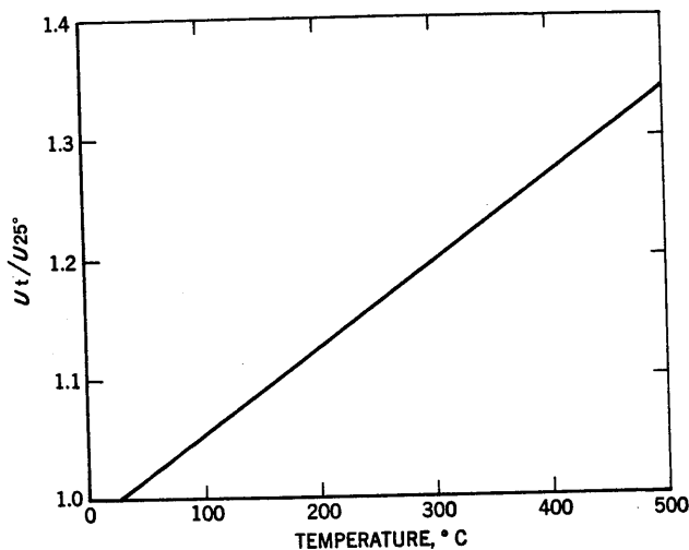
FIGURE 24.—Effect of Temperature on U_1/U_{25} Ratio of Paraffin Hydrocarbons in Air at Atmospheric Pressure in the Absence of Cool Flames.
