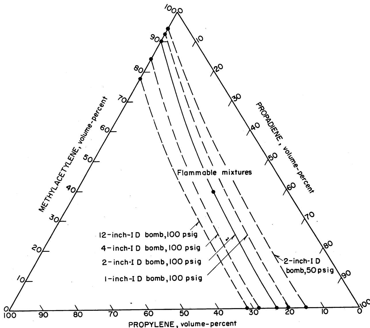
FIGURE 62.—Range of Flammable Mixtures for Methyacetylene-Propadiene-Propylene System at 120° C and at 50 and 100 Psig.
