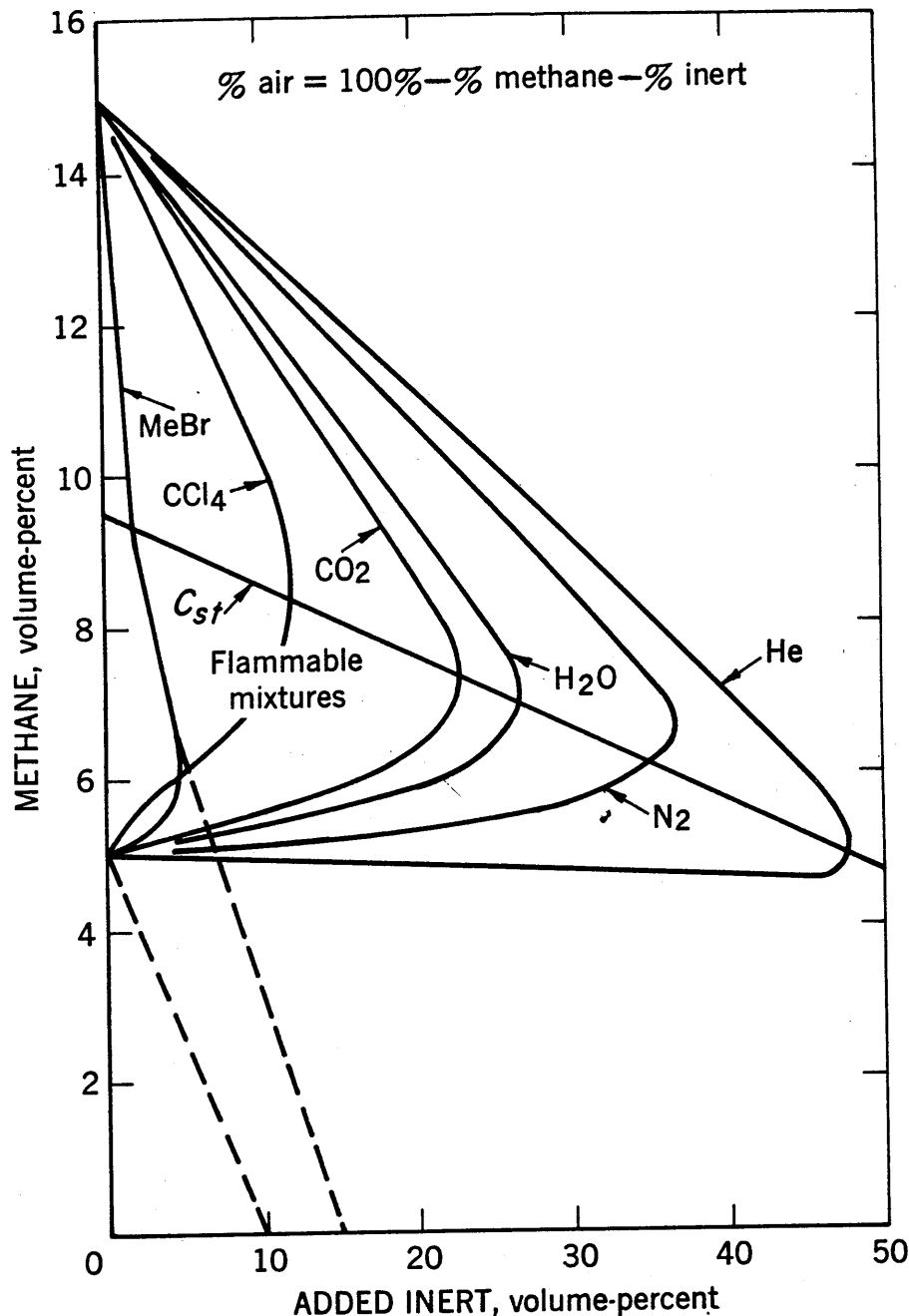
FIGURE 28.—Limits of Flammability of Various Methane-Inert Gas-Air Mixtures at 25° C and Atmospheric Pressure.
