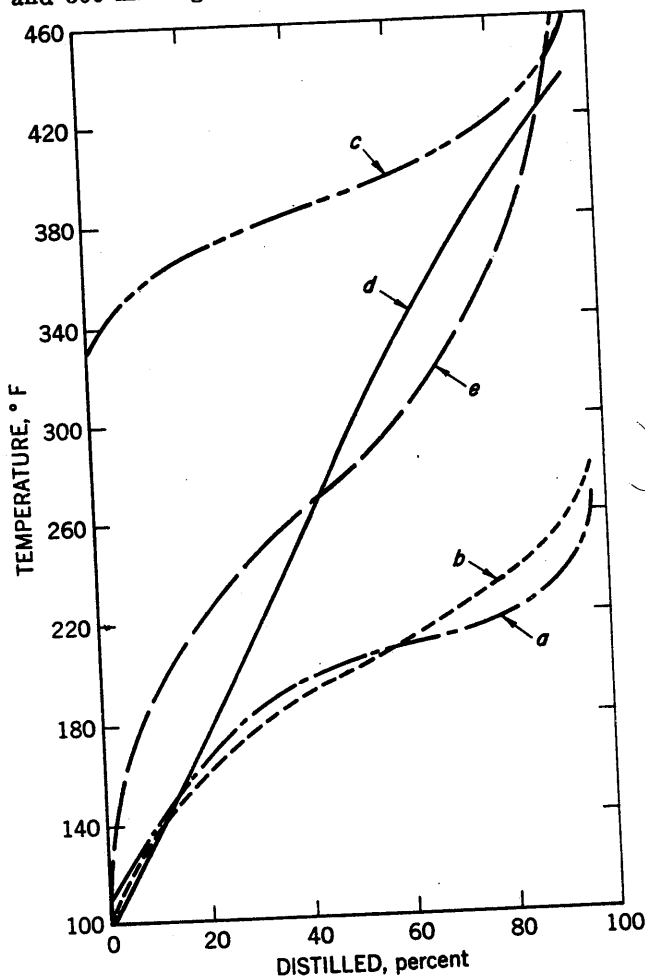
FIGURE 108.—ASTM Distillation Curves for, A, Aviation Gasoline, Grade 100/130; B, Aviation Gasoline, Grade 115/145; C, Aviation Jet Fuel, Grade JP-1; D, Aviation Jet Fuel, Grade JP-3; and E, Aviation Jet Fuel, Grade JP-4.
