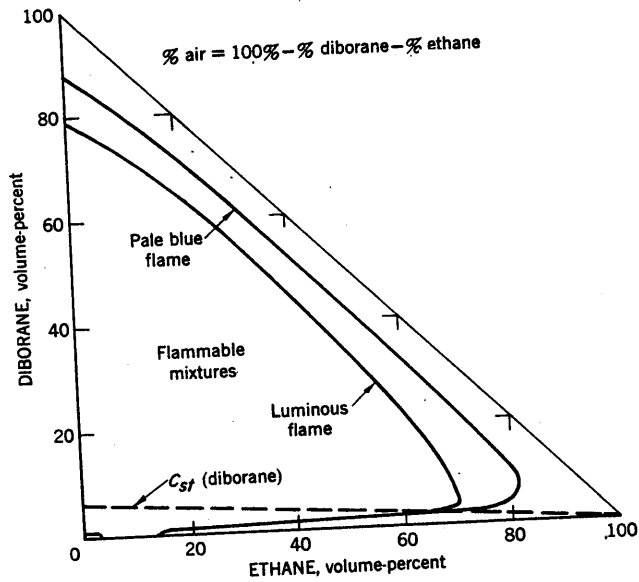
FIGURE 107.—Limits of Flammability of Diborane-Ethane-Air Mixtures at Laboratory Temperatures and 300 mm Hg Initial Pressure.
