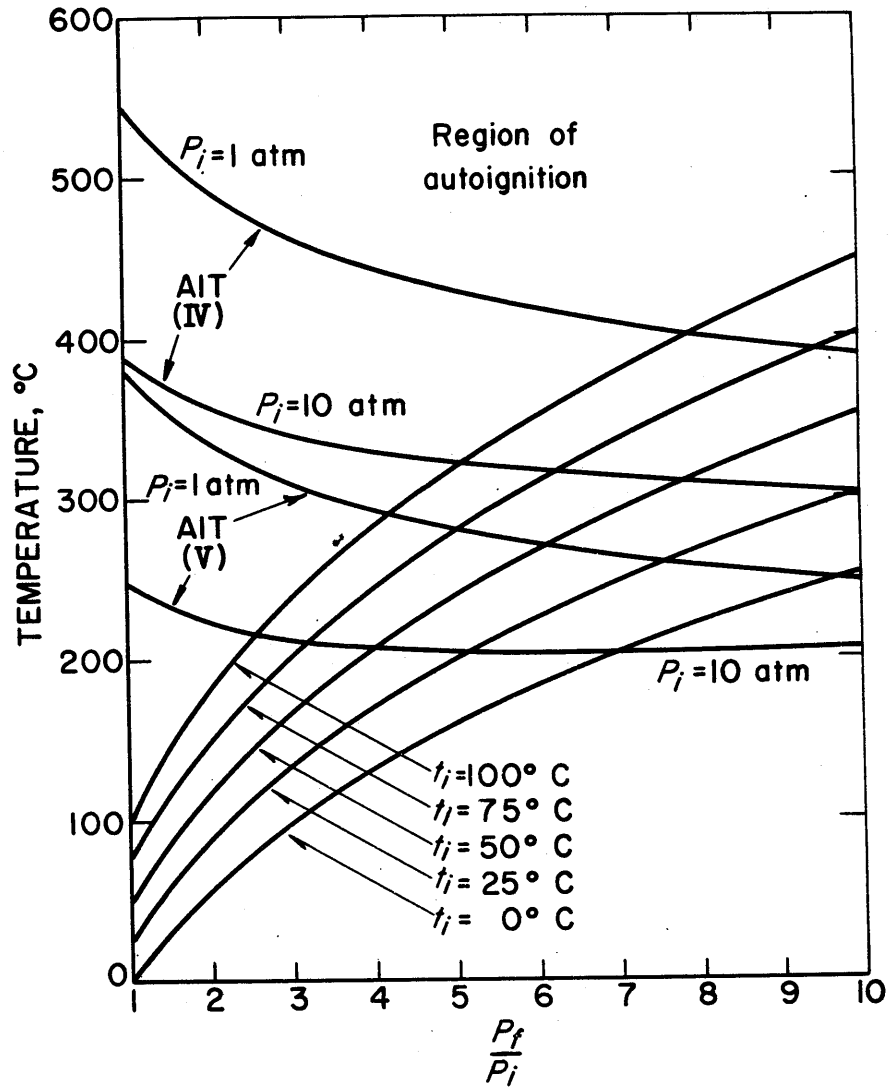
FIGURE 125.—Variation In Air Temperature With P_f/P_i in an Adiabatic Compression Process for Five Initial Air Temperatures (0°, 25°, 50°, 75°, and 100° C). Regions of autoignition for lubricants IV and V at P_f/P_i Between 1 and 10 Atmosphere and P_i of Between 1 and 10 Atmospheres.
