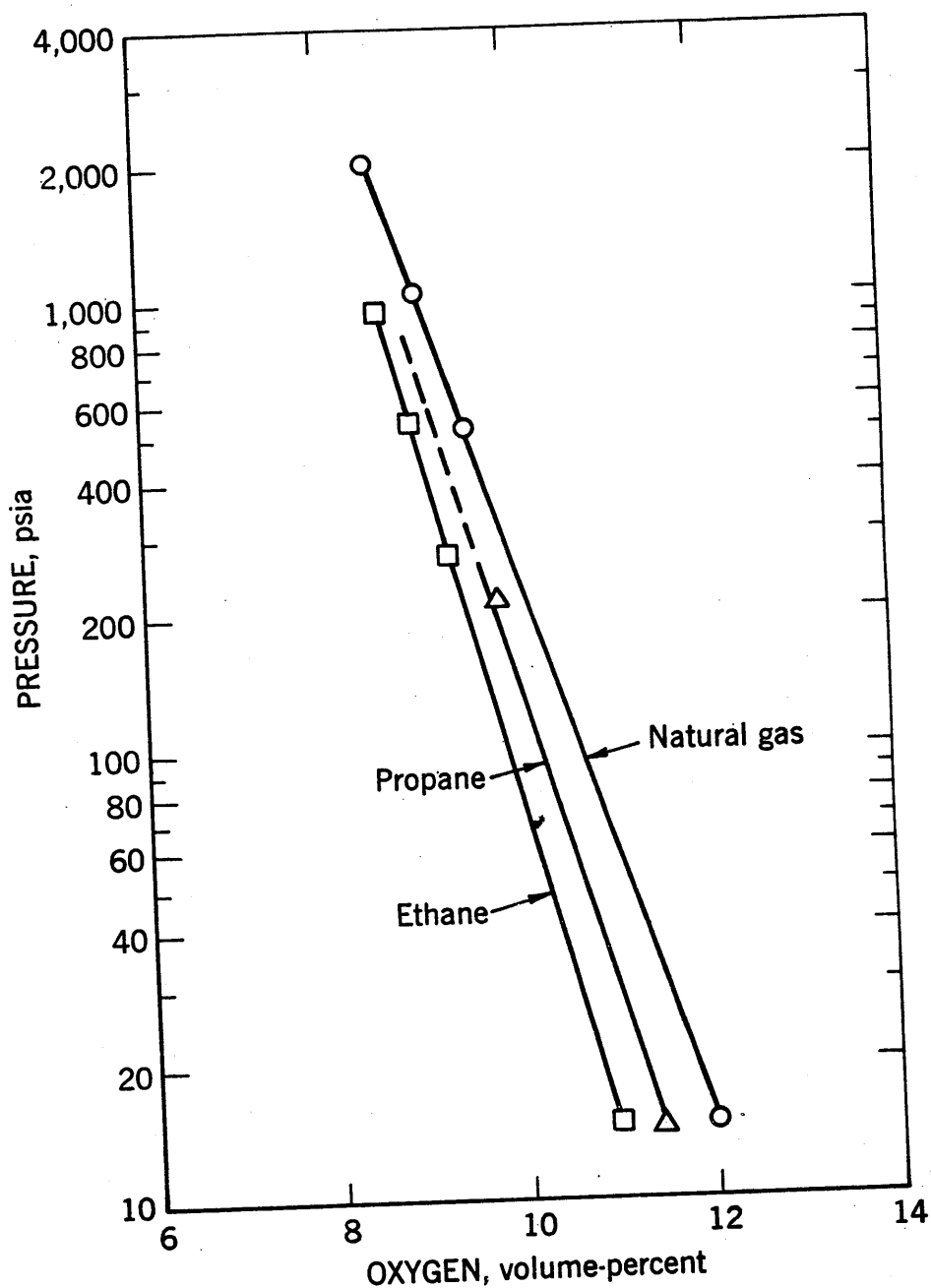
FIGURE 41.—Effect of Pressure on Minimum Oxygen Requirements for Flame Propagation Through Natural Gas-Nitrogen-Air, Ethane-Nitrogen-Air, and Propane-Nitrogen-Air Mixtures at 26° C.
