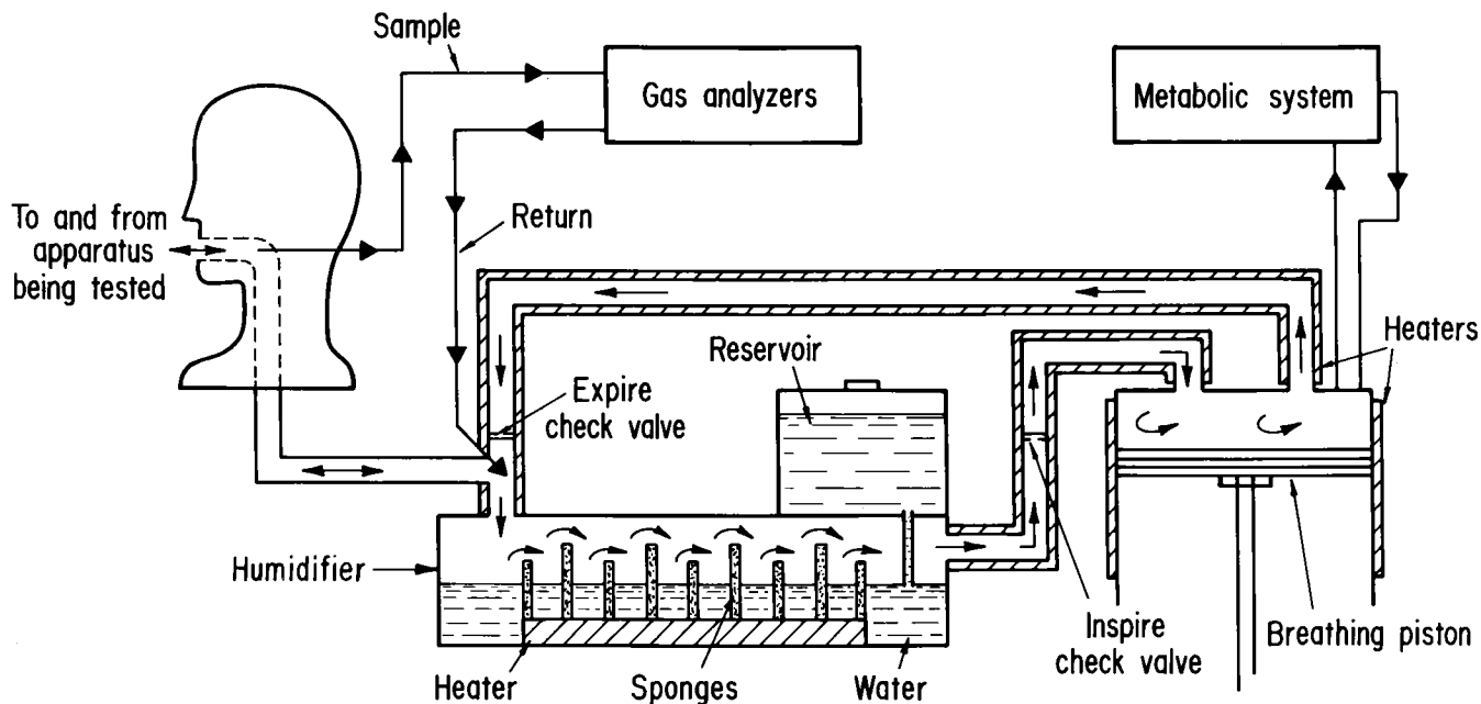
FIGURE 4.—IBM temperature and humidity system schematic.
