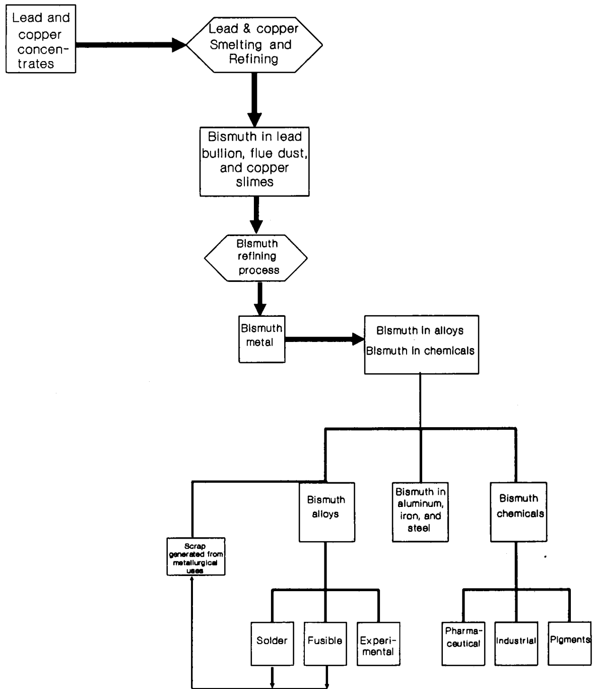
Figure 4.—Bismuth processing cycle.
