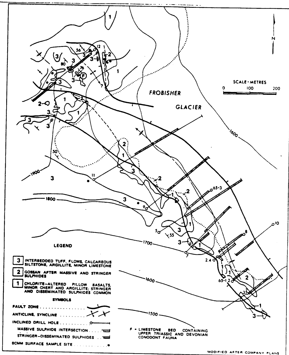
FIGURE 4. - Geology and drill hold locations, Windy Craggy deposit. A copy of figure 54 Macintyre (9).
