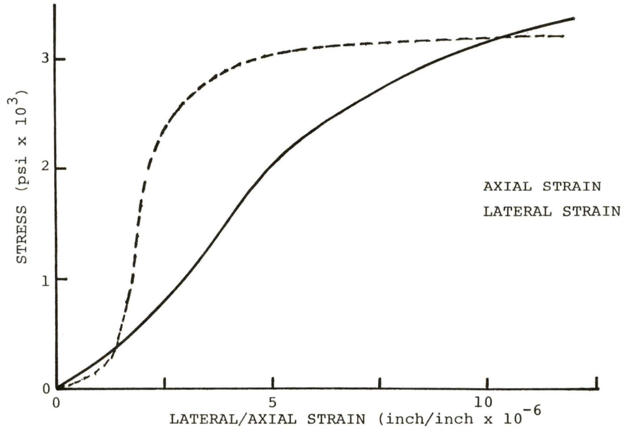
FIGURE C-1. Typical axial stress-axial strain and axial stress-lateral strain curves for a discontinuous rock mass.
