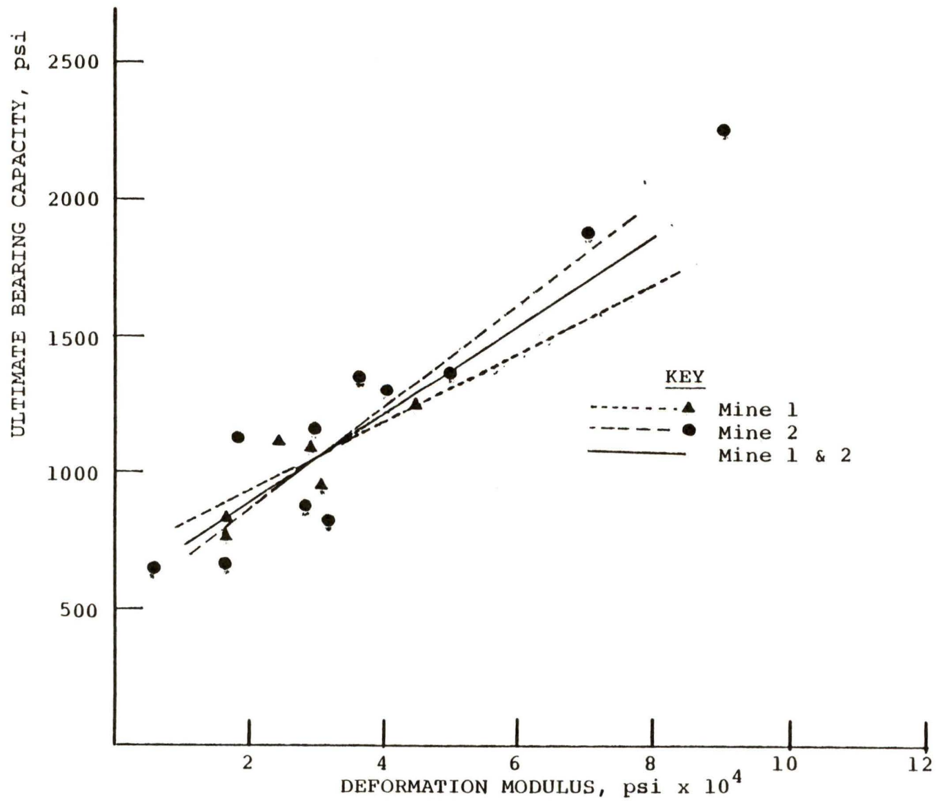
FIGURE 4.8 Correlation of deformation modulus with ultimate bearing capacity.
