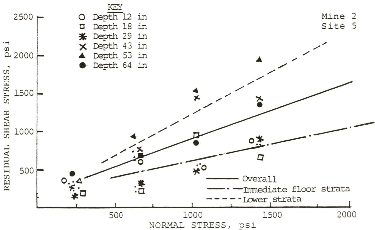
FIGURE 4-12 Shear strength - normal stress relationships for immediate floor strata.
