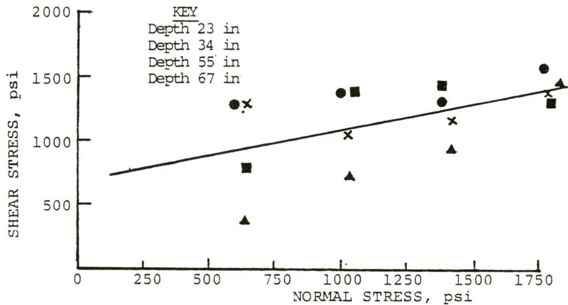
FIGURE 4.14 Shear strength - normal stress relationship for immediate roof strata - Mine 1.
