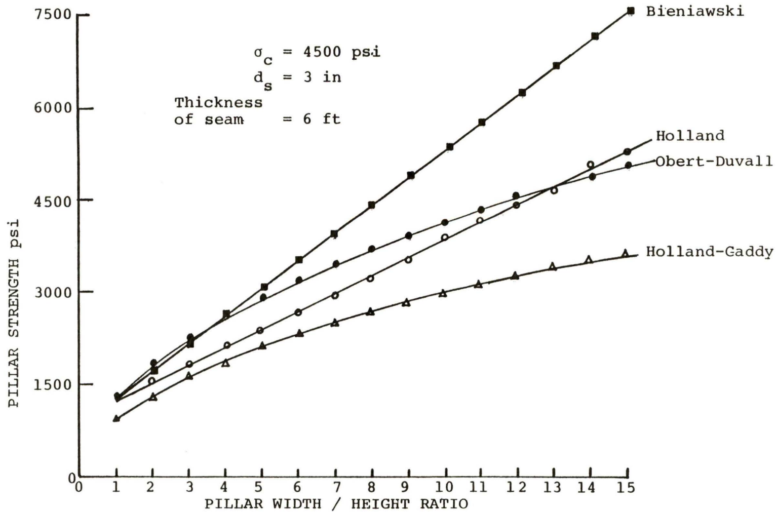
FIGURE 4.1 A comparison of commonly utilized pillar strength formulas.
