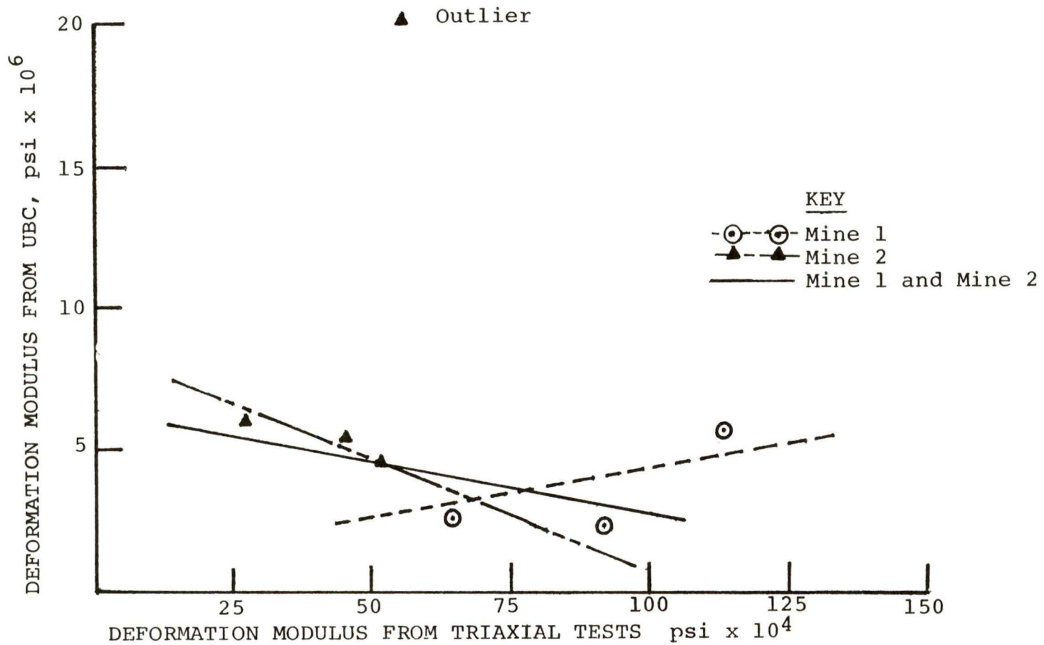
FIGURE 4.21 Correlation of deformation modulus as obtained from triaxial test with that obtained from bearing capacity tests.
