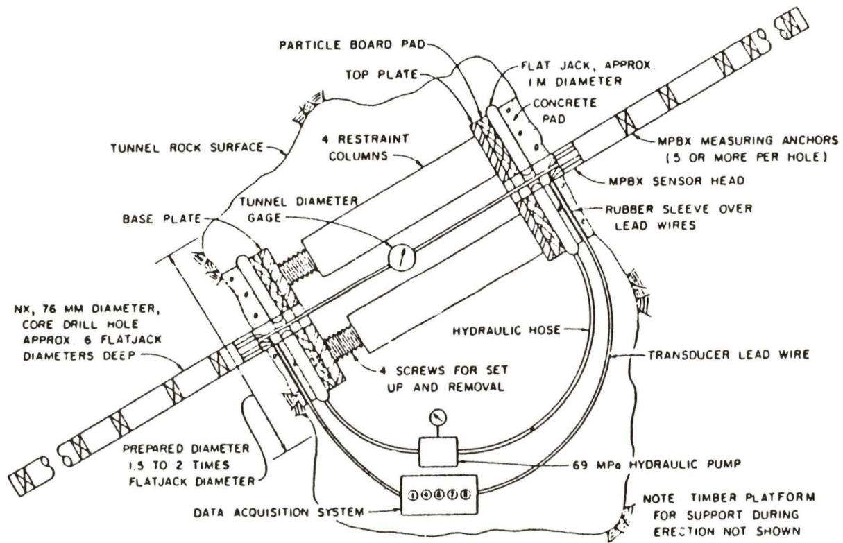
Figure 2.12 In-situ Deformability Measurement Technique (ISRM, 1978)
