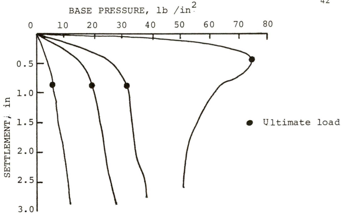
FIGURE 2.9 Vesic's criterion for determination of ultimate bearing capacity
