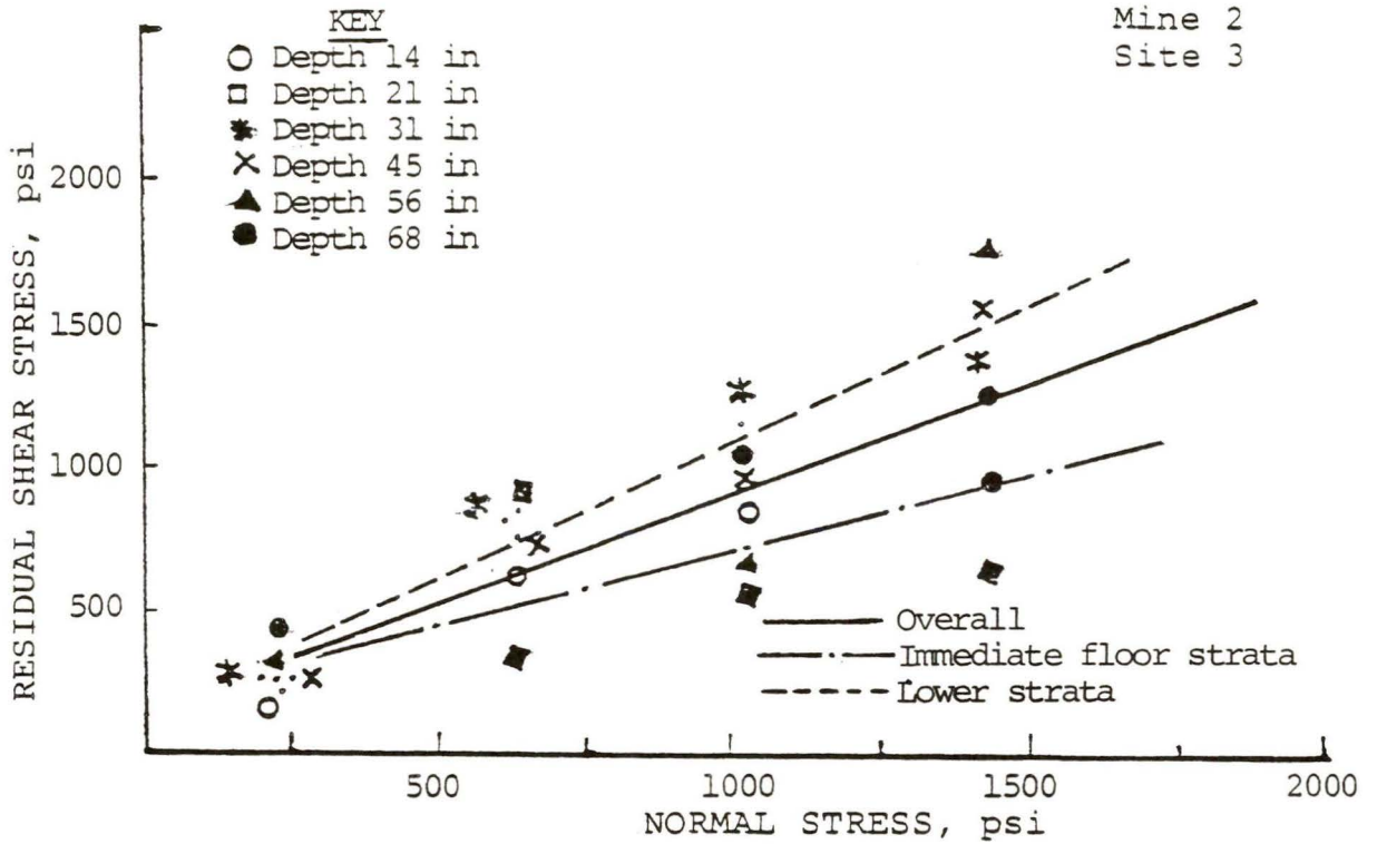
FIGURE B-9 Shear strength - normal stress relationships for immediate floor strata.
