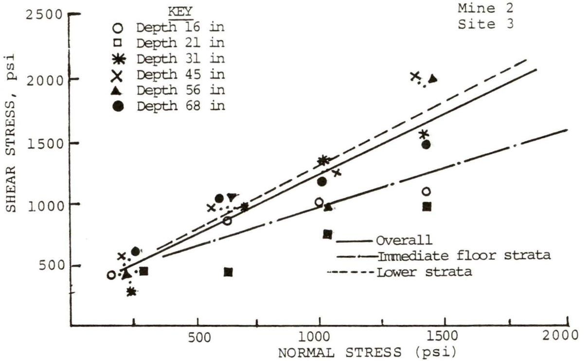
FIGURE B-5 Shear strength - normal stress relationships for immediate floor strata.
