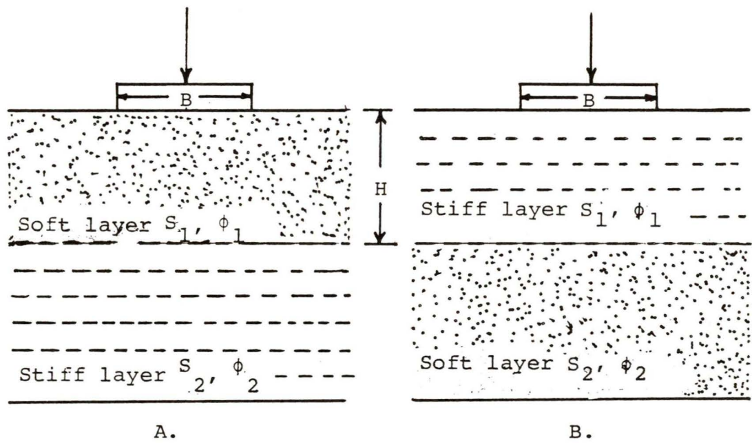
FIGURE 2.5 Bearing capacity analysis for two layered soil media (after Brown and Meyerhof, 1969).
