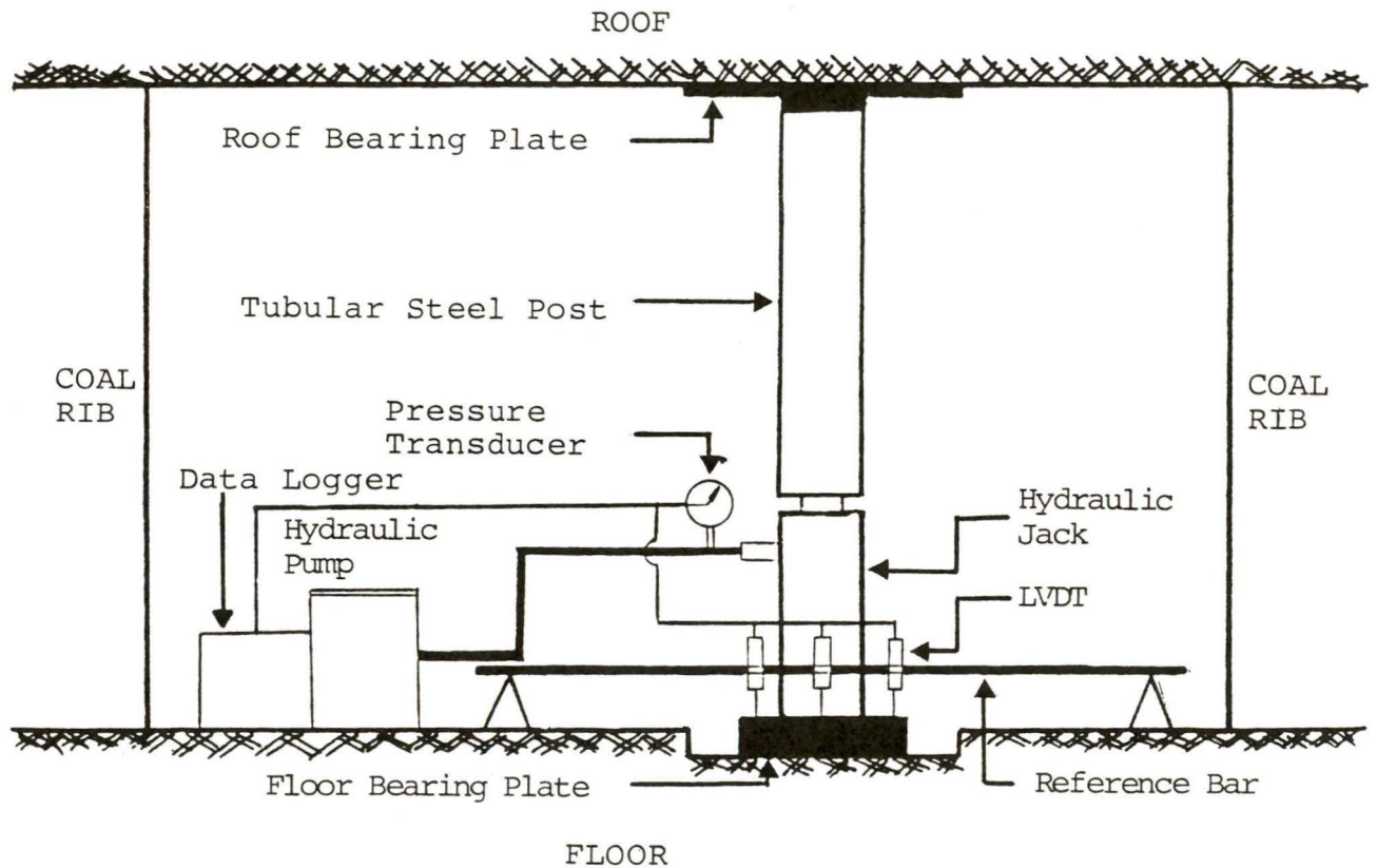
Figure 3.1. Bearing Capacity Measurement Setup.
