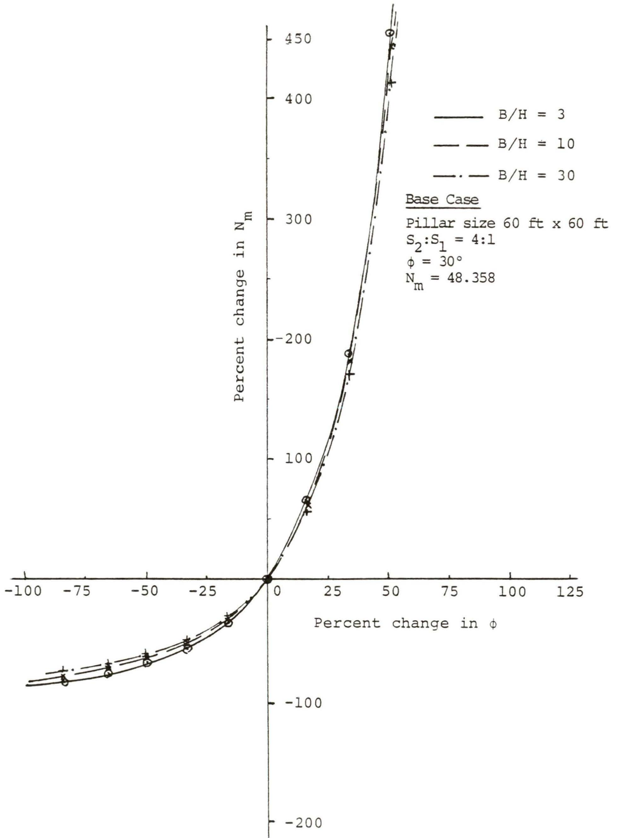
FIGURE 2.6 Sensitivity analysis of N_m with \phi (Chugh and Chandrashekhar, 1986).
