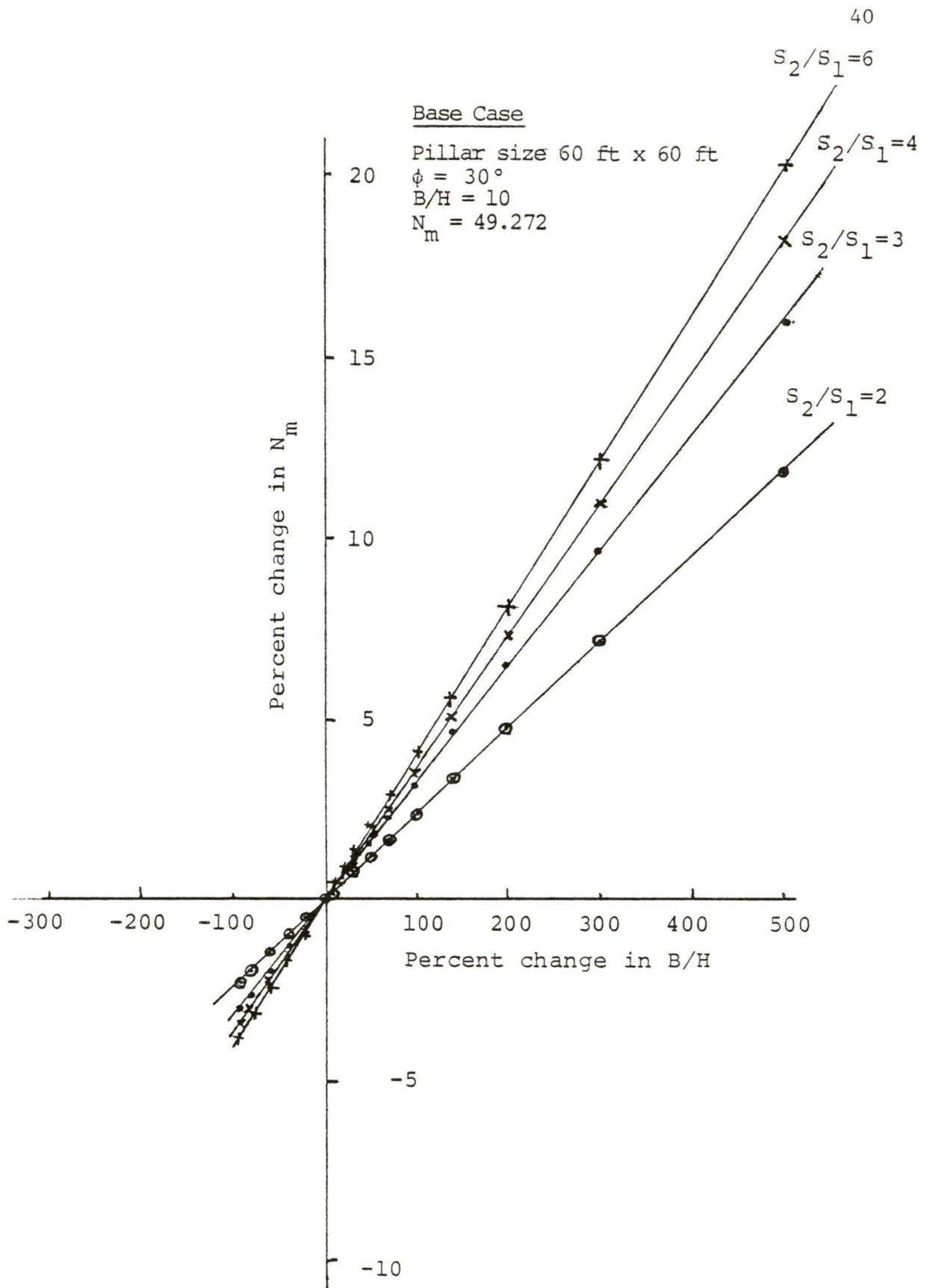
FIGURE 2.8 Sensitivity analysis of N_m with B/H (Chugh and Chandrashekhar, 1986).
