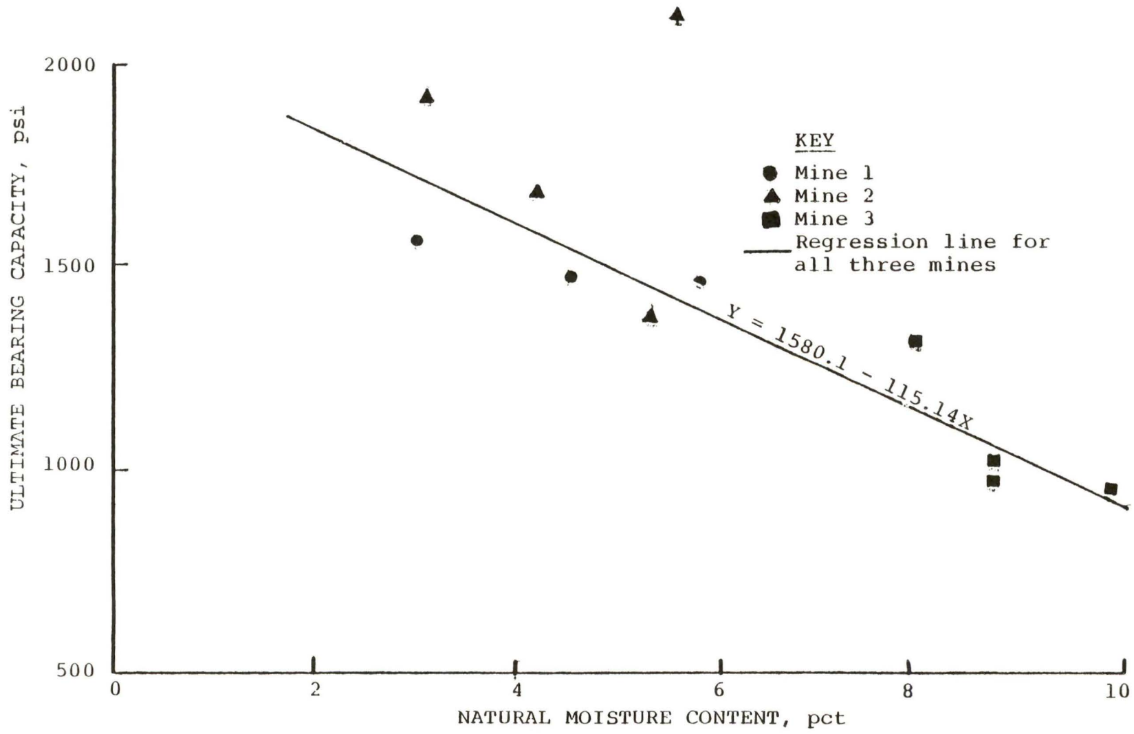
FIGURE 4.20 Correlation of ultimate bearing capacity with natural moisture content of immediate floor strata in 0-12 in range.
