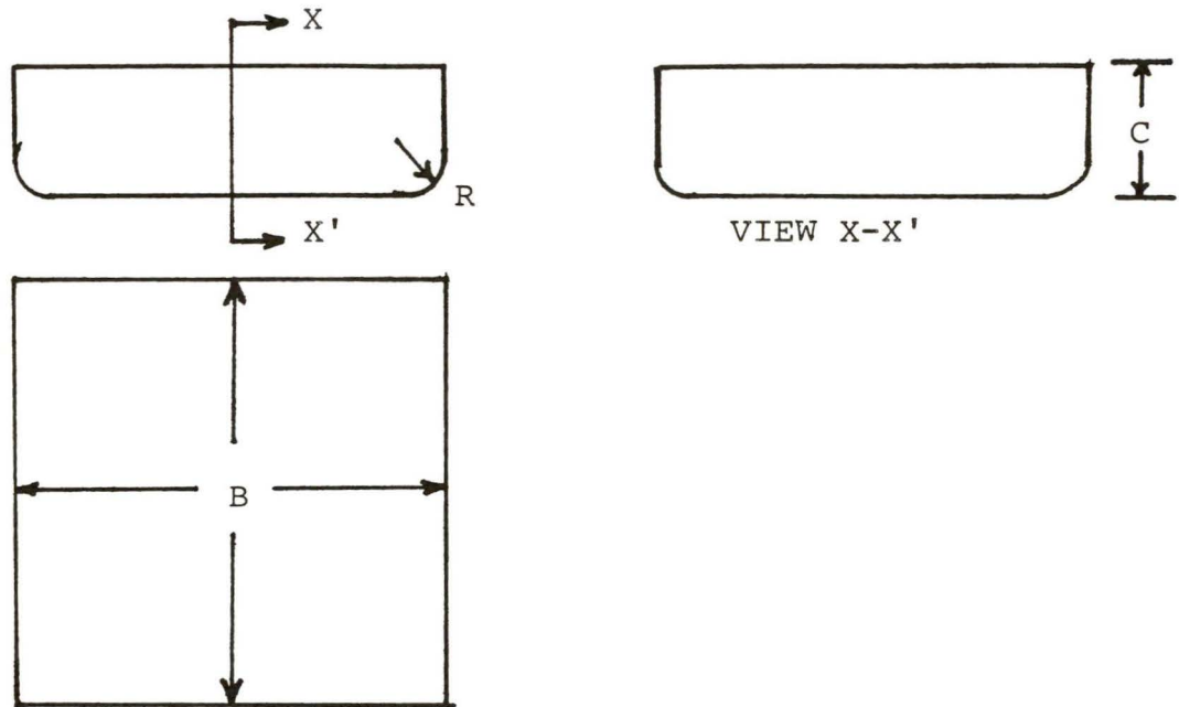
FIGURE 2.11 Bearing capacity plate dimensions.
