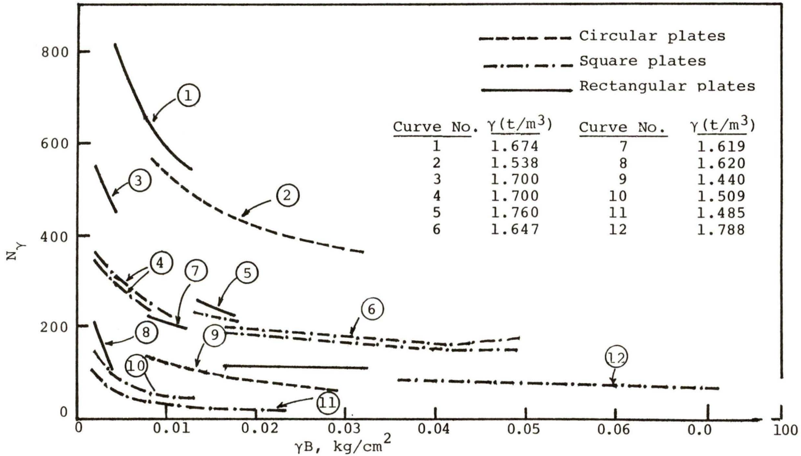
FIGURE 2.4. Effect of size on bearing capacity of shallow foundations. (After De Beer, 1965).
