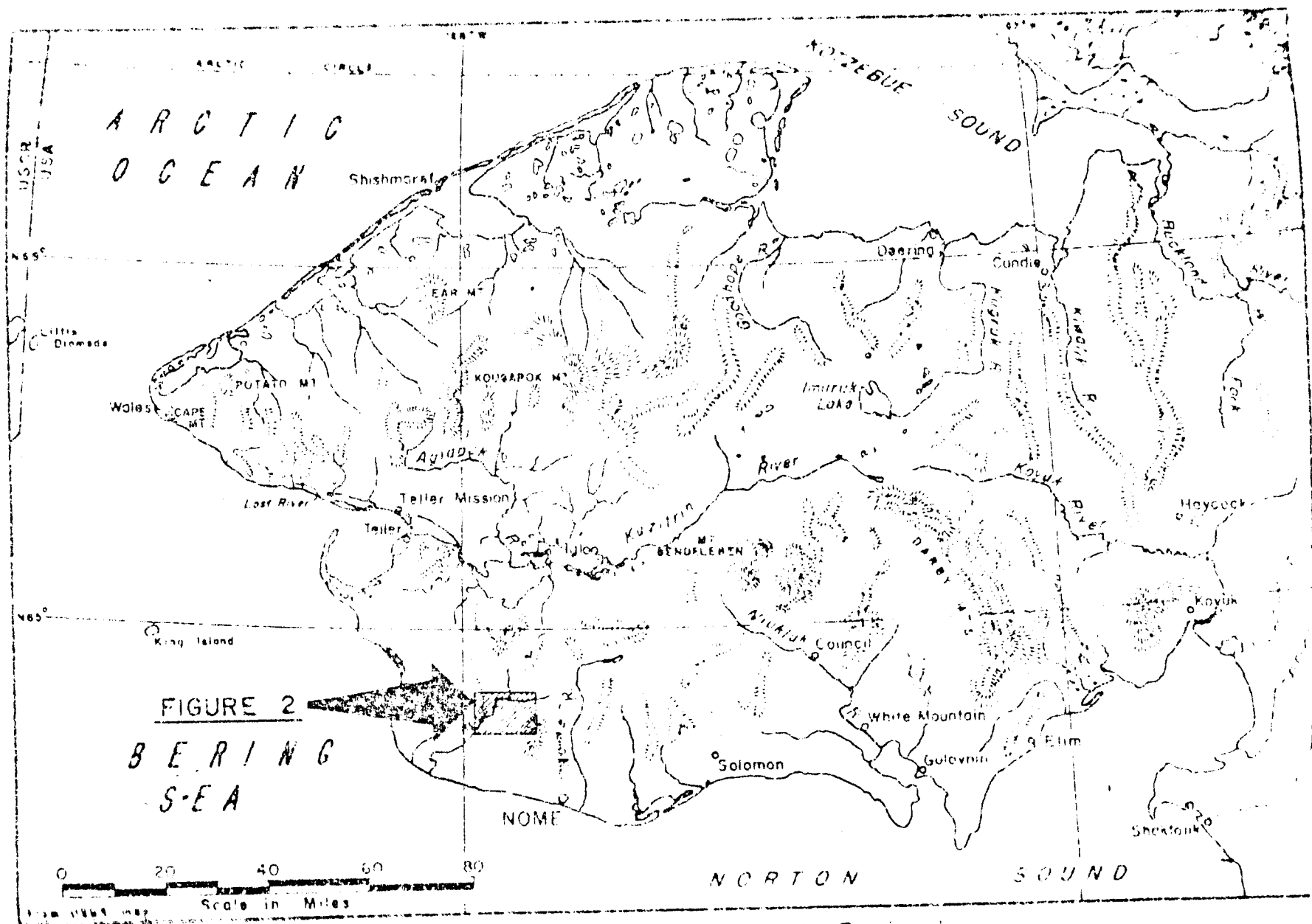
FIGURE 1-Index Map, Seward Peninsula.
