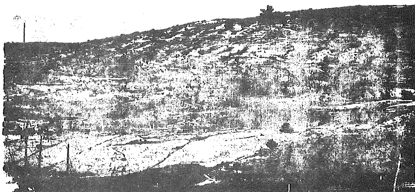
Figure 8. Collapse area over Lewis No. 1 and No. 2 mines. Outcrops of these mines are expressed by depressions and pillars and ridges. Mining was at a depth of less than 100 feet, and about ten feet of coal was extracted. Compare joints in exposed sandstone in foreground with same area shown on Figures 31 and 32. Locality 7, subsidence-inventory map.
