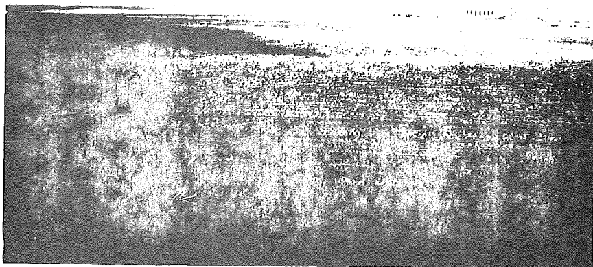
Figure 16. Broad swale over Lincoln mine. The swale in mid-foreground is fortuitously outlined by shadows cast by trees. Normally, this feature would be hard to discern with the unaided eye since it is quite broad (100 feet) and is only two or three feet deep. The mining depth at this locality is 50 to 200 feet and five to ten feet of coal has been extracted. Tipple of the Lincoln mine is in background. Locality 77, subsidence-inventory map.
