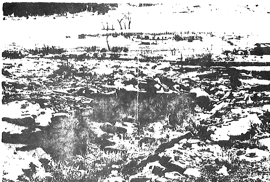
Figure 9. Collapse over room of Lewis No. 1 mine. Pit is about ten feet by 15 feet and is three feet deep. From five to ten feet of coal was extracted at a depth of approximately 50 feet. Flume carrying irrigation water in middle ground must be periodically re-set because underground fires in this area are causing continued subsidence. Locality 7, subsidence-inventory map.
