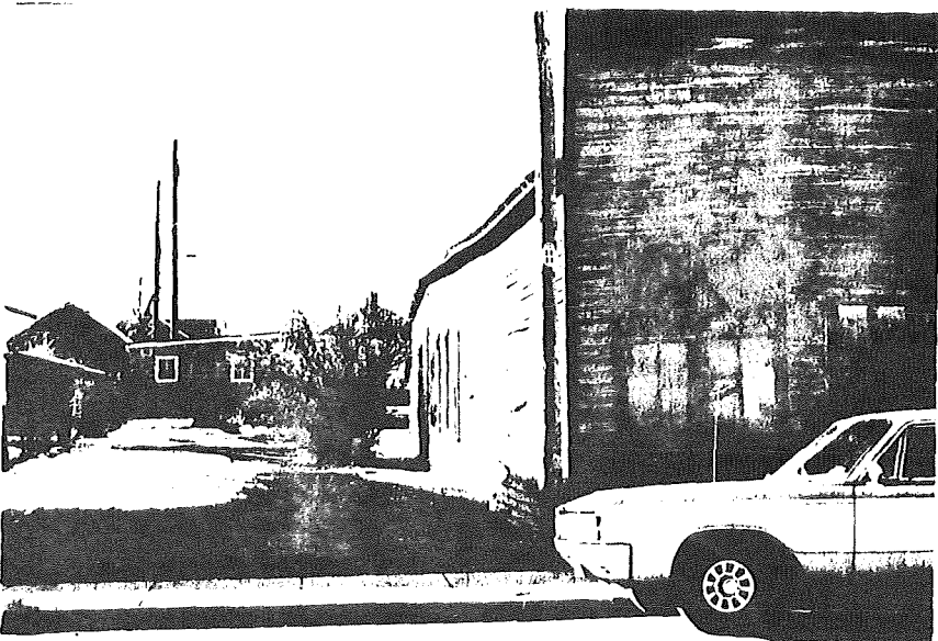
Figure 28. Abandoned building, Main Street, Louisville. The uniformity line of the siding and the rhomboid shape of the windows suggest torsional effects which might be associated with subsidence. However, the obvious age of the building suggests that the structural warping is simply due to general deterioration over a span of time. Locality 43, subsidence-inventory map.
