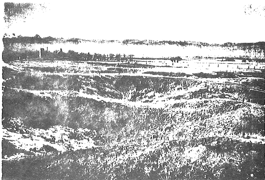
Figure 12. Large, well-developed subsidence pits over rooms at the Shanahan mine. Pits are eight to ten feet deep and 15 to 25 feet across. The coal seam at this mine was unusually thick (10 to 15 feet), which accounts for the large amount of vertical subsidence. The mining depth was less than 100 feet. Locality 21, subsidence-inventory map.
