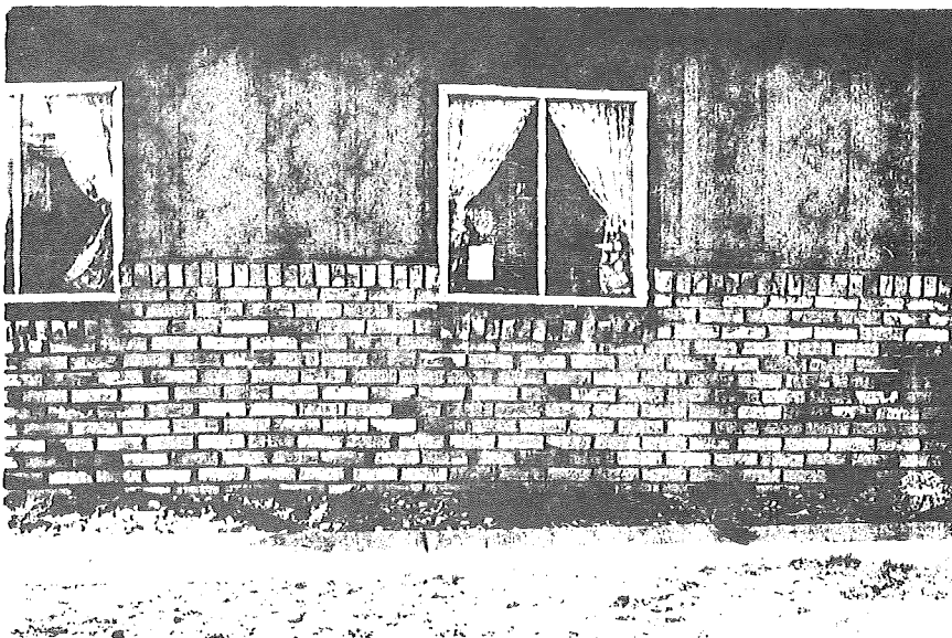
Figure 26. Detail of garage shown in Figure 24. Stairstep cracks and pickwork are one-half inch wide. Window has rhomboid shape, glass is cracked. This damage is similar to what one might expect if ground beneath foundation had subsided. Locality 15, subsidence-inventory map.
