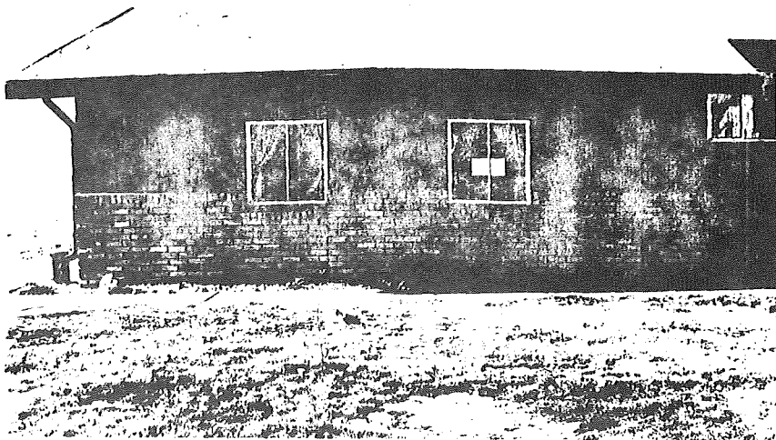
Figure 25. Garage over Black Diamond mine. At this locality, ten to ten feet of coal were extracted at a depth of 150 to 150 feet. The garage and house are fairly isolated, so that surrounding terrain is relatively undisturbed by man. No ditches, swales, or other indications of subsidence were found in fields around the house. For this reason, the damage to the garage is thought to be due to swelling soils. Note bow of roof line along gutter. Locality 15, subsidence-inventory map.
