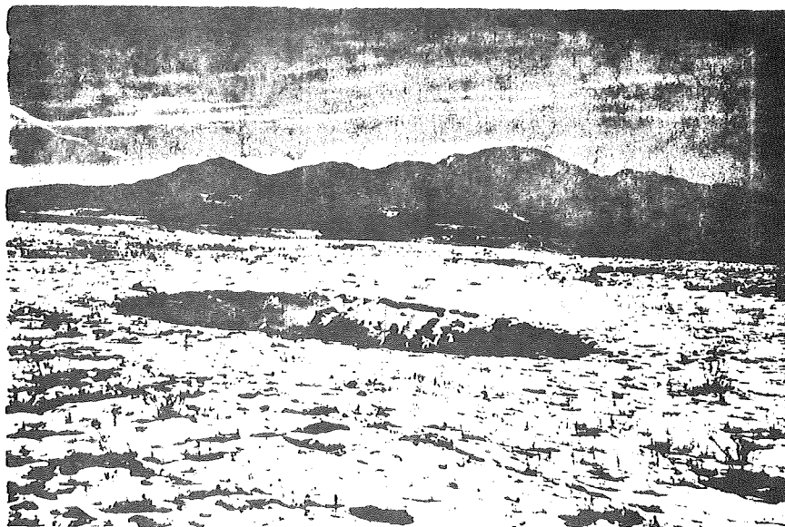
Figure 11. Large subsidence pit over the Premier mine. The pit is approximately 30 feet in diameter and eight feet deep. About ten feet of coal was mined at a depth of about 100 feet. Near locality 1, subsidence-inventory map.
