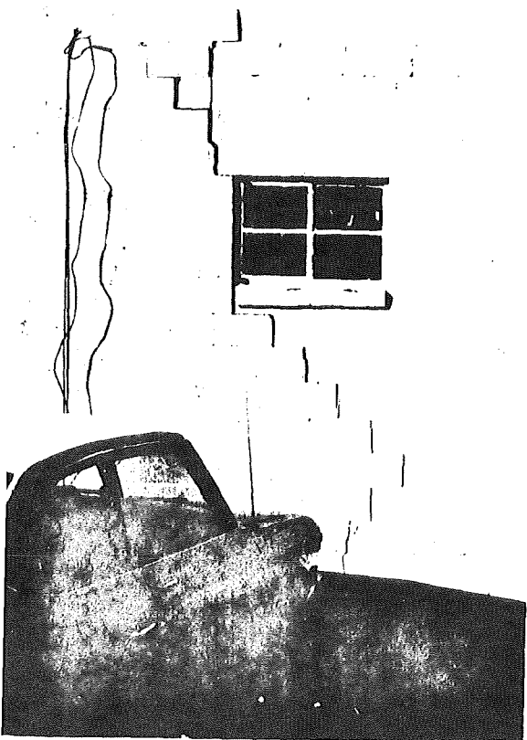
Figure 27. Damage to VFW hall, Main Street, Louisville. This part of Louisville was undermined many years ago. A seam 10 to 15 feet was extracted at a depth of about 100 feet. Because the mining occurred so long ago, it is thought that the damage to this relatively recent building is related to faulty design or construction, rather than to subsidence. Locality 43, subsidence-inventory map.
