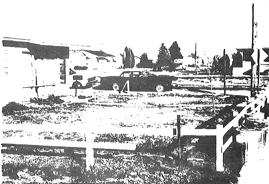
Figure 20. Subsidence over Strathmore mine, South Longmont, Colorado, Lafayette. The low sag in the front lawn and the irregular sidewalk are subsidence related. This "subsidence" is actually the result of compaction of trash and rubble used to fill a true subsidence pit which formed in 1956 (Denver Post, March 27, 1956). There was rapid collapse and overnight development of a hole 40 feet deep and 15 to 20 feet square. Locality shown on subsidence-inventory map.
