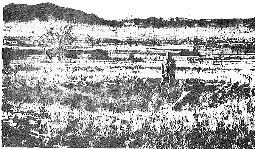
Figure 13. Collapse pit over the Allen Bond mine. Features such as this aided in locating the true position of the Allen Bond mine. The previously reported position of the mine showed no evidence of surface subsidence. A thick (10 to 15 feet) coal seam was mined here at a depth of approximately 100 feet. Locality 19, subsidence-inventory map.
