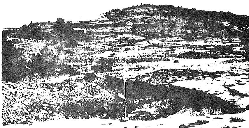
Figure 7. Collapse over room of Marshall No. 1 mine. The collapse area is approximately 15 feet by 30 feet and is about three feet deep. From five to ten feet of coal were extracted from this area at a depth of about 50 feet. Lower slopes of hill in background are also shown in Figures 6 (area A), 8, 31, and 32. Locality 4, subsidence-inventory
