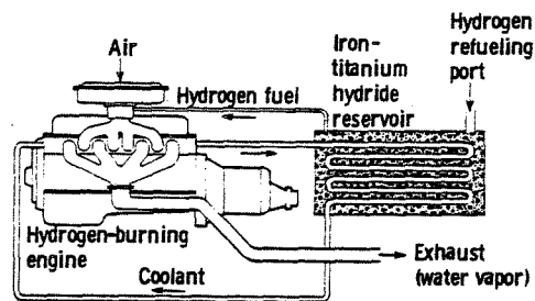
Figure 59. - Hydrogen storage heated by engine coolant.
