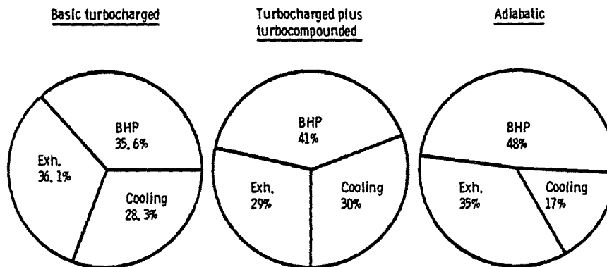
Figure 14. - Energy balance comparison (diesel engine).
