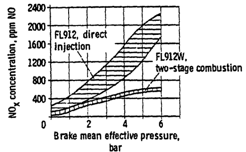
Figure 7. - NO x concentrations with direct injection compared to two-stage combustion.
