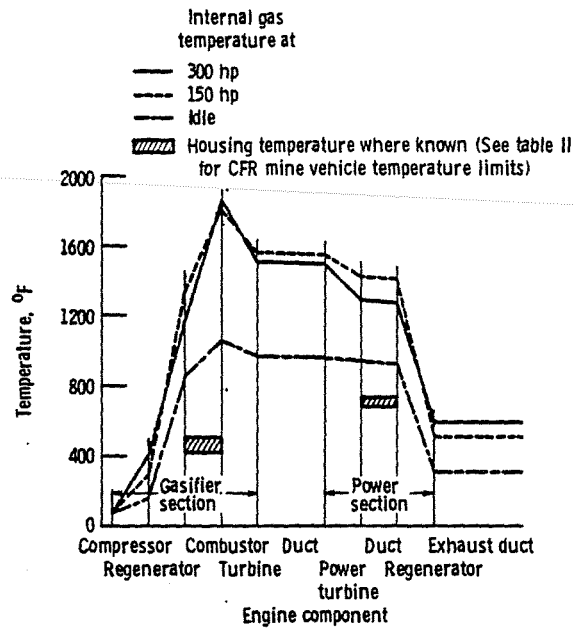
Figure 36. - IGT gas turbine temperatures.
