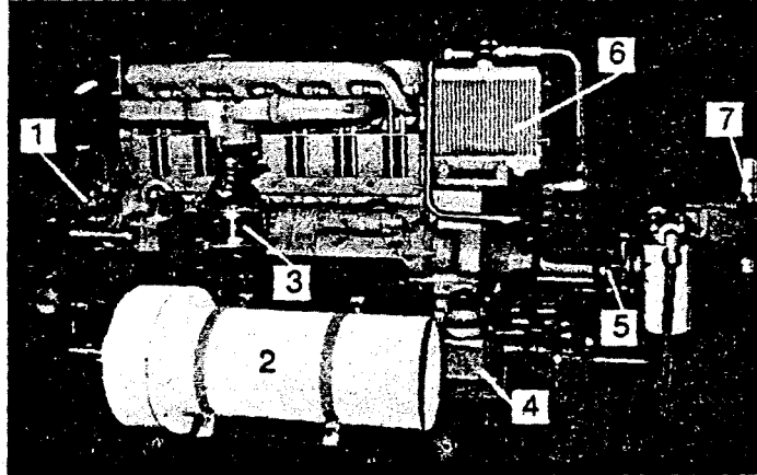
Figure 3. - Deutz air-cooled, six-cylinder, 75-hp schedule 24 engine package.
