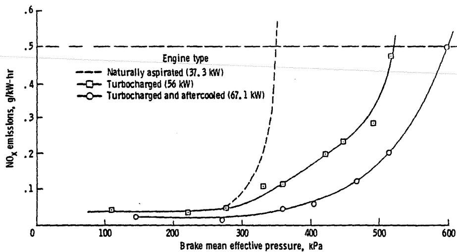
Figure 55. - Brake specific \text{NO}_x emissions vs. brake mean effective pressure for naturally aspirated, turbocharged, and turbocharged-aftercooled hydrogen engines. Turbocharged Caterpillar 3304; barometric pressure, 83.3 kPa; inlet air temperature, 24 \pm 3^\circ\text{C} ; compression ratio, 10.5; throttle, wide open; speed, 1800 rpm.
