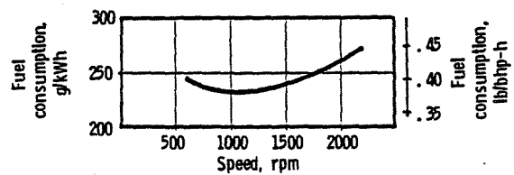
Figure 23. - United Stirling 4-275 engine full-load fuel consumption vs. speed.
