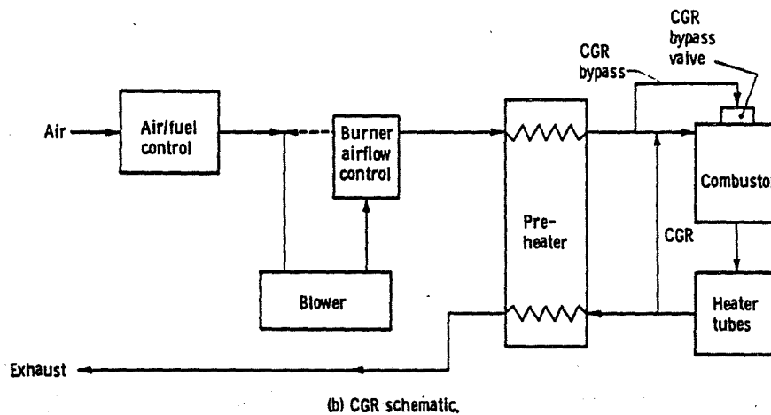
Figure 24. - Stirling engine \text{NO}_x emissions control systems.
