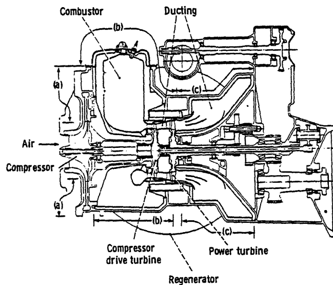
Figure 35. - IGT two-shaft engine.
