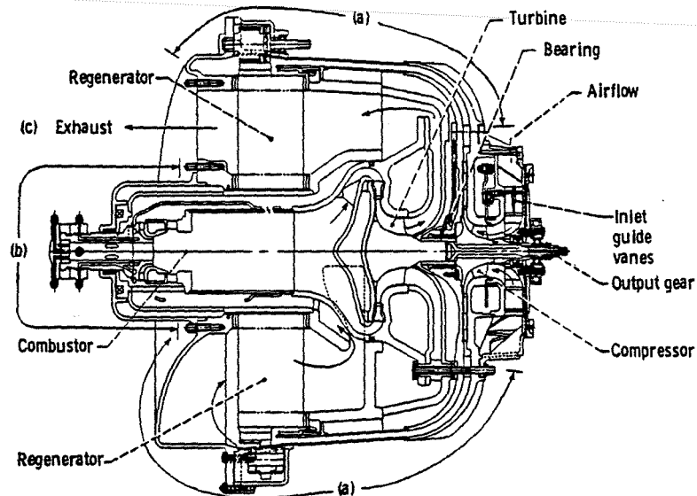
Figure 34. - AGT-101 single-shaft engine.
