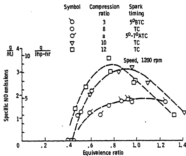
Figure 49. - Specific NO emissions as a function of equivalence ratio, for various compression ratios. Engine speed, 1200 rpm; spark timing as indicated.
