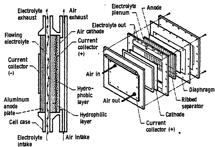
Figure 40. - Aluminum-air cell.
