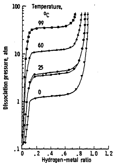
Figure 56. - Various isotherms for \text{Mn}_{1.4}\text{Al}_{0.5} annealed 4 hr at 1125^\circ\text{C} .
