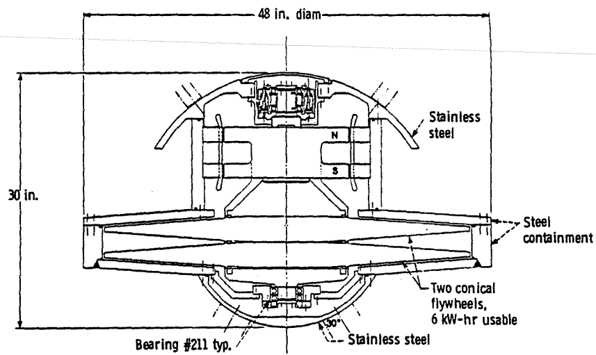
Figure 44. - Flywheel capsule (6 kW-hr).
