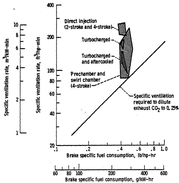
Figure 9. - Specific ventilation rate of diesel engines certified for CFR Part 32 (schedule 24, for nongassy noncoal mines and tunnels).
