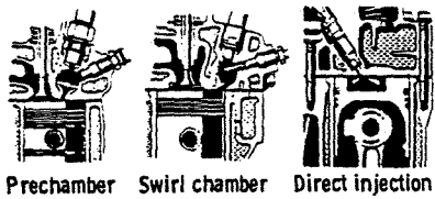
Figure 4. - Different combustion systems used in diesel engines.
