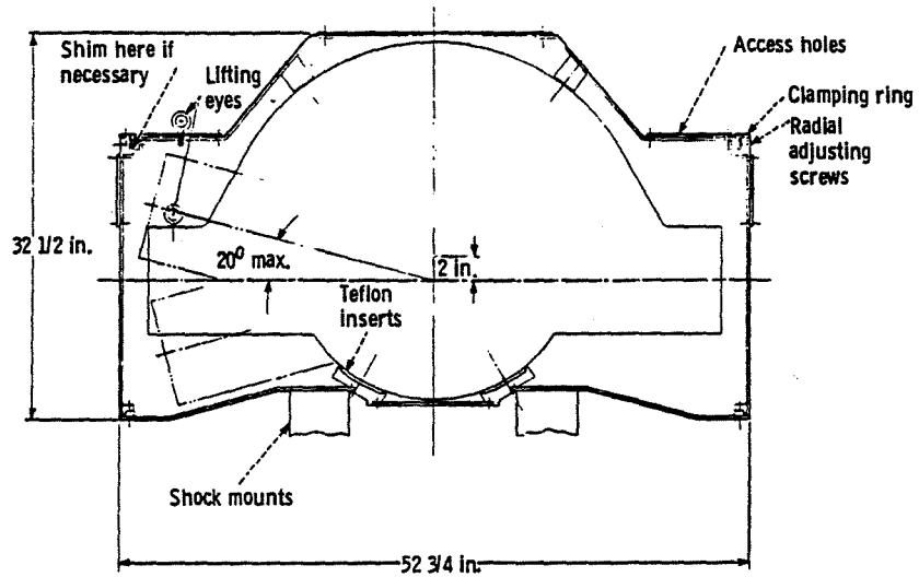
Figure 45. - Flywheel package (6 kW-hr).
