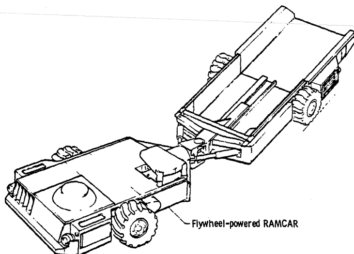
Figure 46. - Artist sketch; flywheel-powered RAMCAR.
