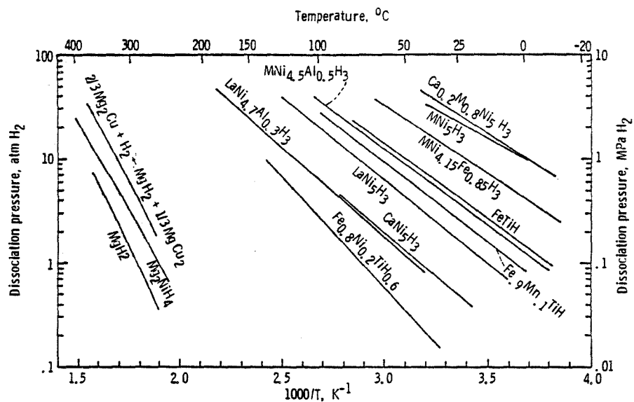
Figure 57. - Van't Hoff plots (desorption) for various hydrides.
