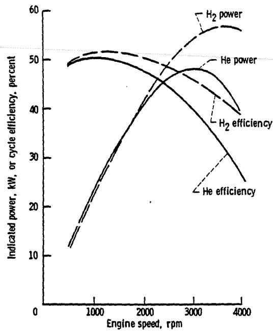
Figure 26. - Comparison of H 2 and He optimized Stirling engines. Cylinder temperature, 704° C; heater tube temperature, 724° C; cooler temperature, 57° C; pressure, 100 bar.
