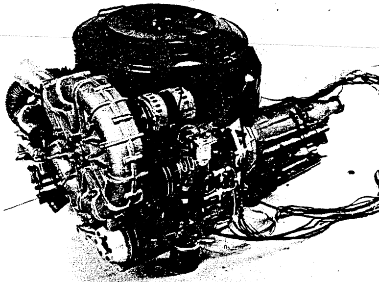
Figure 2L - United Stirling P-40 equipped for test installation in passenger car.
