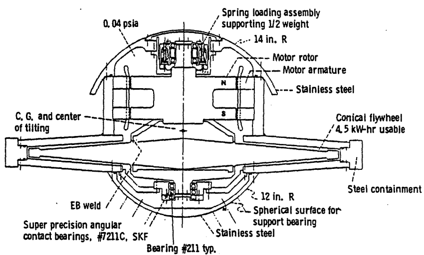
Figure 42. - Flywheel capsule (4.5 kW-hr).
