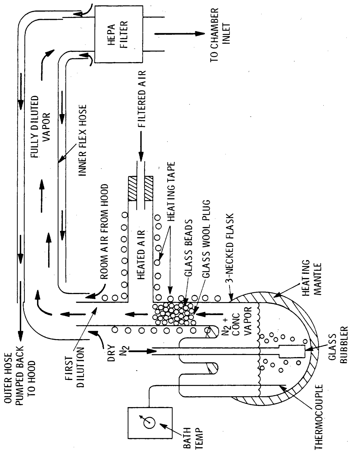
Figure 6. Details of vapor generator for styrene oxide.
