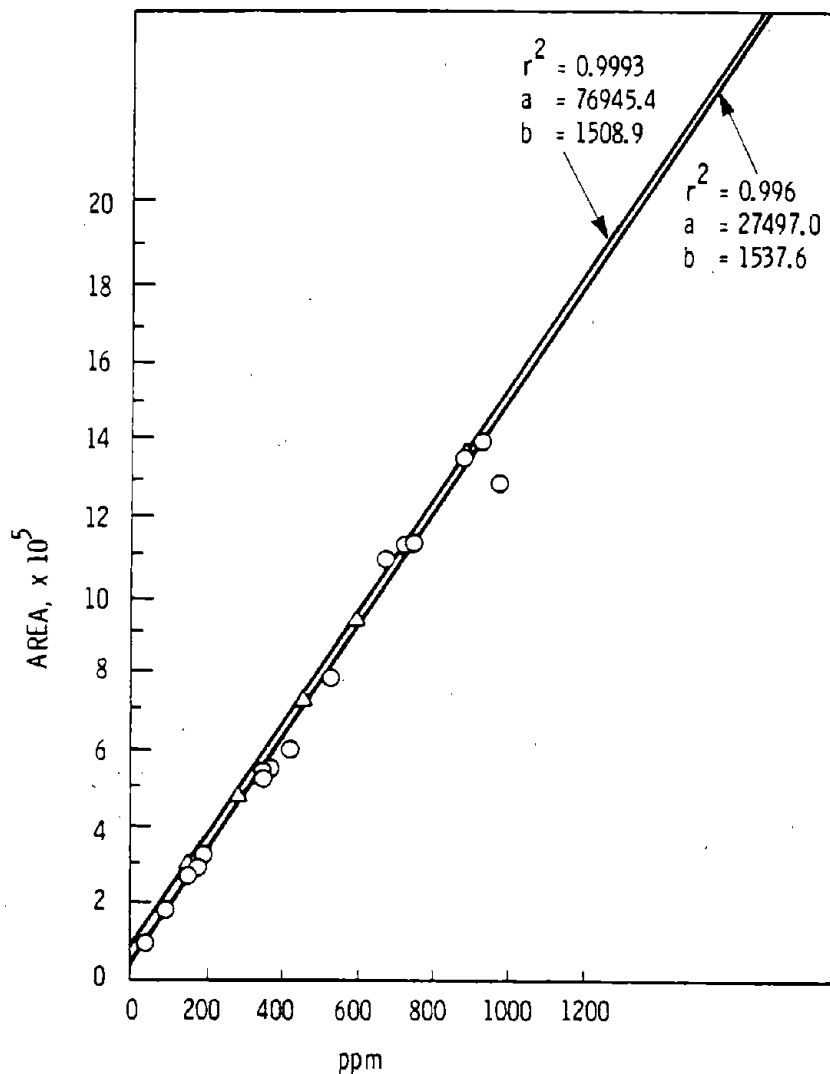
Figure 9. Comparison of standard curves for hexane generated by liquid \circ and vapor \Delta (gas bulb) dilutions.
