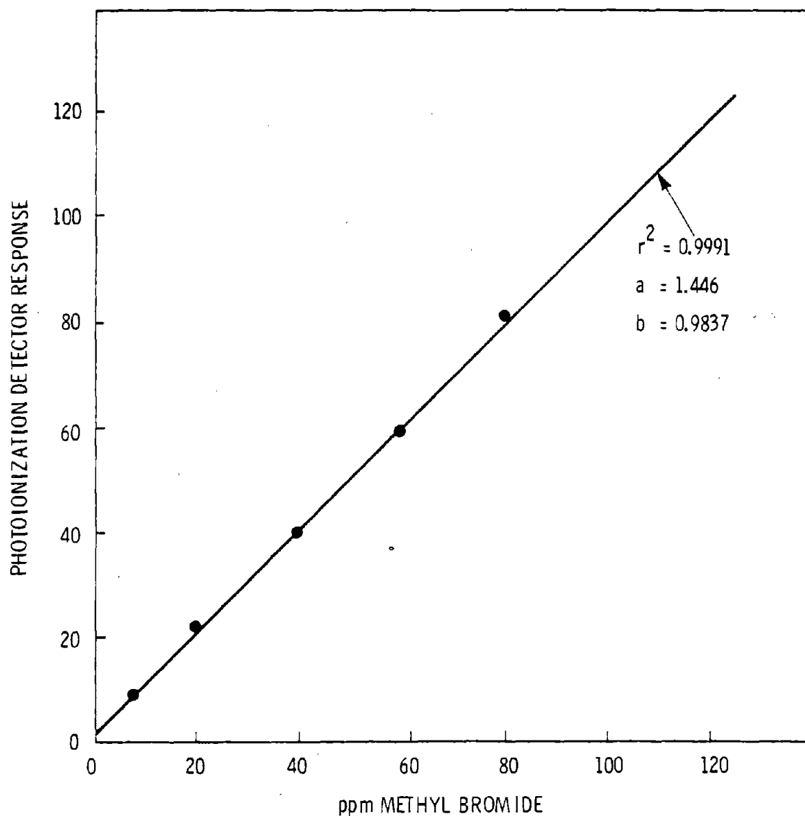
Figure 11. Typical calibration curve for photoionization detector response as a function of methyl bromide concentration.
