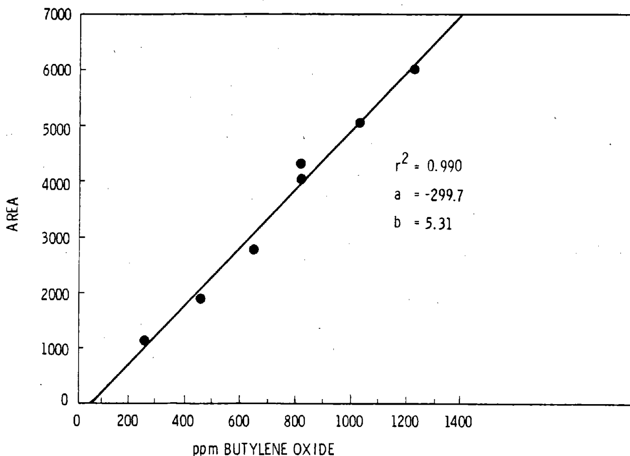
Figure 7. Typical standard calibration for butylene oxide.
