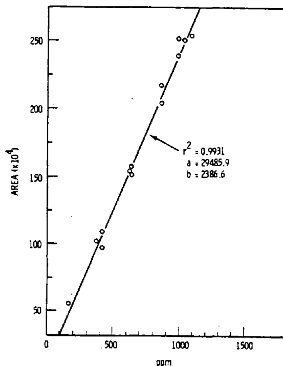
Figure 8. Typical standard curve for styrene oxide generation using liquid dilutions.
