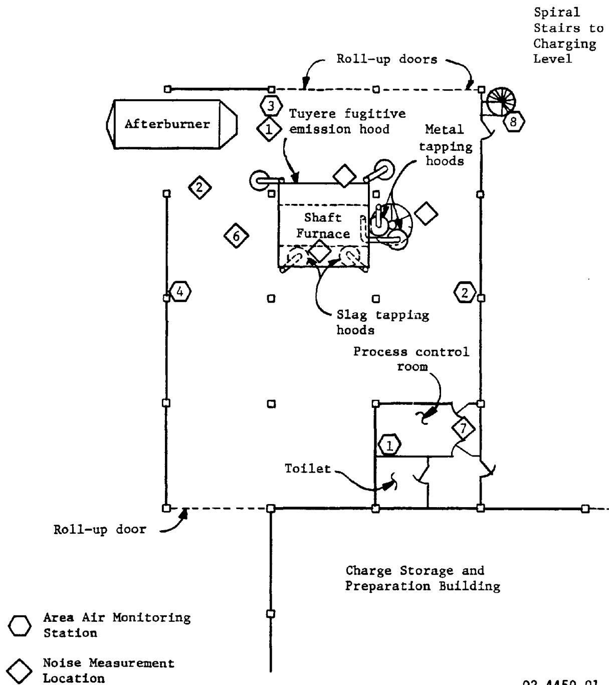
Figure 12. SB furnace ground level work area, SB furnace building.
