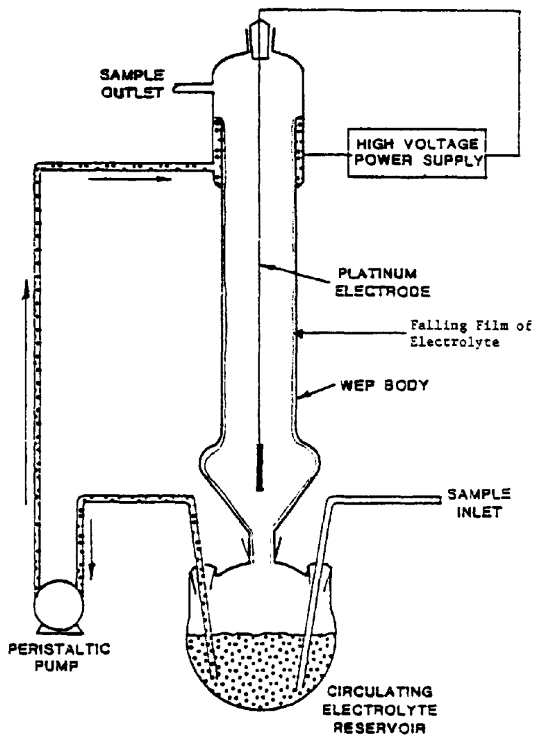
Figure 8. Wet electrostatic precipitator.
