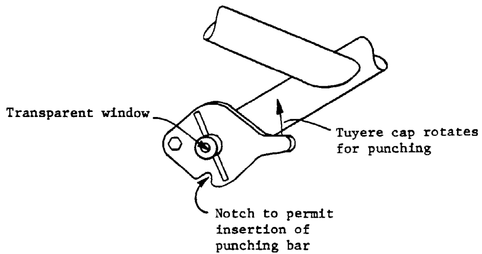
SB Furnace Tuyere
