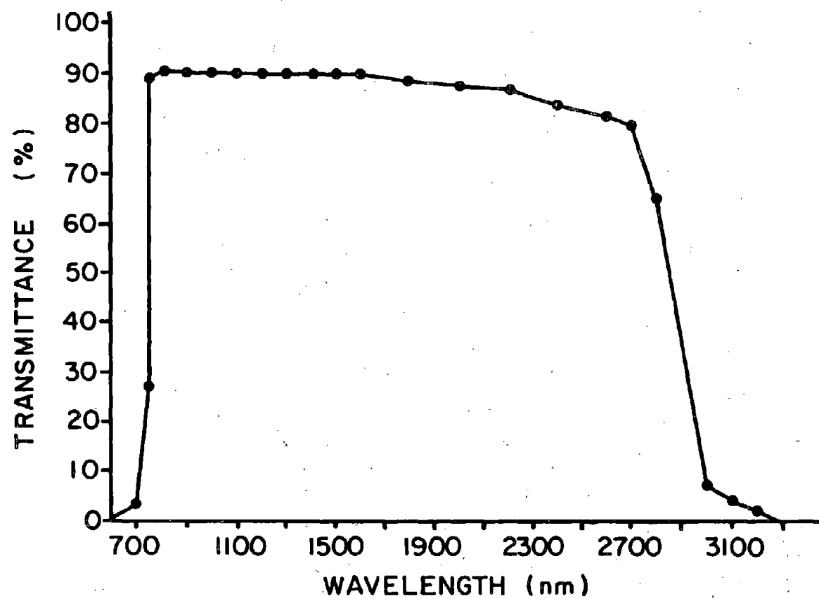
Figure 5. . Spectral transmittance of the Schott RG-715 filter.
