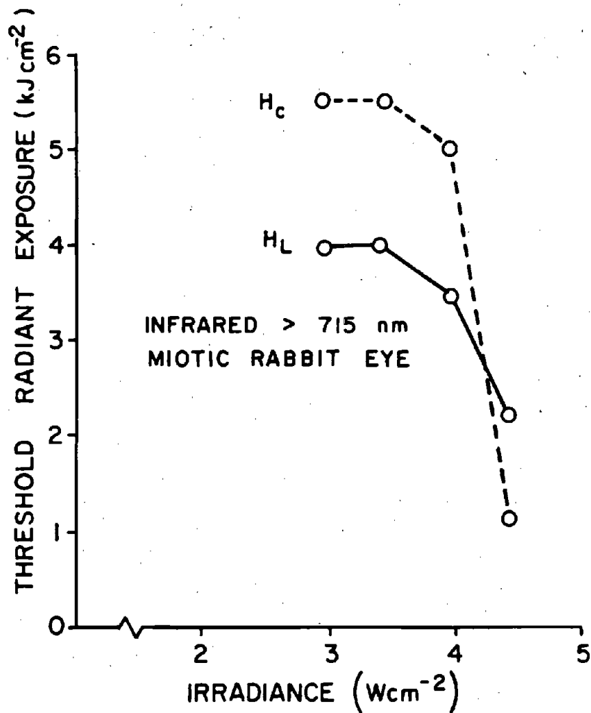
Figure 10. The threshold radiant exposure versus irradiance for the rabbit. These data show that the threshold varies with the rate of delivery of the source when the irradiance exceeds 3.5 W·cm -2 .
