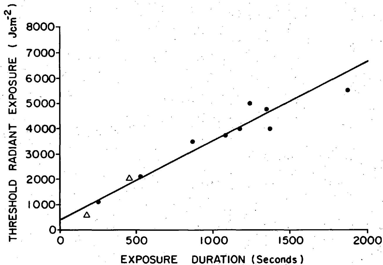
Figure 19. Radiant exposure required to produce a minimal lesion in the rabbit eye for different exposure durations. H_L in J \cdot cm^{-2} is plotted on the ordinate and exposure duration in seconds along the abscissa. The symbol (○) represents data for the IR spectrum, focused beam, and miotic pupil while the (Δ) is the data for full spectrum, focused beam, and miotic pupil.
