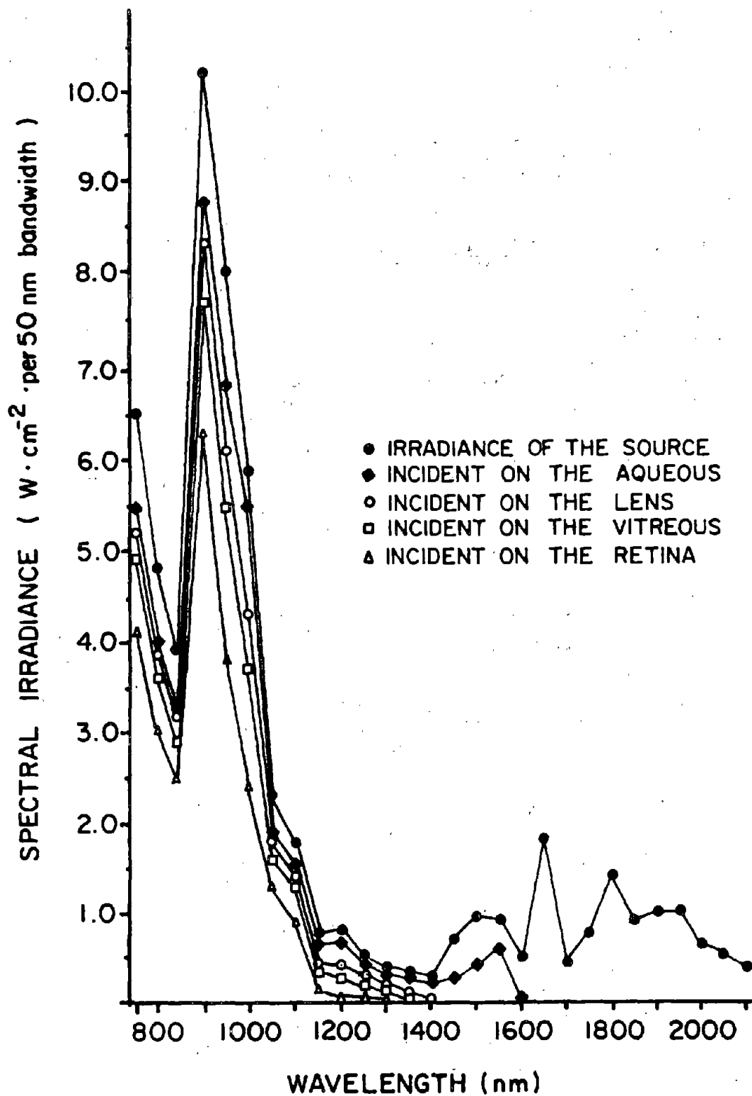
Figure 7. The spectral irradiance of the 5 kW Xenon source measured with an Eppley thermopile in 50 nm wavebands at the plane of exposure after transmittance through the Schott RG-715 filter. The irradiance incident on the aqueous, lens, vitreous, and retina was calculated from the rabbit transmittance data of Barker. 48
