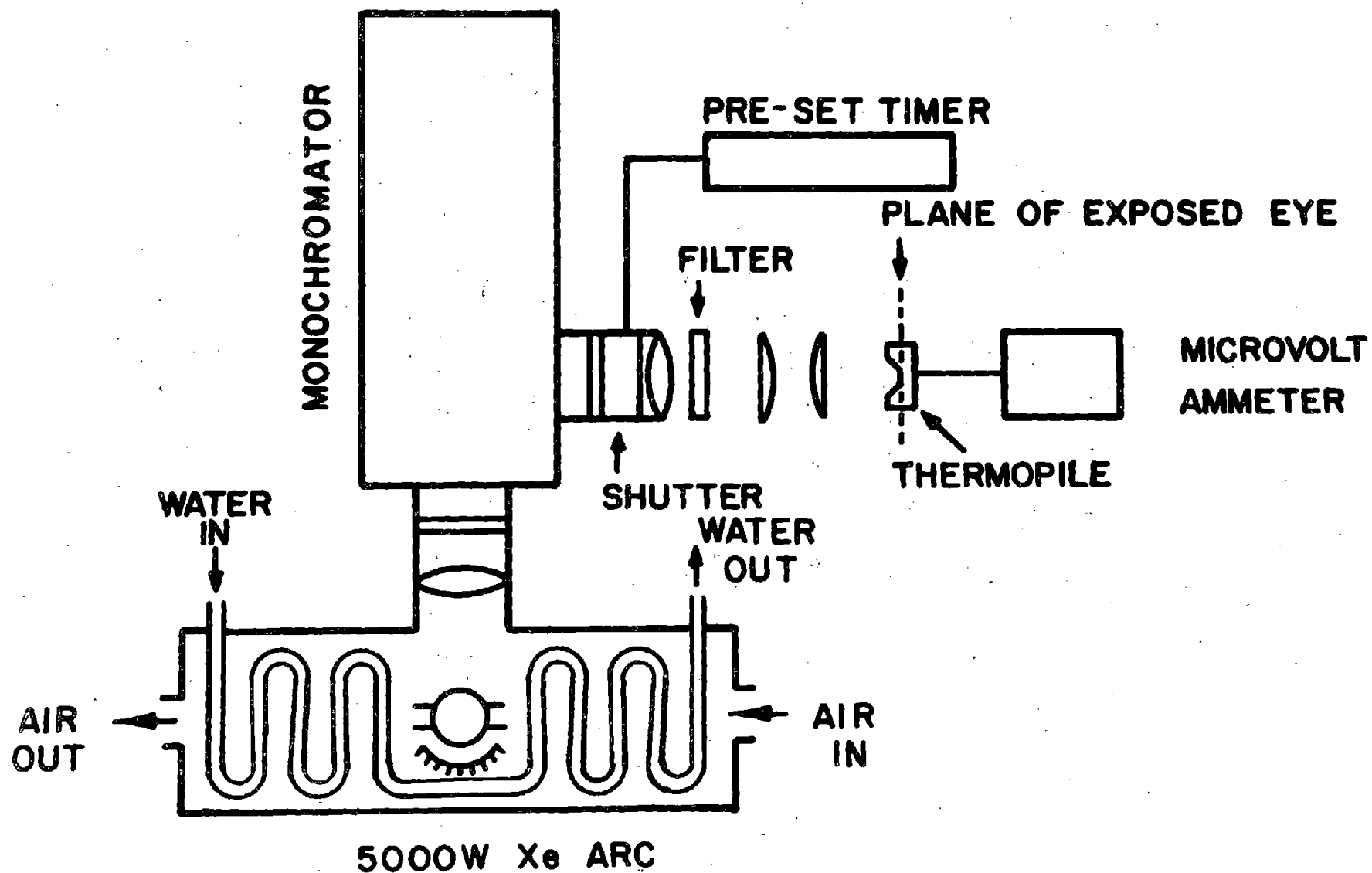
Figure 4. Schematic of the exposure instrumentation. See text for details of description of the system, source measurement, and exposure procedures.
