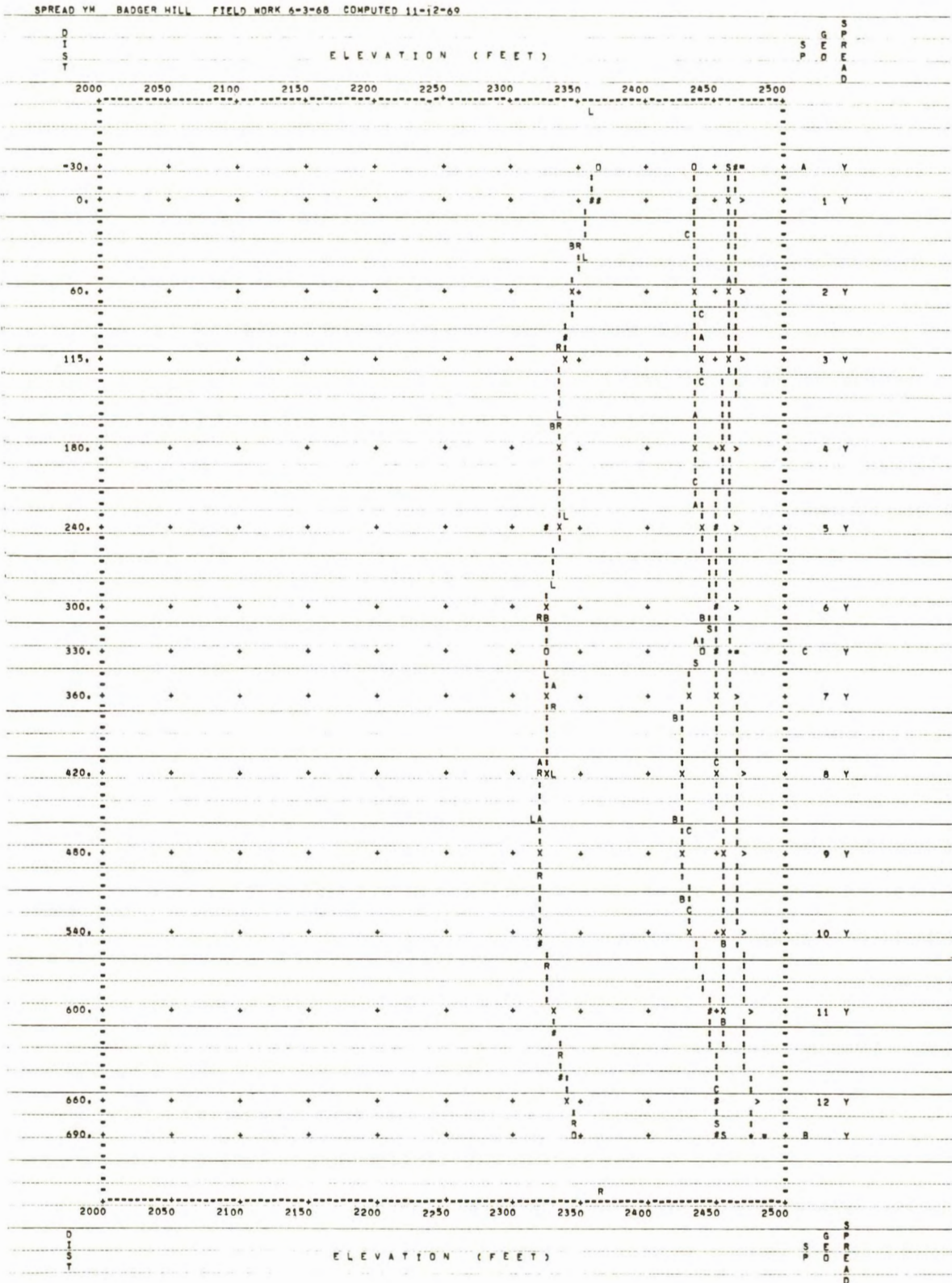
FIGURE 6. - Computer Plot of Seismic Profile YM.
