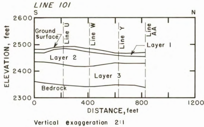
FIGURE 10. - Cross Section Showing Results of Seismic-Refraction Profile 101.
