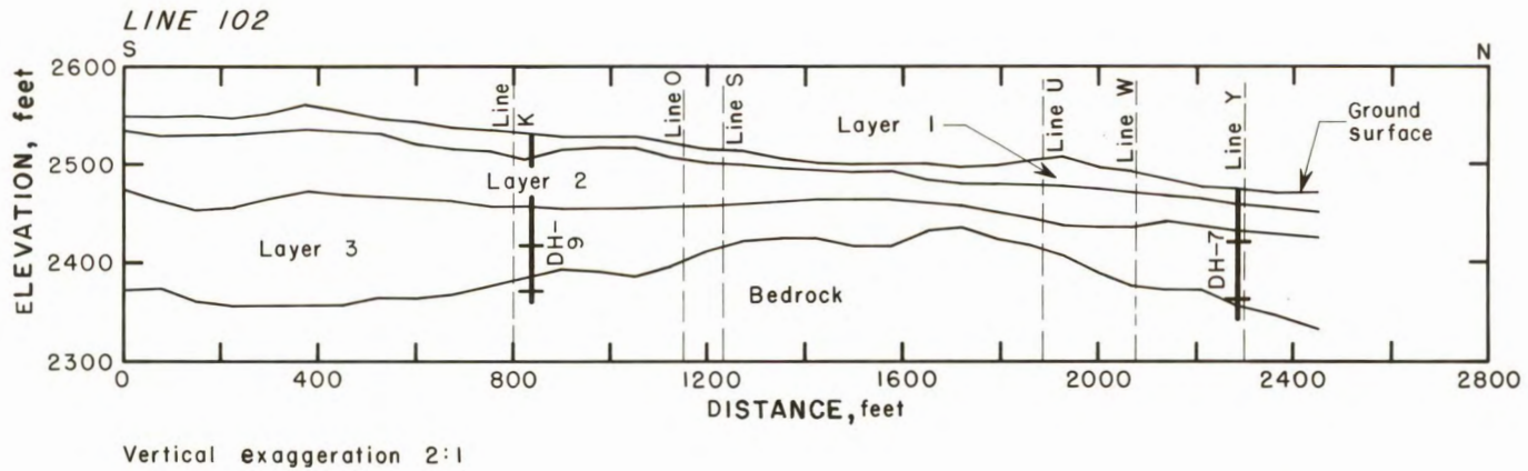
FIGURE 11. - Cross Section Showing Results of Seismic-Refraction Profile 102, and Drill Hole Depths to Layers 3 and 4.
