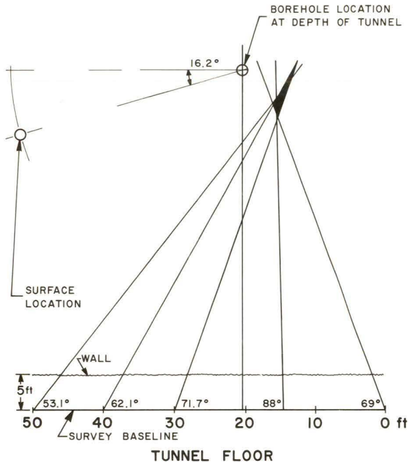
FIGURE 7. - Results of field test at Ft. Ritchie, Md.
