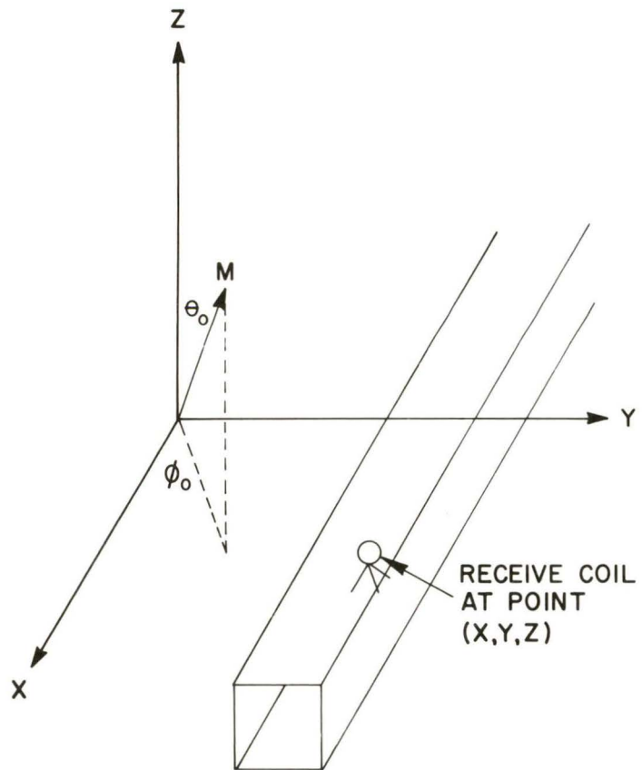
FIGURE B-1. - Coordinate system with the transmitter at the origin.
