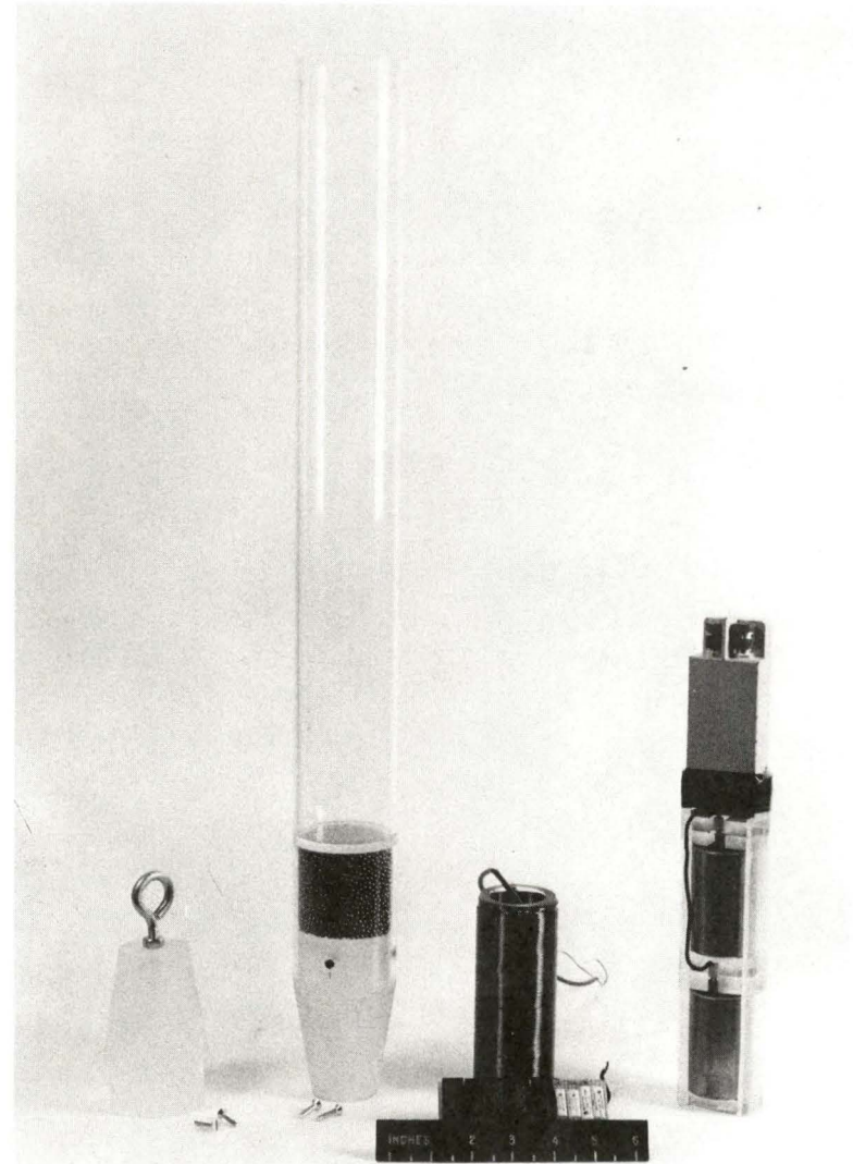
FIGURE 4. - Transmitter disassembled showing from left to right, top seal, plastic case, coil and tuning capacitors, transmitter module, and batteries.
