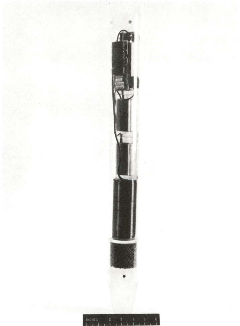
FIGURE 3. - Borehole transmitter.
