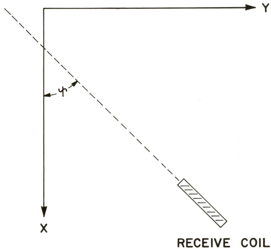
FIGURE B-2. - Plane view of the coil in the null direction.
