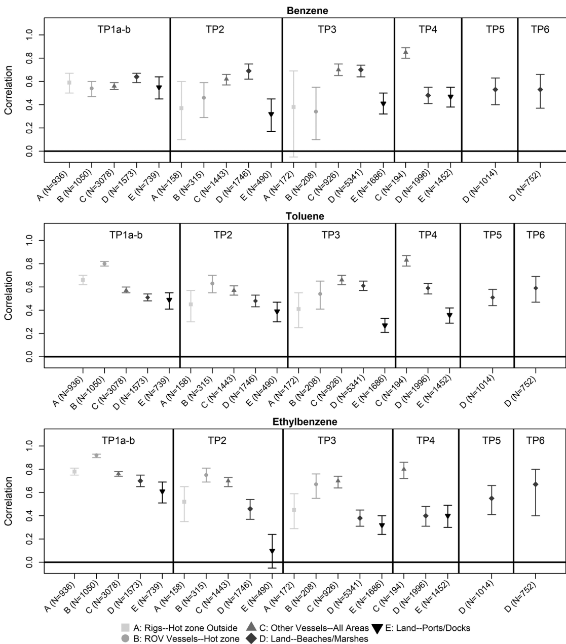
Figure 1. Benzene, toluene, ethylbenzene correlations with total hydrocarbons (THC) by time period. Correlations reflect all outside areas within a particular group. The error bars represent the 95% credible interval and the points represent the median posterior estimate.
