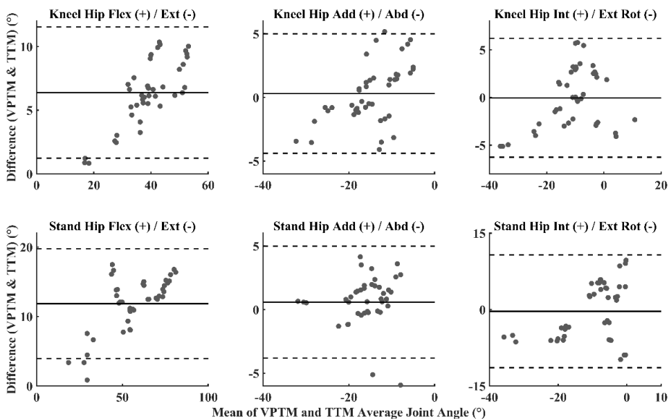
Fig. 5. BA plots of the average HJAs for all trials. The black solid line represents the mean difference, and the black dashed lines represent the mean difference \pm 2 std (upper and lower limits of agreement). Flexion/Extension (Flex/Ext), Adduction/Abduction (Add/Abd), Internal/External Rotation (Int/Ext Rot).
