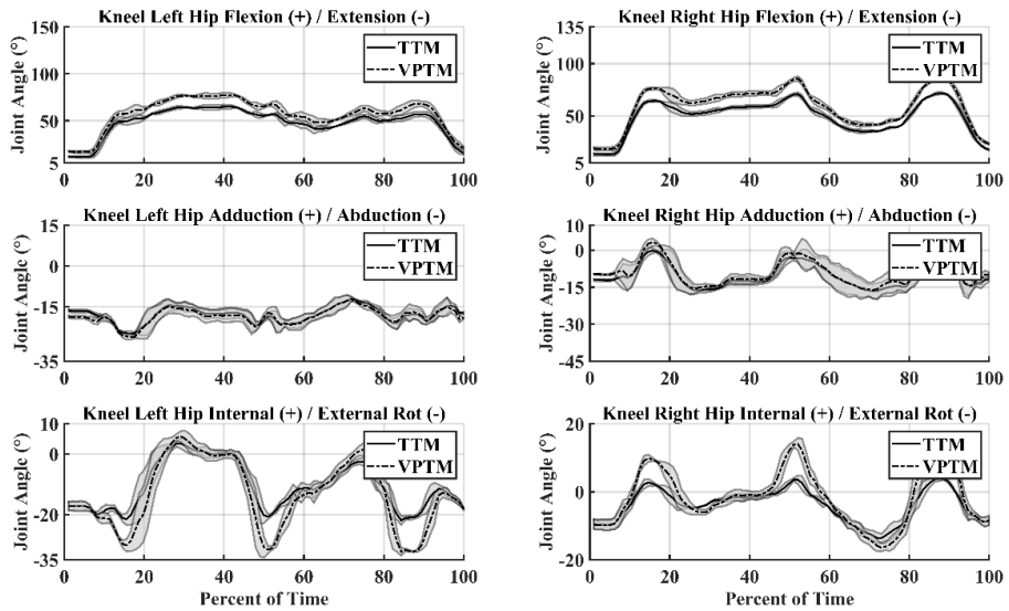
Fig. 6. A representative subject's mean kneeling task HJAs with standard deviation (shaded region) for the TTM and VPTM.
