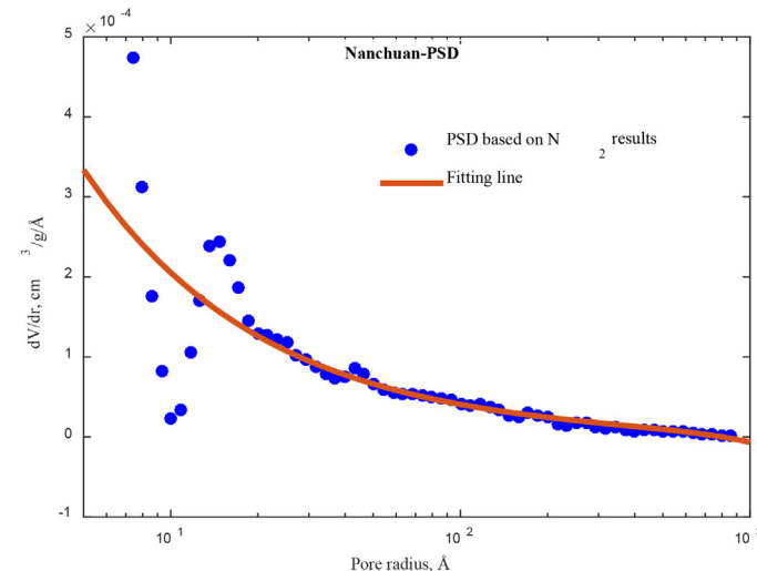
Fig. 2. Pore size distributions (PSD) and idealized curve fits of the two shales, based on DFT analysis.
