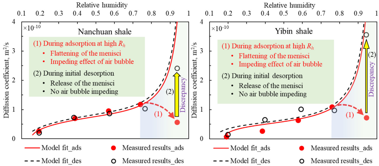
Fig. 7. Comparison between model and observations for Nanchuan (left) and Yibin (right) shales. Fitting parameters are \tau_s^* = 16 , \tau_l^* = 30 , n = 0.5 for Nanchuan shale; and \tau_s^* = 18 , \tau_l^* = 30 , n = 0.5 for Yibin shale and are constant with R_h and for both adsorption and desorption.
