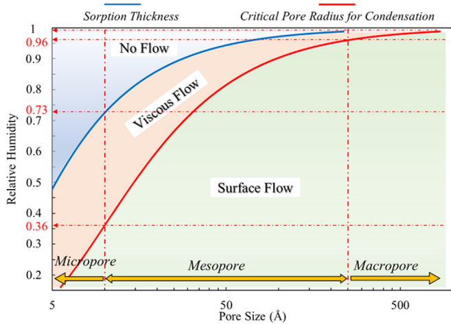
Fig. 14. Different flow modes potentially occurring in micro-/meso-/macropores under the spectrum of R_h conditions. Note that pore size refers to the radius of the capillaries. Flow modes occurring in different pore sizes are classified based on a critical pore radius for condensation and film thickness l_s ( l_s < r_{ca} ). Given a pore size r , if r > r_{ca} , only surface flow occurs; if l_s < r < r_{ca} , only viscous flow of condensate occurs; if r < l_s , no flow occurs in this pore.
