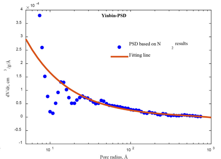
Fig. 2. Pore size distributions (PSD) and idealized curve fits of the two shales, based on DFT analysis.
