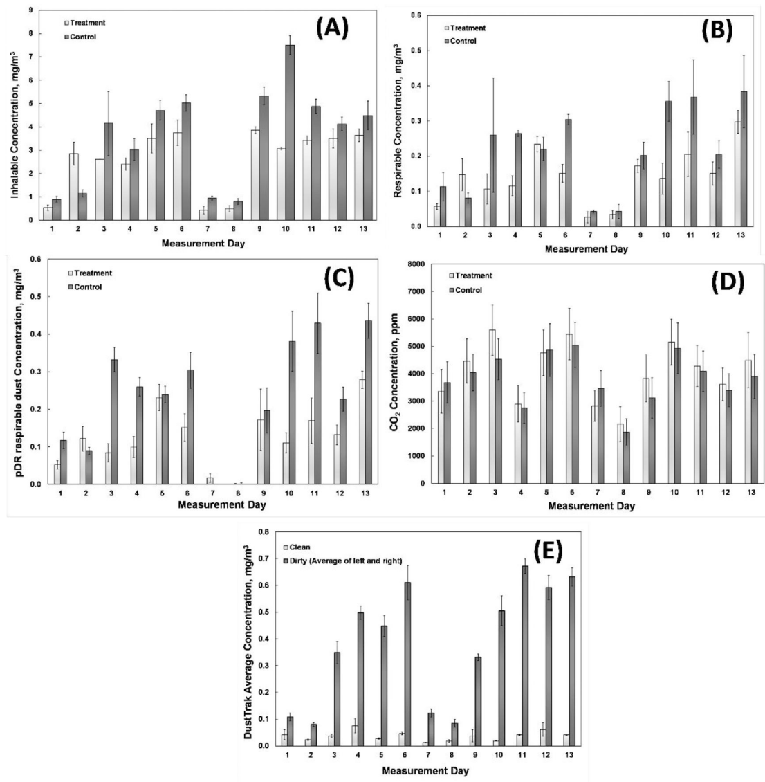
Figure 5. The 24-hr average concentrations inhalable dust (A), respirable dust (B), pDR respirable dust (C), and CO 2 (D) in swine farrowing treatment room (TR) and control room (CR). Recirculating ventilation system exhaust air and reentry dust concentrations for the TR (E). The y-axis error bars represent the standard deviation in the measurements among the three sampling locations in the TR and CR.
