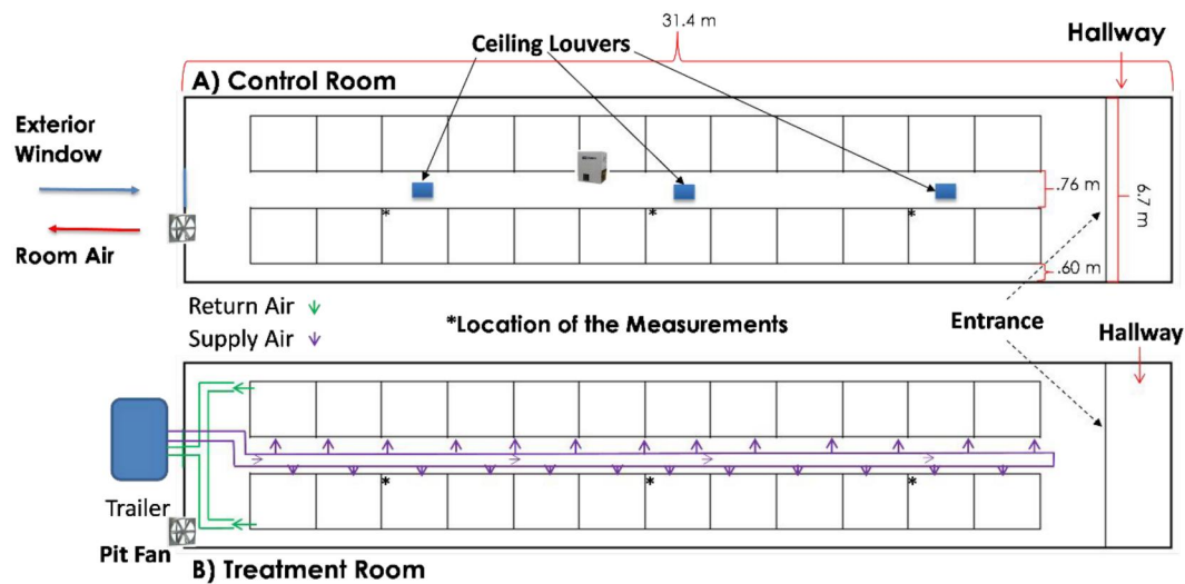
Figure 1. Layout for (A) control room and (B) treatment room layout showing the mobile air handling unit and duct system installed outside the treatment room, the ceiling louvers, radial fans, entrance, and the location of the measurements. This figure does not represent a floor plan but is only intended to provide a simple schematic of both rooms.
