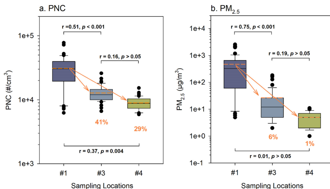
Fig. 6. (a) PNC and (b) PM 2.5 at indoor sampling locations 1 (inside vape shop) as well as outdoor sampling locations 3 (outside ~1–3 m away from the vape shop door) and 4 (outside ~6–8 m away from the vape shop door) for vape shop I. The solid line in each box represents the median value, and the dash line in each box represents the mean value.
