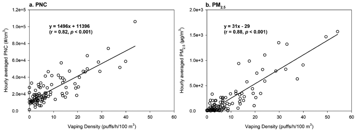
Fig. 3. Relationships between hourly averaged PNC and PM 2.5 and vaping density (puffs/h/100 m³) when the shop door was closed for vape shops A–F and I with particle samplings.
