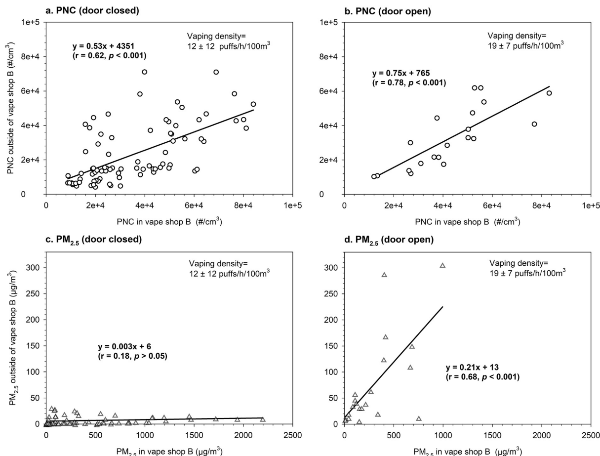
Fig. 5. Effects of door open and close on the particle transport from vape shop B to the outdoor environment (i.e., sampling location 3: ~1–3 m away from the front door of vape shop B).
