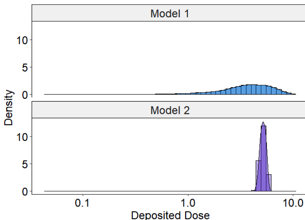
Fig. 3. Comparison of estimated deposited doses estimated by Models 1 and 2*
