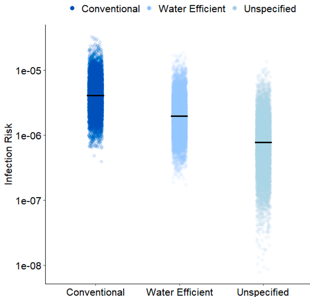
Fig. 2. Infection risks for a 7.8-min shower at a concentration of 100 L. pneumophila CFU/L*
