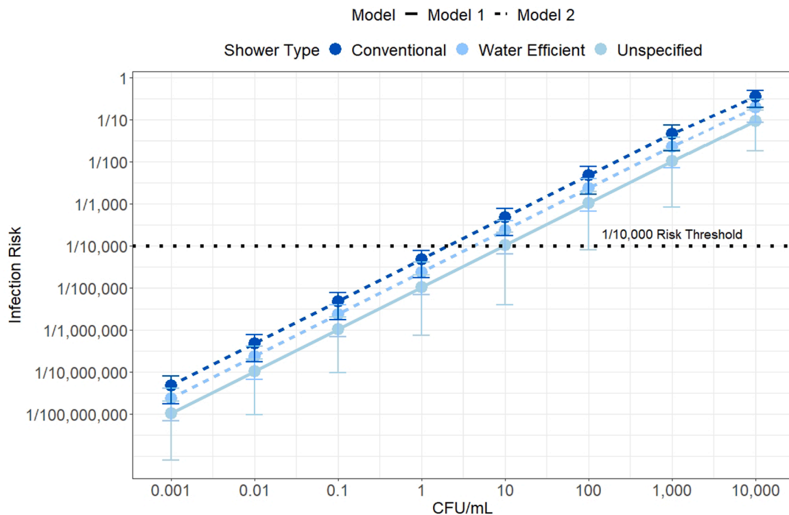
Fig. 1. Infection risks for a 7.8-min shower and a range of L. pneumophila concentrations (CFU/mL). “Unspecified” risk estimates come from Model 1, where the type of shower in the original work describing the model (Schoen and Ashbolt, 2011) does not specify the shower as conventional or water efficient.
