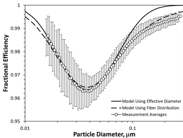
Figure 5. Measured efficiency values with error bars (standard deviation) averaged across all six N95 filtering layers assessed in this study. The corresponding total efficiency curves incorporating either an effective diameter or a distribution of fiber diameters are also shown and utilized filter characteristics given as suggested values in Tables 1 and 3.
