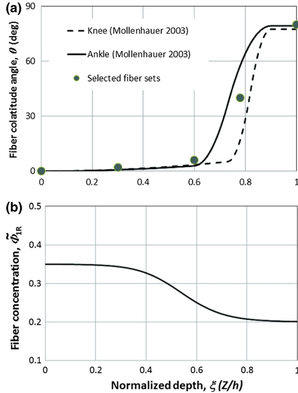
FIG. 2. The fiber orientation and volumetric concentration as a function of cartilage depth. a The fiber orientation for representative human ankle and knee cartilage layers [28]. From the deep zone ( \xi=0 ) to the superficial zone ( \xi=1.0 ), the fiber orientation varies from nearly vertical to the contact surface (approximately 0^\circ ) to nearly parallel to the contact surface (approximately 80^\circ ). A set of five fiber orientations ( symbols ) are selected to represent the test data. b Fiber volumetric fraction with respect to the solid, \tilde{\phi}_{1R}(\xi) , as a function of cartilage depth (constructed based on experimental data [5,36])
