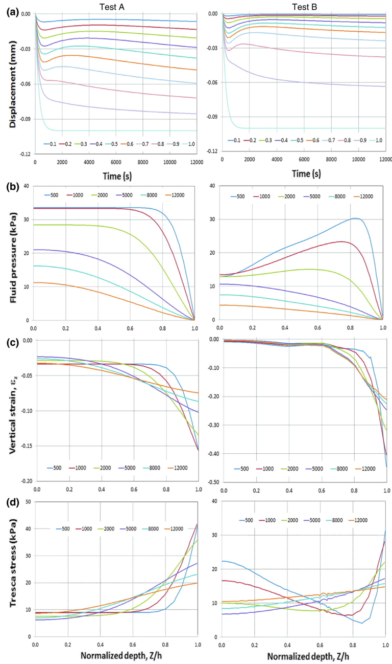
FIG. 5. The predicted vertical displacements, fluid pressure, vertical nominal strain, and Tresca stress as a function of cartilage depth and time for Tests A and B (isotropic models). All parameters were taken at R = 0 , where R is the referential radial coordinate. a vertical displacement. b Fluid pressure. c Vertical nominal strain. d Tresca stress. Left column Test A. Right column Test B. The time histories of the vertical displacement at ten different depths ( \xi = Z/h equal to 0.1, 0.2, 0.3, 0.4, 0.5, 0.6, 0.7, 0.8, 0.9, 1.0) are plotted. \xi is the normalized depth with \xi = 0 and 1.0 referring to the bone–cartilage interface and contact surface, respectively. The fluid pressure, vertical nominal strain, and Tresca stress for six time points ( t equal to 500, 1000, 2000, 5000, 8000, and 12000 s) across the cartilage layer are plotted
