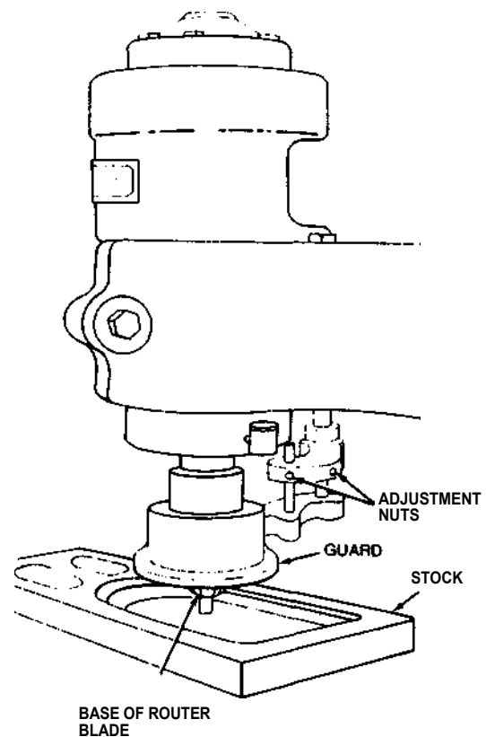
Example of adjustable tool guard on router from Concepts and Techniques of Machine Safeguarding, 1992.
