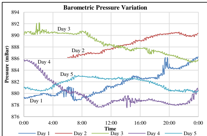
Figure 10. Barometric pressure data measured at the surface from study site during tracer gas testing of the gob.
