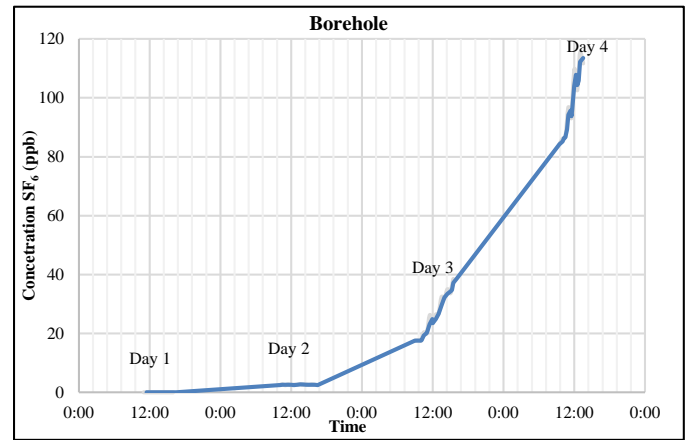
Figure 9. Increasing concentrations of SF 6 measured at the surface borehole site during the gob test.
