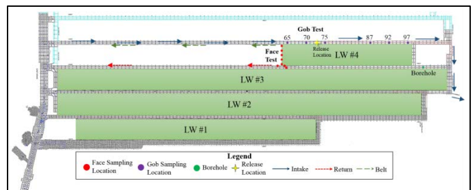
Figure 1. Mine study site. Study panel is panel 4. Green color indicates mined-out portions of longwall panel blocks.
