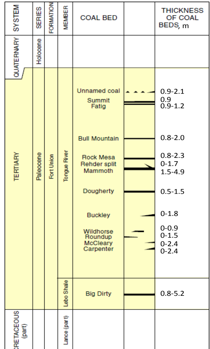
Figure 3. Local stratigraphy and coal beds, Bull Mountain Basin Mt, Fort Union Formation. Mine operator is working in Mammoth Coal bed. Modified from Woolsey et al., 1917; Connor and Biewick, 1989; Stricker 1999.
