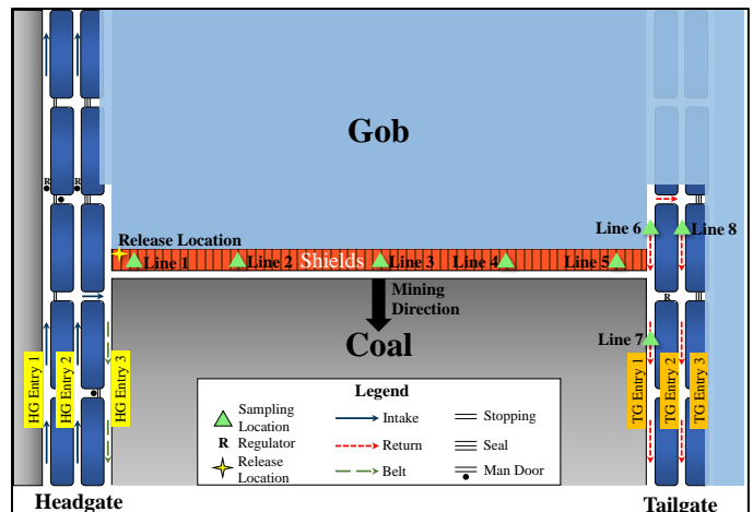
Figure 2. Study site. Near-face ventilation configuration and sampling locations.
