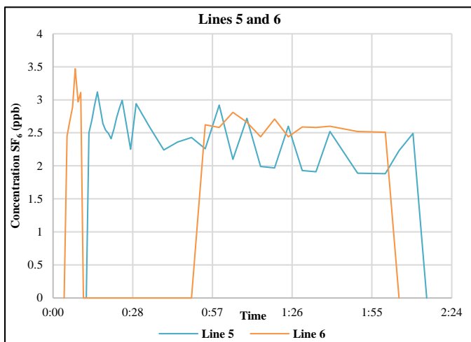
Figure 5. Tracer gas concentrations determined for sampling during face test over test duration, sample lines 5 and 6. The arrival and peak occurred on line 6 located inby the face in the former, first tailgate gateroad, prior to the arrival and peak on sample line 5 at shield 177.
