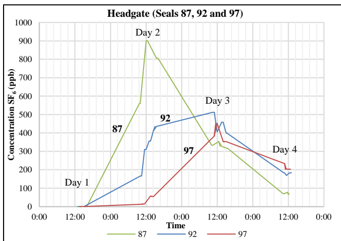
Figure 8. Tracer gas concentrations determined for sampling during gob test from headgate locations at the inby set of monitoring locations, seals 87, 92, and 97.
