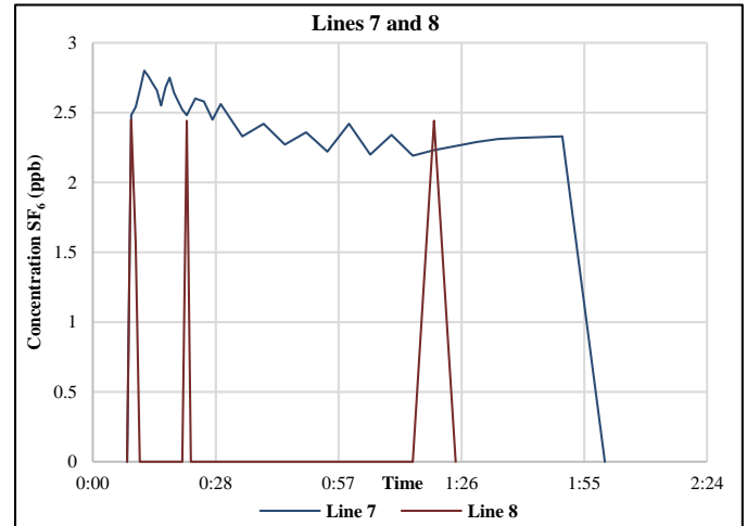
Figure 6. Tracer gas concentrations determined for sampling during face test over test duration, sample lines 7 and 8. The analysis from sample line 8 samples show limited data above the detection limit. More continuous measurements were made on sample line 7, the outby location of tailgate gateroad 1.
