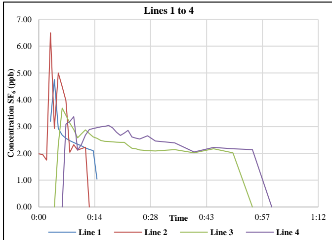
Figure 4. Tracer gas concentrations determined for sampling during face test over test duration, sample lines 1 through 4. First arrival and peak occurred on line 2, prior to arrival and peak on sample line 1.
