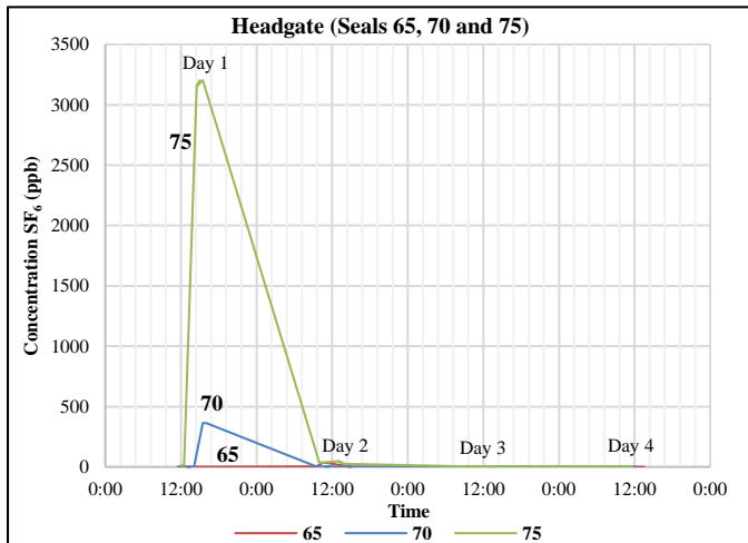
Figure 7. Tracer gas concentrations determined for sampling during gob test from headgate locations nearest to the face.
