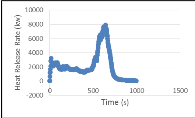
Figure 2. An example of heat release rate curve vs. time.
