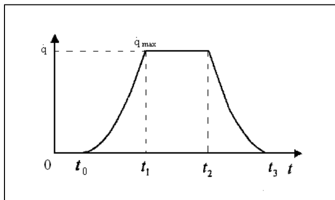
Figure 1. Idealized t-squared fire curve with HRR vs. Time (source: Zhou and Luo, 2010).
